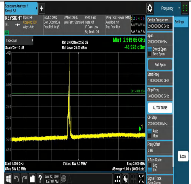
Band2_15MHz_QPSK_18675_1RB#74_1000~3000_1000~3000
