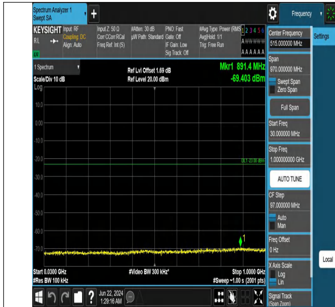
Band2_15MHz_QPSK_18900_1RB#74_30~1000_30~1000
