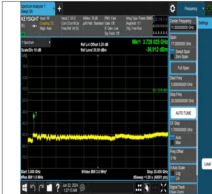
Band2_15MHz_QPSK_18675_1RB#74_3000~20000_3000~2000
