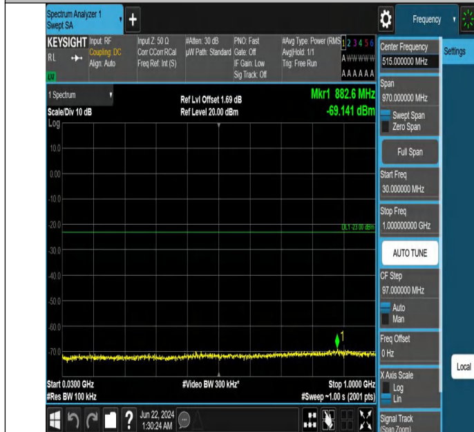
Band2_15MHz_QPSK_19125_1RB#0_30~1000_30~1000
