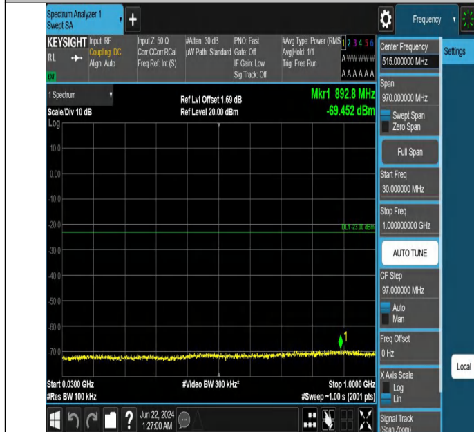
Band2_15MHz_QPSK_18675_1RB#74_30~1000_30~1000
