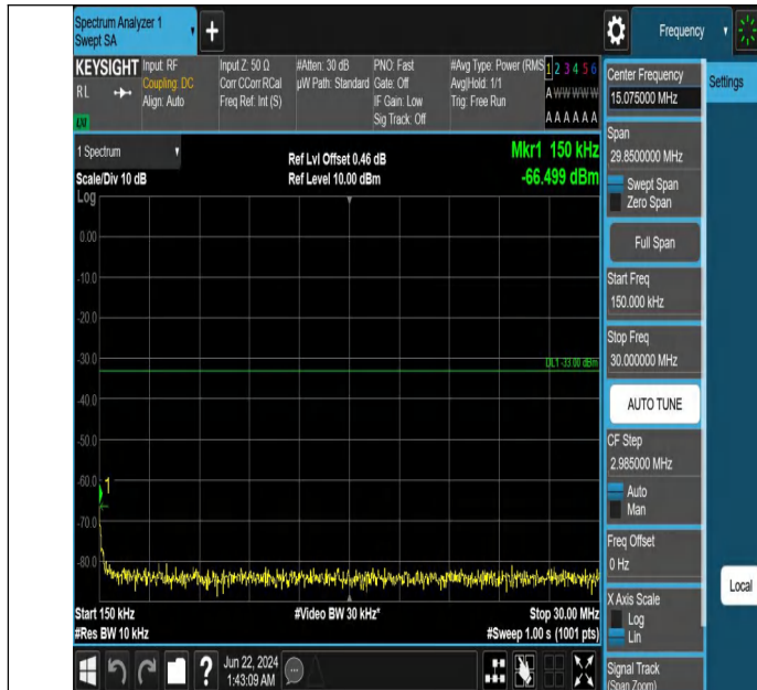
Band2_20MHz_QPSK_18700_1RB#99_0.15~30_0.15~30
