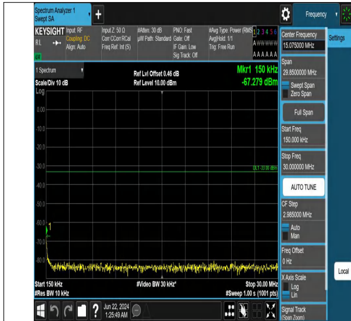
Band2_15MHz_QPSK_18675_1RB#0_0.15~30_0.15~30
