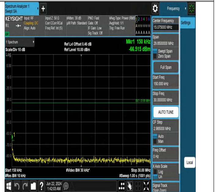
Band2_20MHz_QPSK_18700_1RB#0_0.15~30_0.15~30
