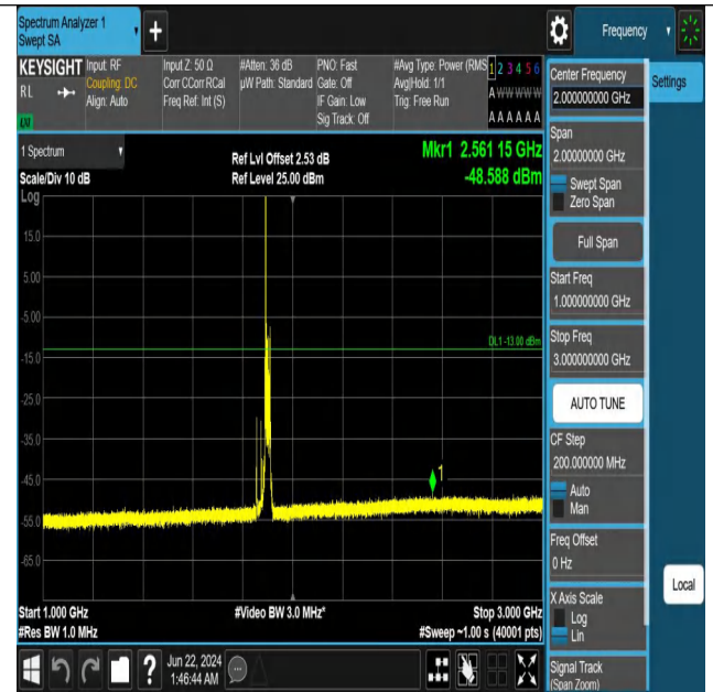
Band2_20MHz_QPSK_19100_1RB#0_1000~3000_1000~3000
