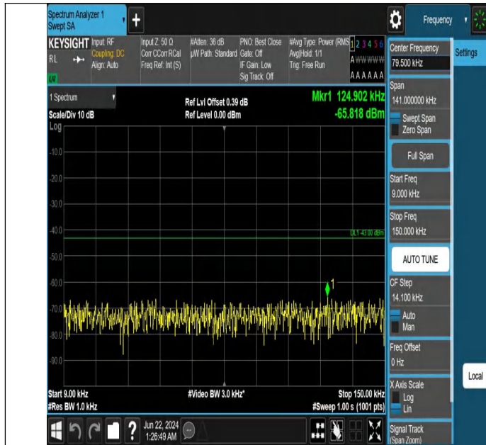
Band2_15MHz_QPSK_18675_1RB#74_0.009~0.15_0.009~0.15
