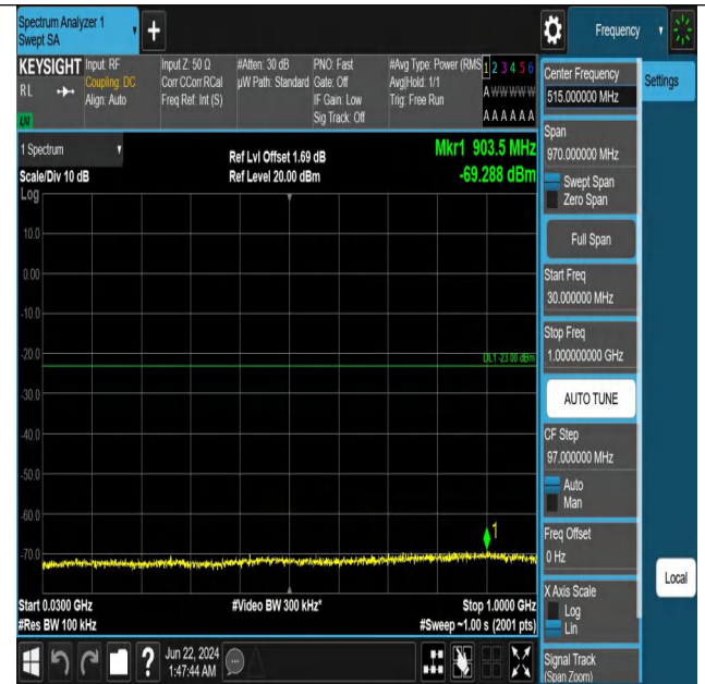
Band2_20MHz_QPSK_19100_1RB#99_30~1000_30~1000
