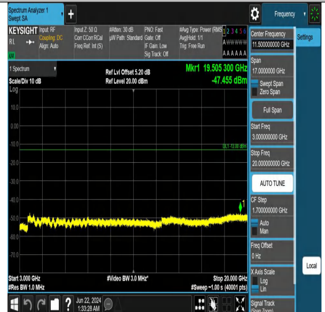
Band2_15MHz_QPSK_18900_75RB#0_3000~20000_3000~2000
