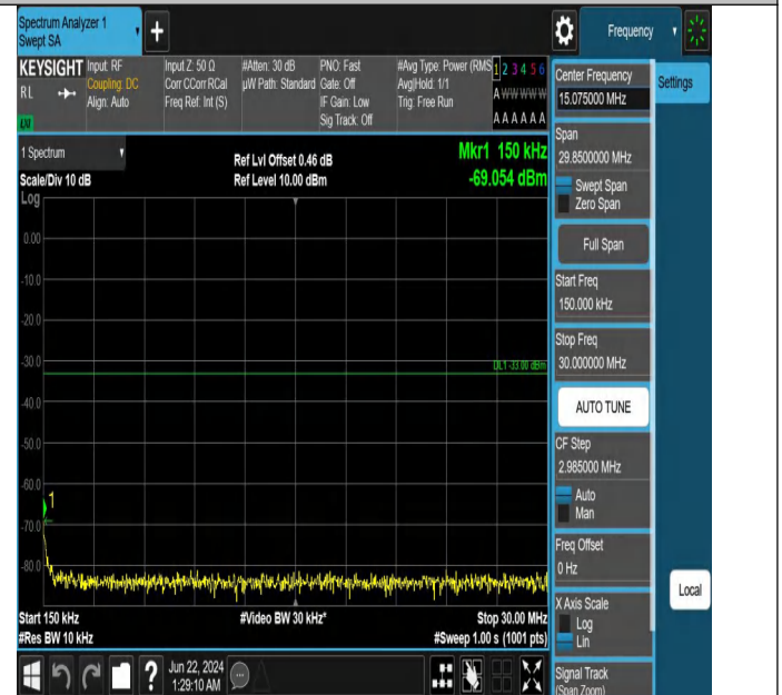
Band2_15MHz_QPSK_18900_1RB#74_0.15~30_0.15~30
