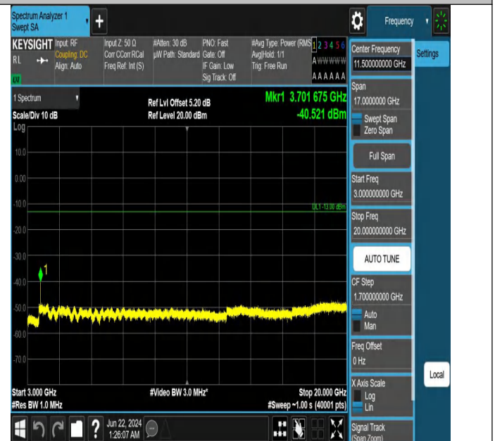
Band2_15MHz_QPSK_18675_1RB#0_3000~20000_3000~20000
