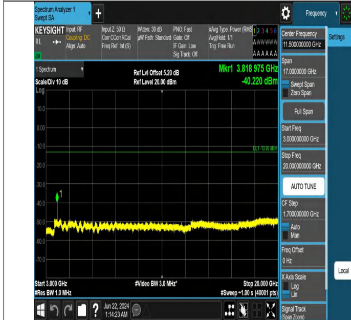
Band2_10MHz_QPSK_19150_1RB#49_3000~20000_3000~2000
