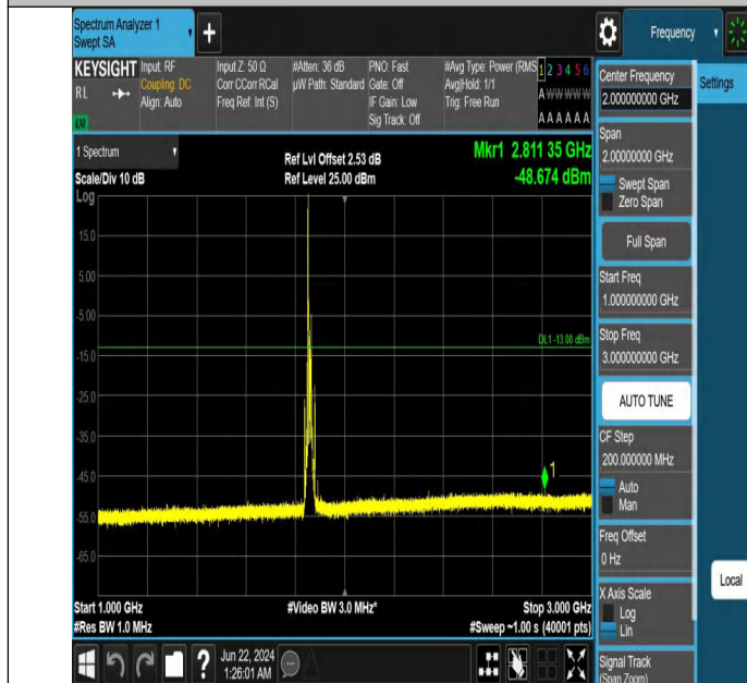
Band2_15MHz_QPSK_18675_1RB#0_1000~3000_1000~3000
