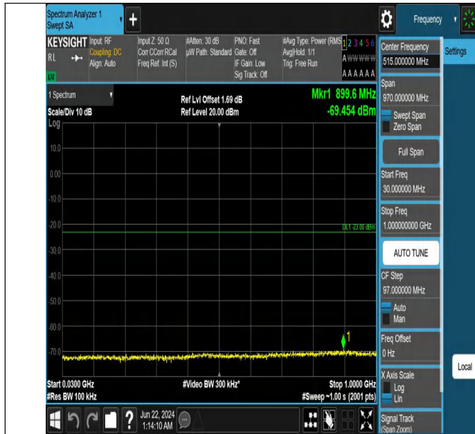
Band2_10MHz_QPSK_19150_1RB#49_30~1000_30~1000
