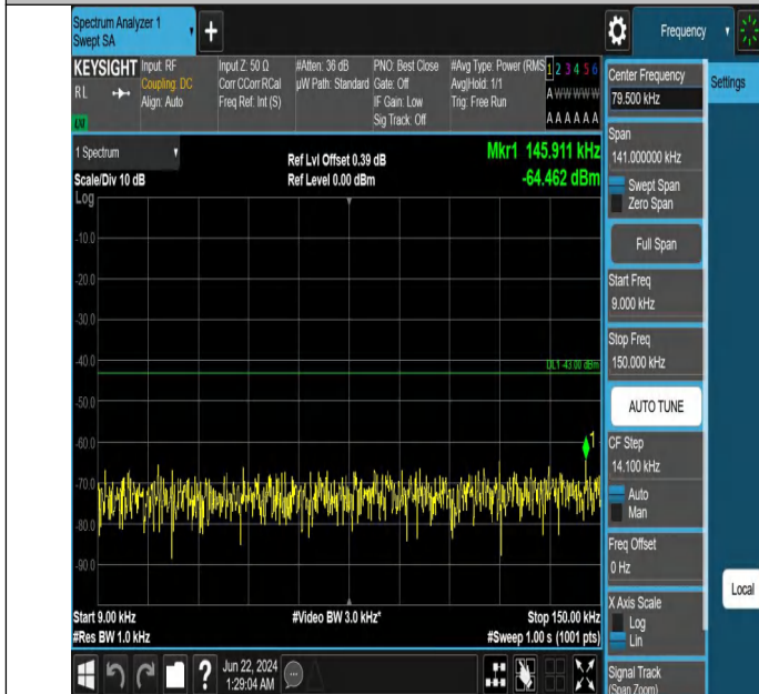
Band2_15MHz_QPSK_18900_1RB#74_0.009~0.15_0.009~0.15
