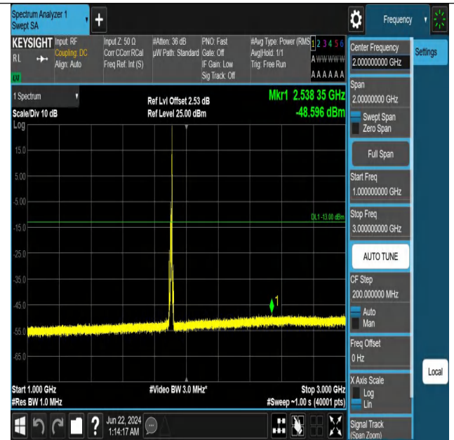
Band2_10MHz_QPSK_19150_1RB#49_1000~3000_1000~3000
