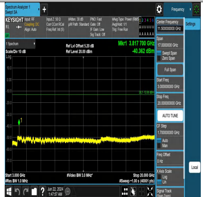
Band2_20MHz_QPSK_19100_1RB#99_3000~20000_3000~2000
