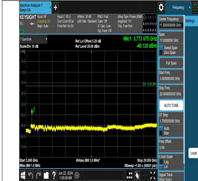
Band2_15MHz_QPSK_18900_1RB#74_3000~20000_3000~2000
