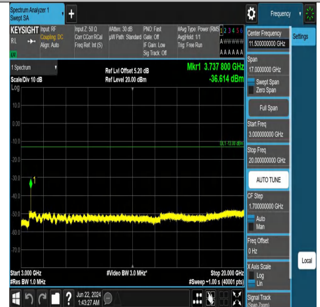
Band2_20MHz_QPSK_18700_1RB#99_3000~20000_3000~2000
