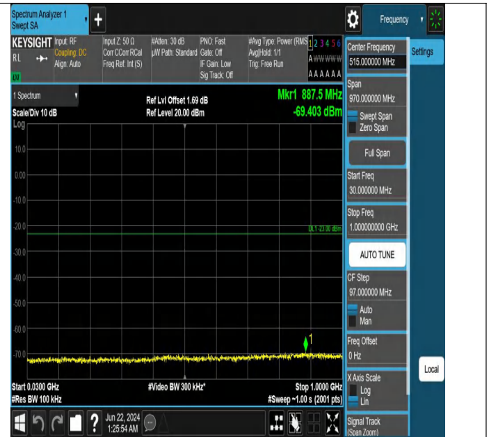
Band2_15MHz_QPSK_18675_1RB#0_30~1000_30~1000
