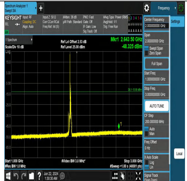
Band2_15MHz_QPSK_19125_1RB#0_1000~3000_1000~3000
