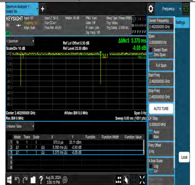
NTNV-11be20MIMO-Ant2-2462
