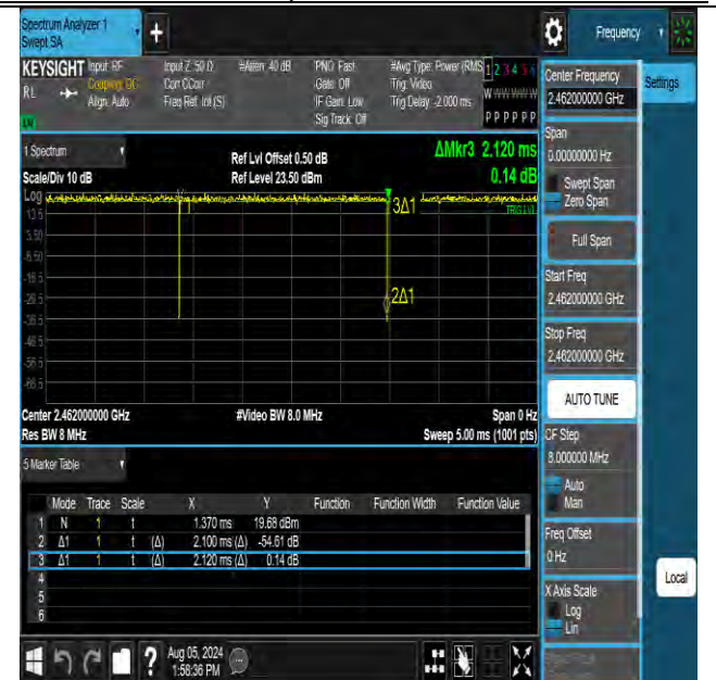
NTNV-11g-CDD-Ant2-2462
