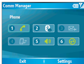
Comm Manager
