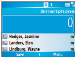
Phone Screen
