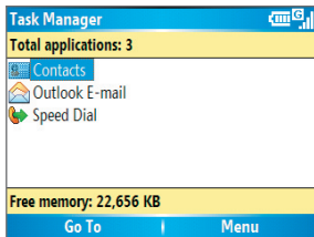
Task Manager
