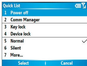
Quick list
