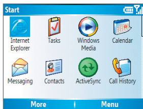
Start menu
