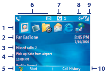
Home Screen
