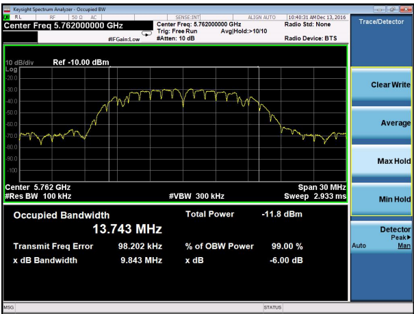
5762MHz-ANT B
