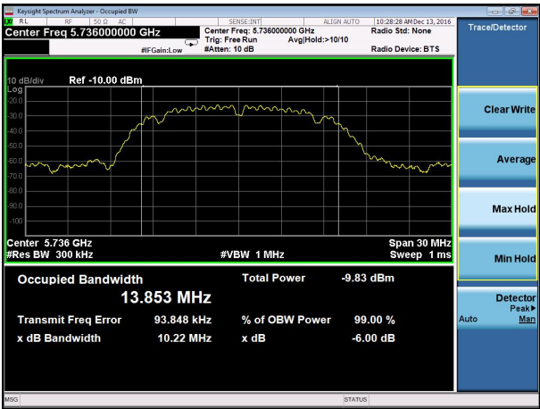
5736MHz-ANT B
