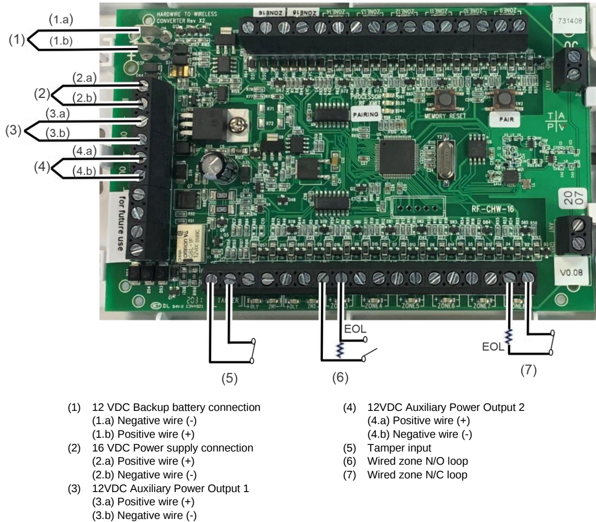
Figure 1: Wiring diagram
