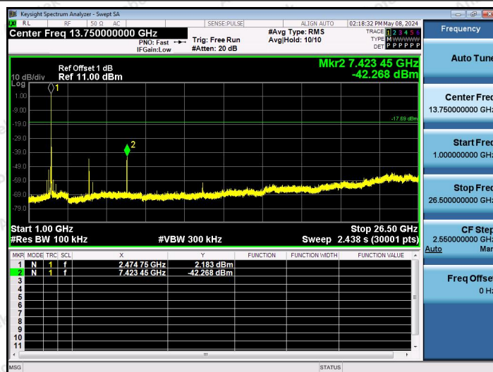
2.4G-Ant1-2474-1000~26500-PASS
