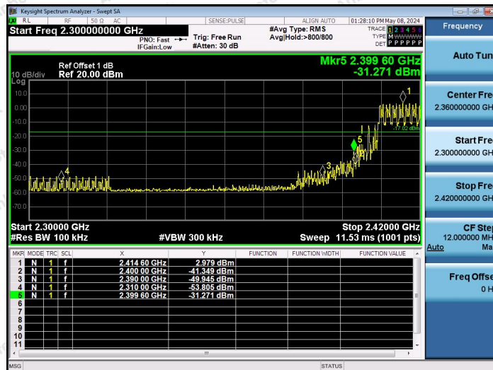
2.4G-Ant1-Hop_2408-PASS
