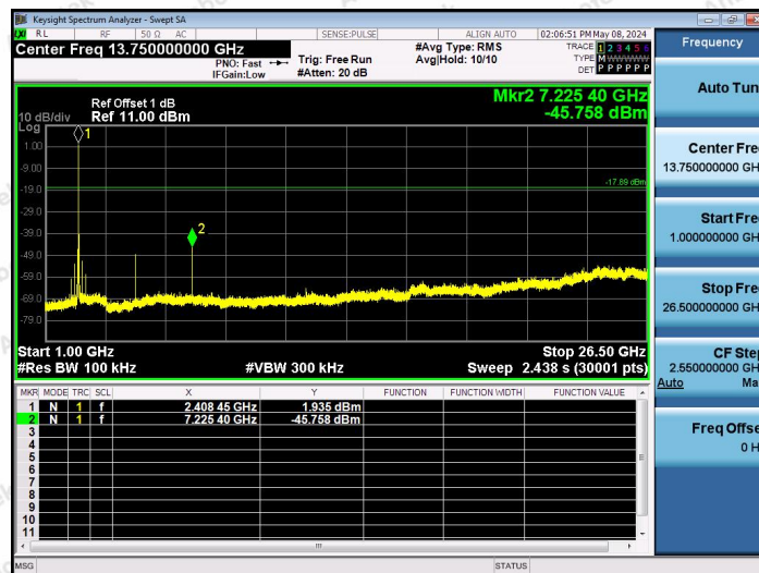
2.4G-Ant1-2408-1000~26500-PASS
