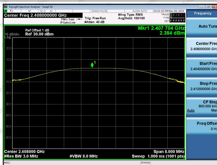
2.4G-Ant1-2408-PASS
