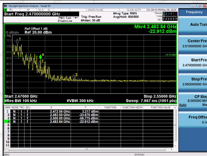
2.4G-Ant1-Hop_2474-PASS
