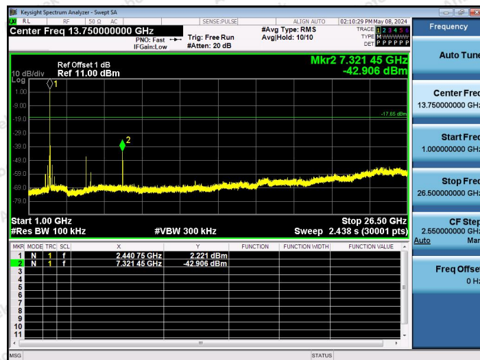
2.4G-Ant1-2440-1000~26500-PASS
