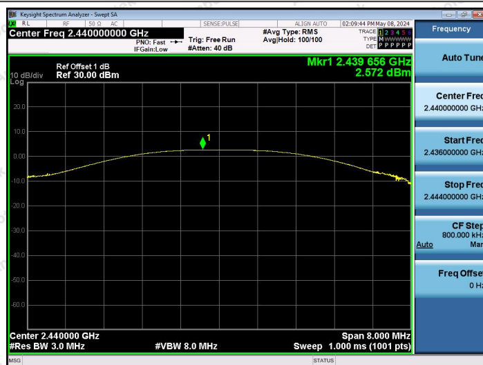
2.4G-Ant1-2440-PASS
