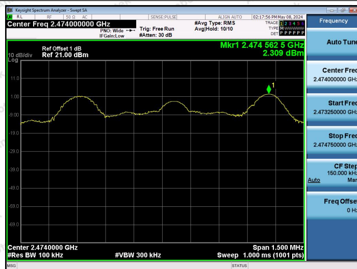
2.4G-Ant1-2474-0~Reference-PASS
