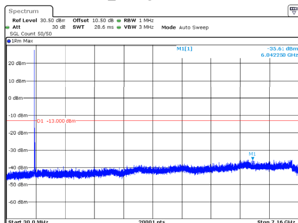
n12_15MHz_15kHz_707.5MHz_DFT-s-OFDM QPSK_RB1@0 -35.61dBm
