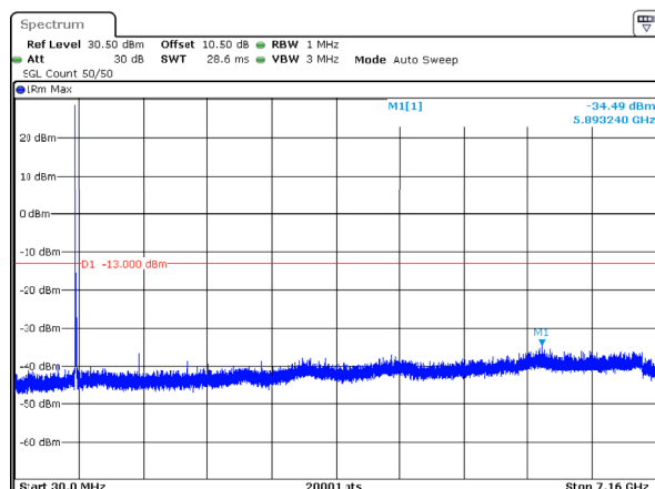
n12_15MHz_15kHz_706.5MHz_DFT-s-OFDM QPSK_RB1@0 -34.49dBm
