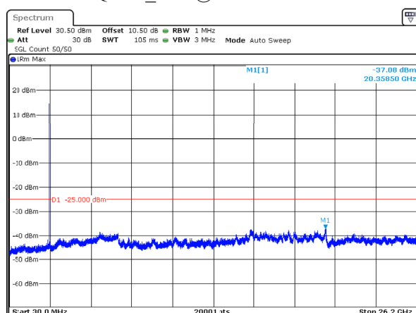
n38_5MHz_15kHz_2572.5MHz_DFT-s-OFDM QPSK_RB1@24 -37.08dBm
