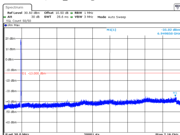
n12_15MHz_15kHz_708.5MHz_DFT-s-OFDM QPSK_RB75@0 -35.02dBm
