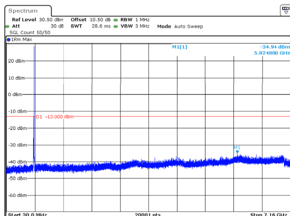
n12_15MHz_15kHz_706.5MHz_DFT-s-OFDM QPSK_RB1@78 -34.94dBm
