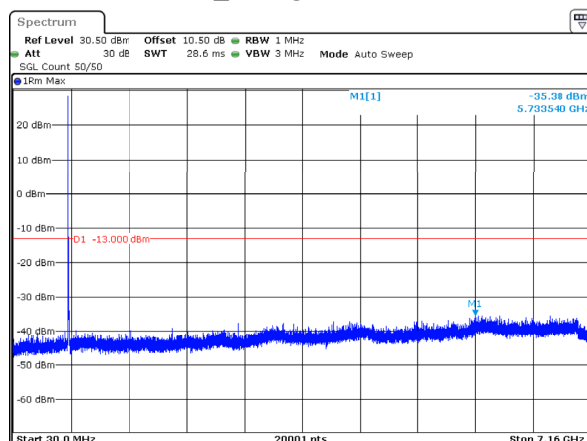
n12_10MHz_15kHz_704MHz_DFT-s-OFDM QPSK_RB1@0 -35.38dBm
