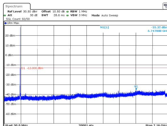
n12_15MHz_15kHz_708.5MHz_DFT-s-OFDM QPSK_RB1@78 -35.32dBm
