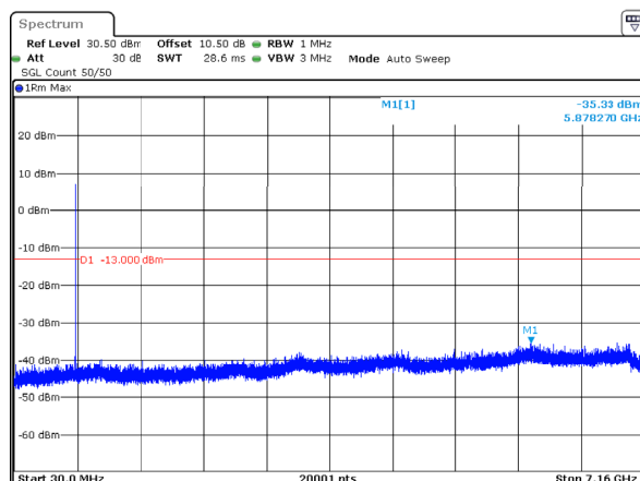
n12_5MHz_15kHz_713.5MHz_DFT-s-OFDM QPSK_RB1@24 -35.33dBm
