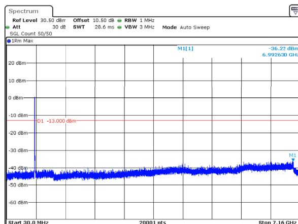
n12_10MHz_15kHz_704MHz_DFT-s-OFDM QPSK_RB50@0 -36.22dBm
