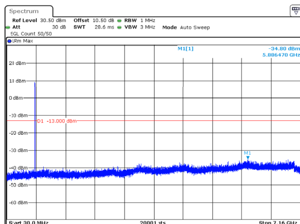
n12_5MHz_15kHz_713.5MHz_DFT-s-OFDM QPSK_RB1@0 -34.80dBm
