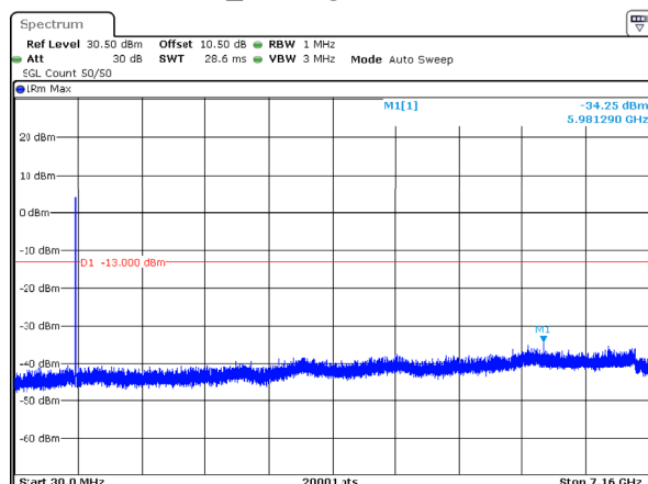
n12_5MHz_15kHz_713.5MHz_DFT-s-OFDM QPSK_RB25@0 -34.25dBm
