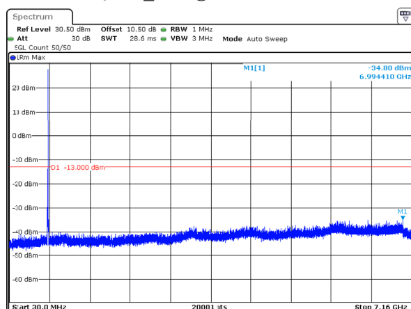
n12_15MHz_15kHz_707.5MHz_DFT-s-OFDM QPSK_RB1@78 -34.80dBm
