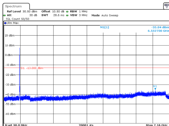
n12_10MHz_15kHz_704MHz_DFT-s-OFDM QPSK_RB1@51 -35.04dBm
