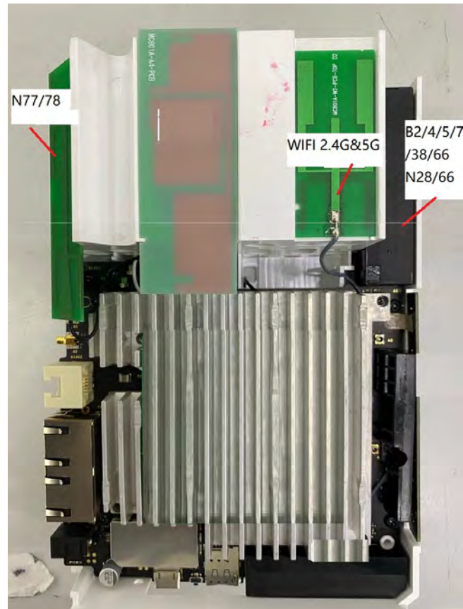
Antenna location
