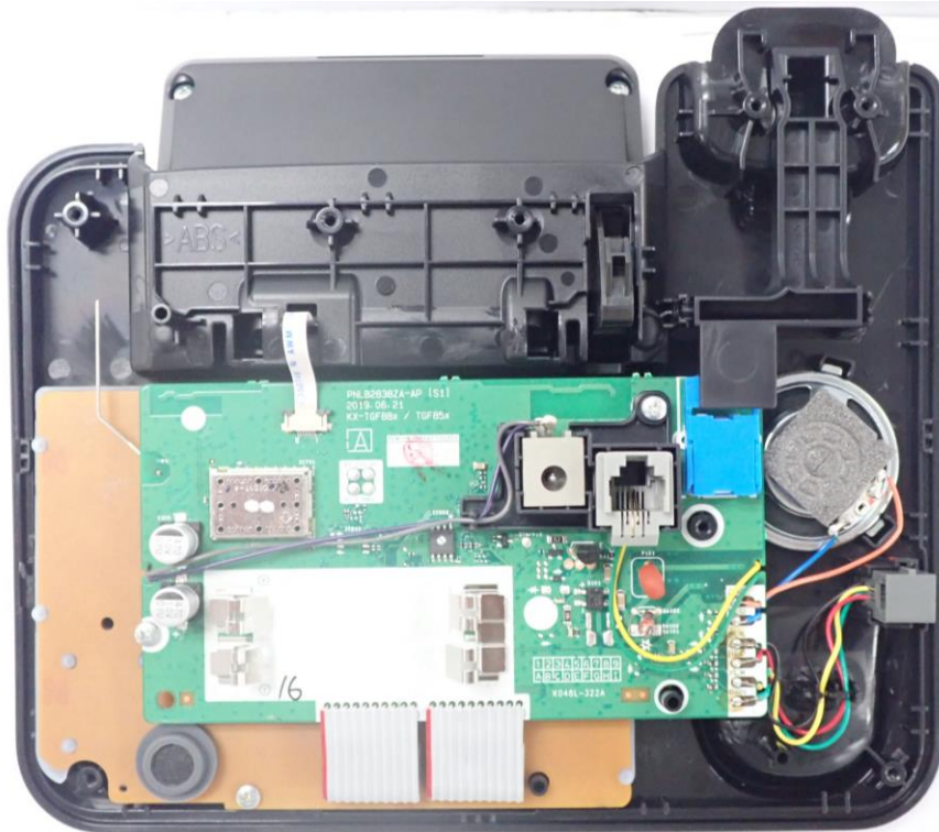
Main Board (Back side)
