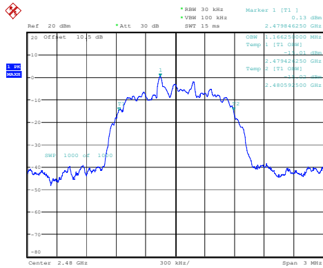
2DH1_High 1.166MHz
