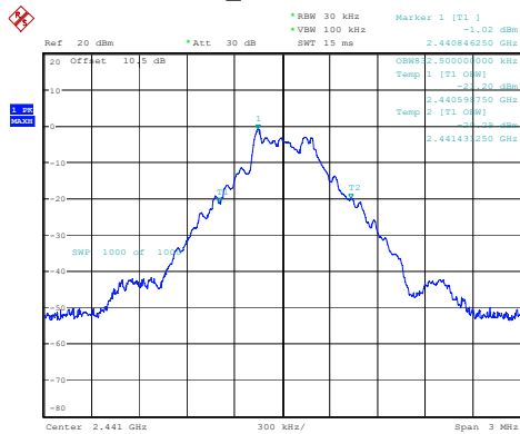
DH1_Middle 0.833MHz
