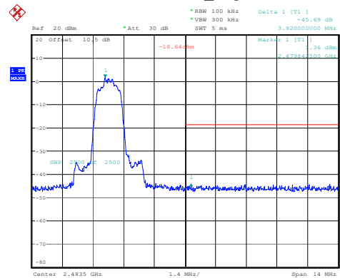
2DH1_High
