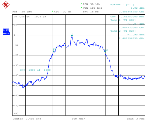
2DH1_Low 1.166MHz
