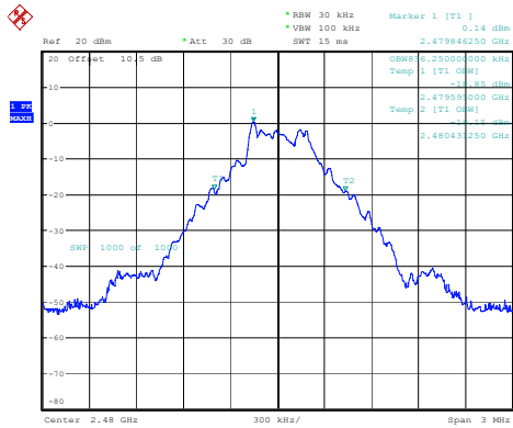
DH1_High 0.836MHz
