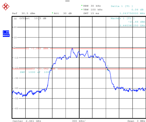
2DH1_Middle 1.264MHz
