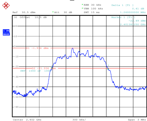
2DH1_Low 1.260MHz
