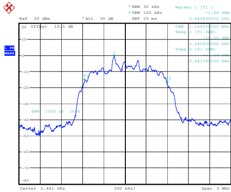
2DH1_Middle 1.166MHz
