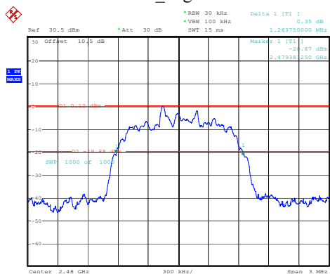
2DH1_High 1.264MHz
