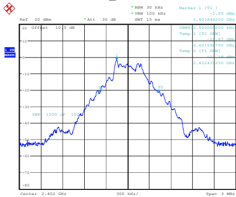
DH1_Low 0.833MHz
