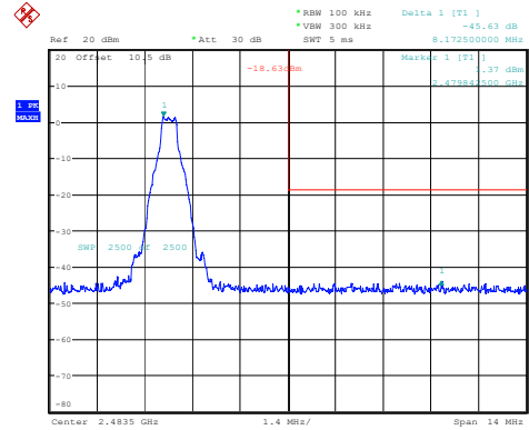
DH1_High
