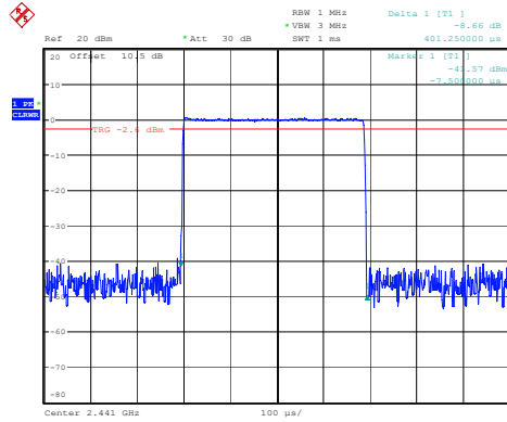
DH1_Hopping 0.401ms
