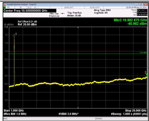
66-66-20MHz-20MHz-64QAM-64QAM-132072-132270-100RB#0-100RB#0-1000~20000MHz-PASS
