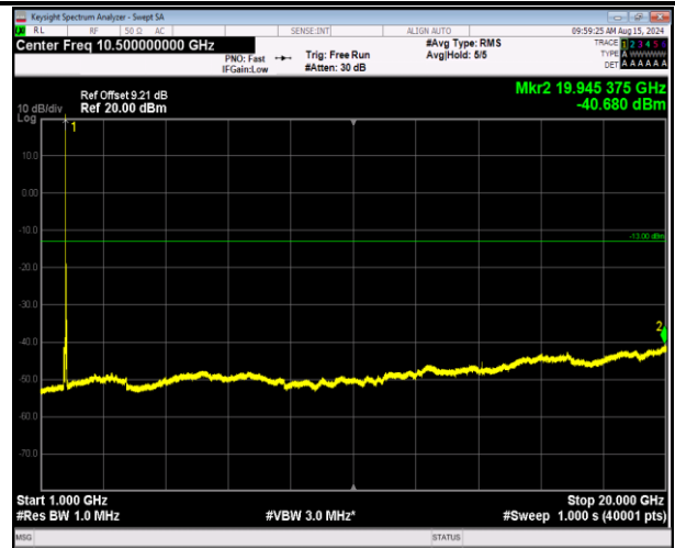
66-66-20MHz-5MHz-16QAM-16QAM-132522-132639-1RB# 0-0RB#0-1000~20000MHz-PASS
