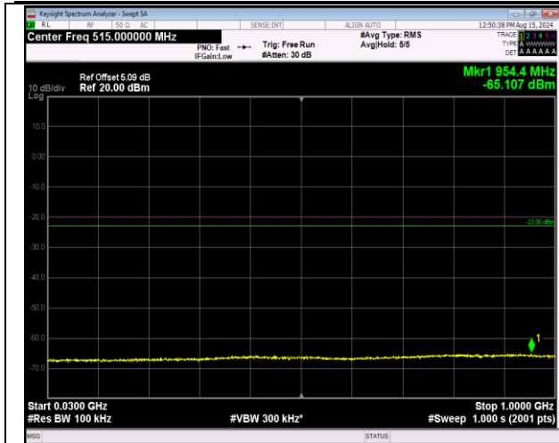
66-66-20MHz-20MHz-16QAM-16QAM-132072-132270-1 00RB#0-100RB#0-30~1000MHz-PASS
