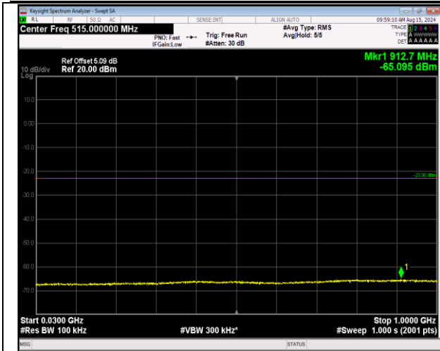
66-66-20MHz-5MHz-16QAM-16QAM-132522-132639-1R B#0-0RB#0-30~1000MHz-PASS
