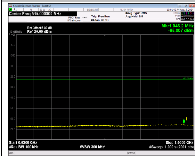
66-66-20MHz-5MHz-16QAM-16QAM-132522-132639-1R B#0-1RB#24-30~1000MHz-PASS
