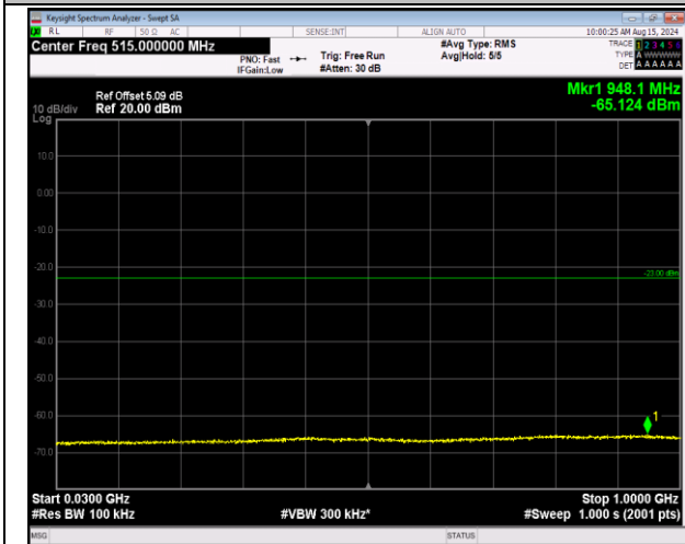
66-66-20MHz-5MHz-16QAM-16QAM-132522-132639-1R B#99-0RB#0-30~1000MHz-PASS
