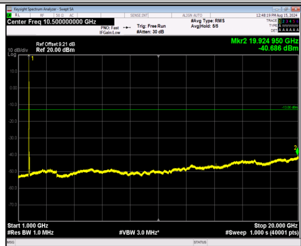
66-66-20MHz-20MHz-16QAM-16QAM-132072-132270-1RB #99-ORB#0-1000~20000MHz-PASS
