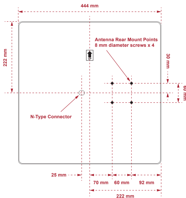
Mounting Diagram
