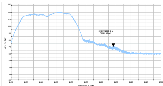
802.11g-Channel 11 Peak
