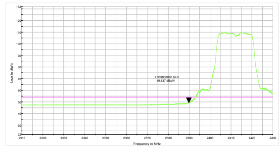
802.11g-Channel 1 Average
