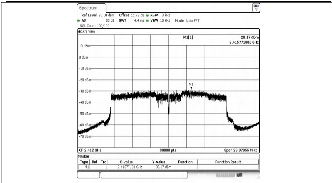
11AX20SISO-Ant1-2412-PASS
