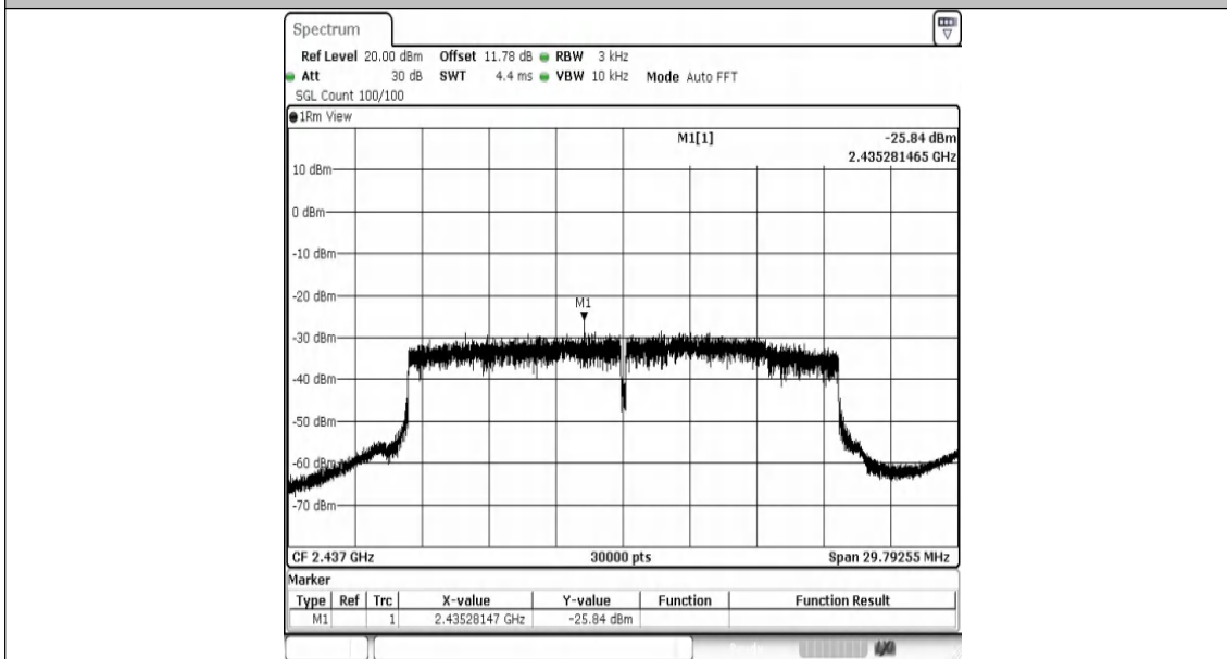
11AX20SISO-Ant1-2437-PASS
