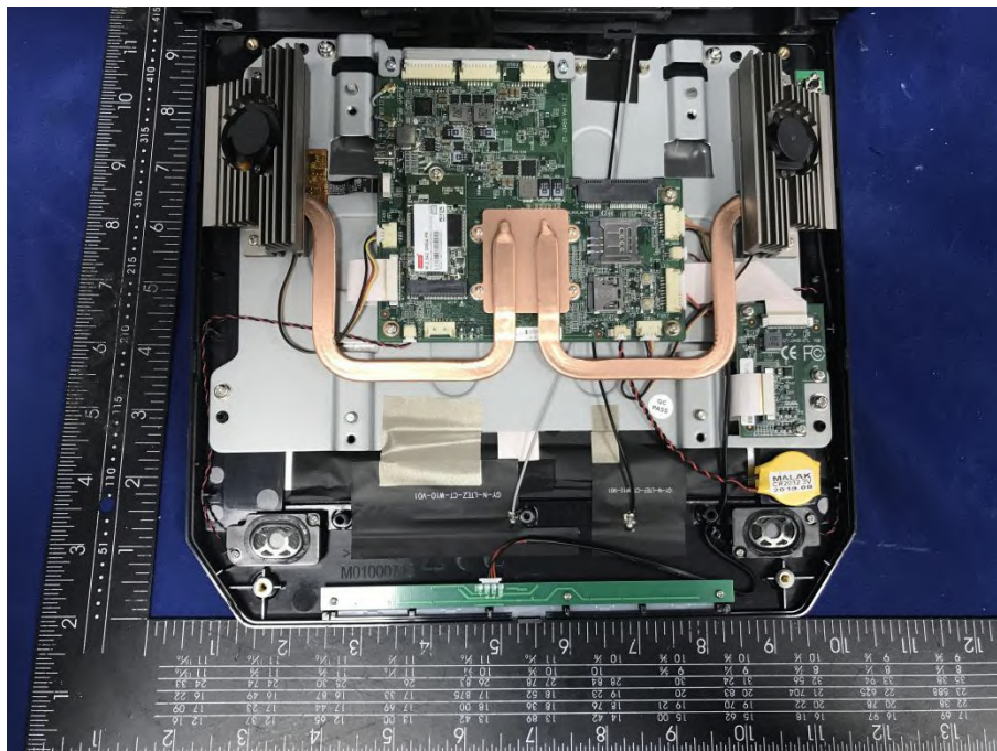
J3455 PCB
