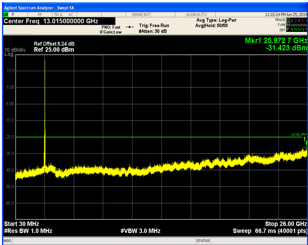
LTE Band41 QPSK BW=10MHz Channel=41190 RB Size=50 Position=#0
