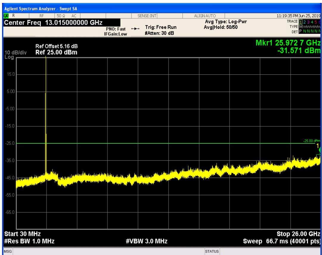
LTE Band41 QAM16 BW=10MHz Channel=40090 RB Size=1 Position=#0
