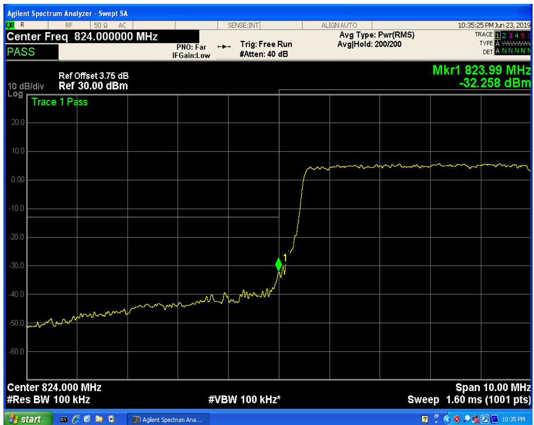
LTE Band5 QAM16 BW=10MHz Channel=20450 RB Size=25 Position=#Max
