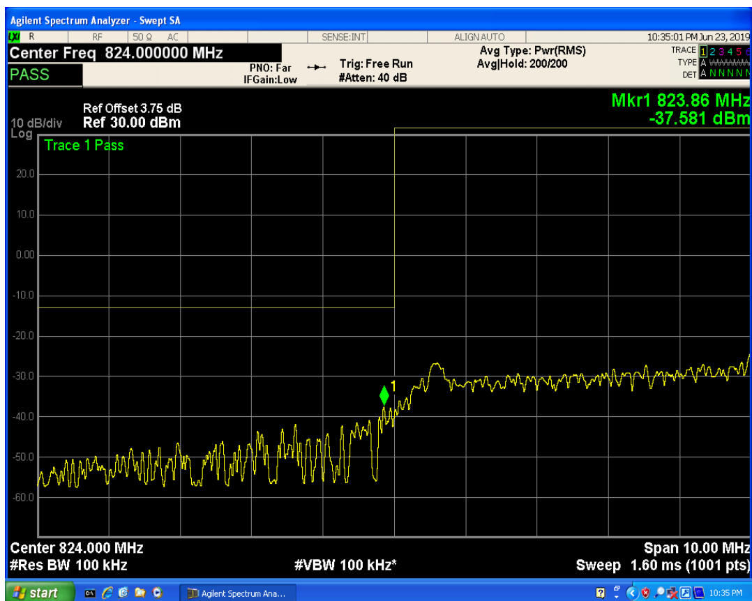
LTE Band5 QPSK BW=10MHz Channel=20450 RB Size=25 Position=#0
