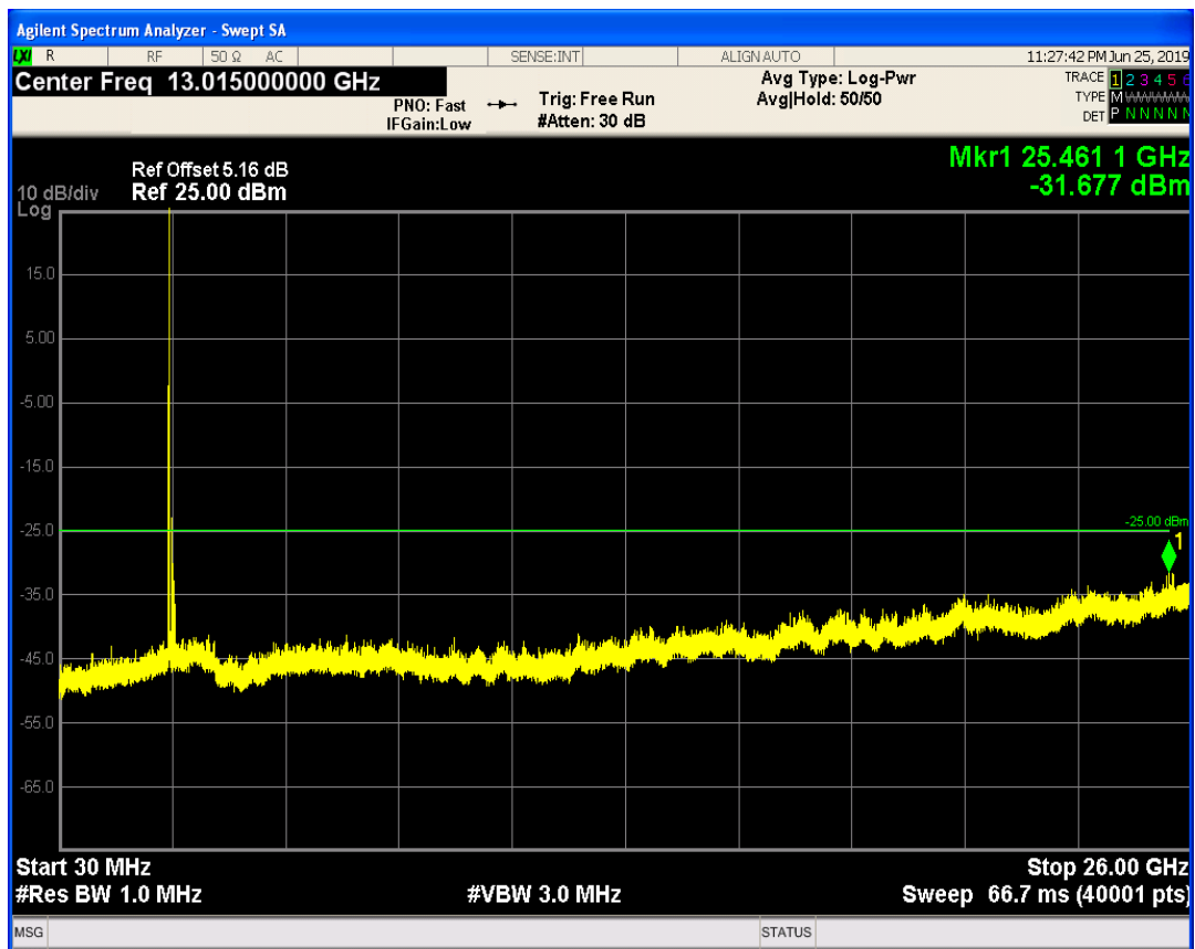
LTE Band41 QAM16 BW=15MHz Channel=40115 RB Size=1 Position=#0
