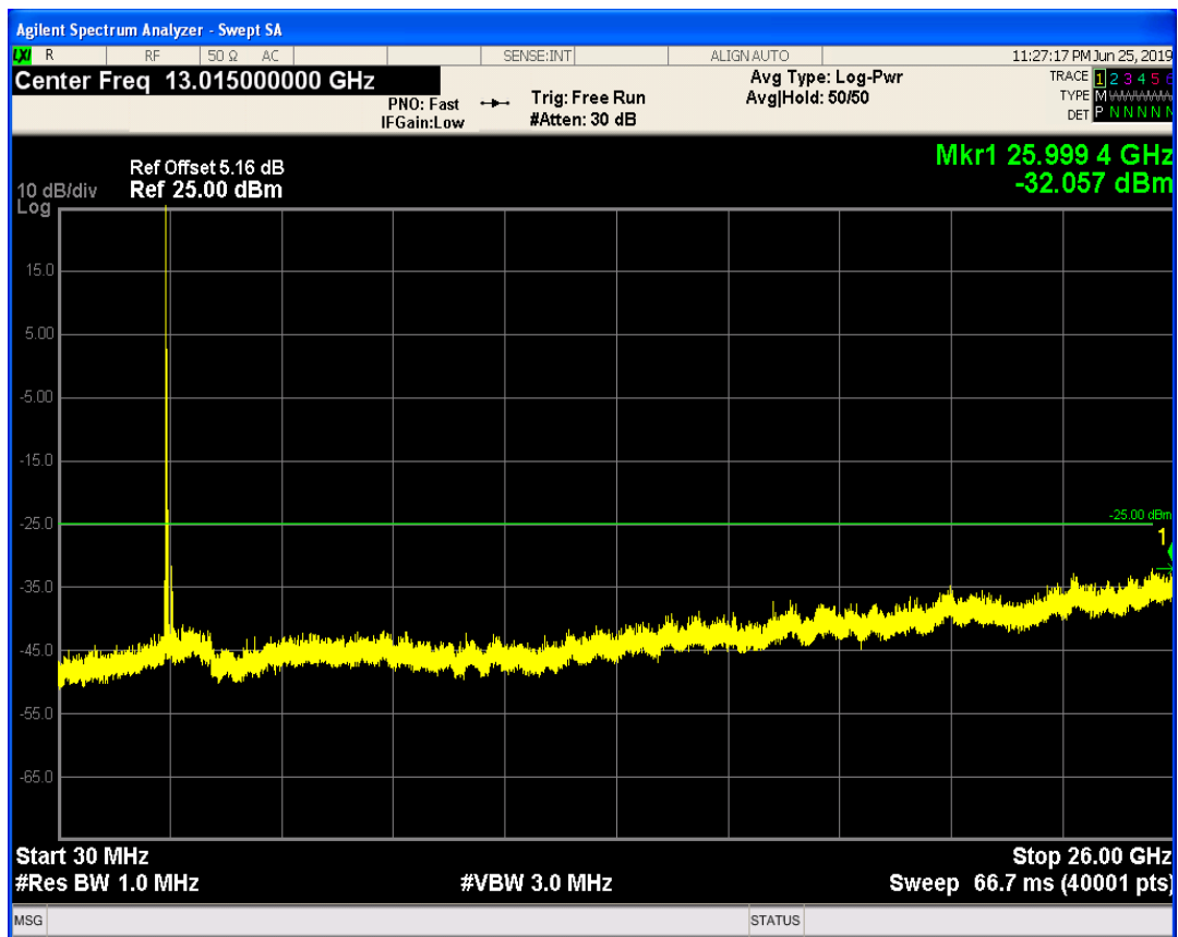
LTE Band41 QAM16 BW=10MHz Channel=41190 RB Size=1 Position=#Max
