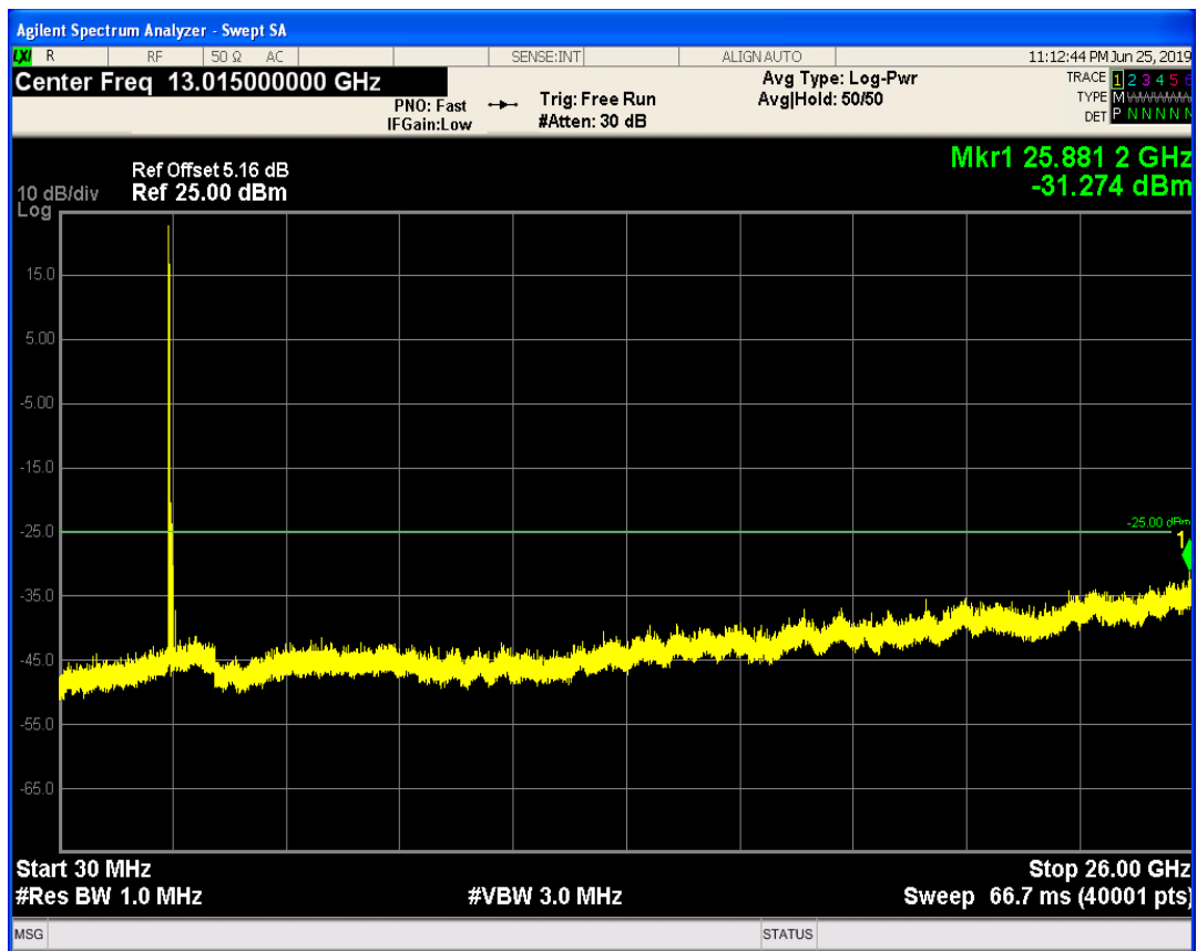
LTE Band41 QAM16 BW=5MHz Channel=41215 RB Size=12 Position=#0
