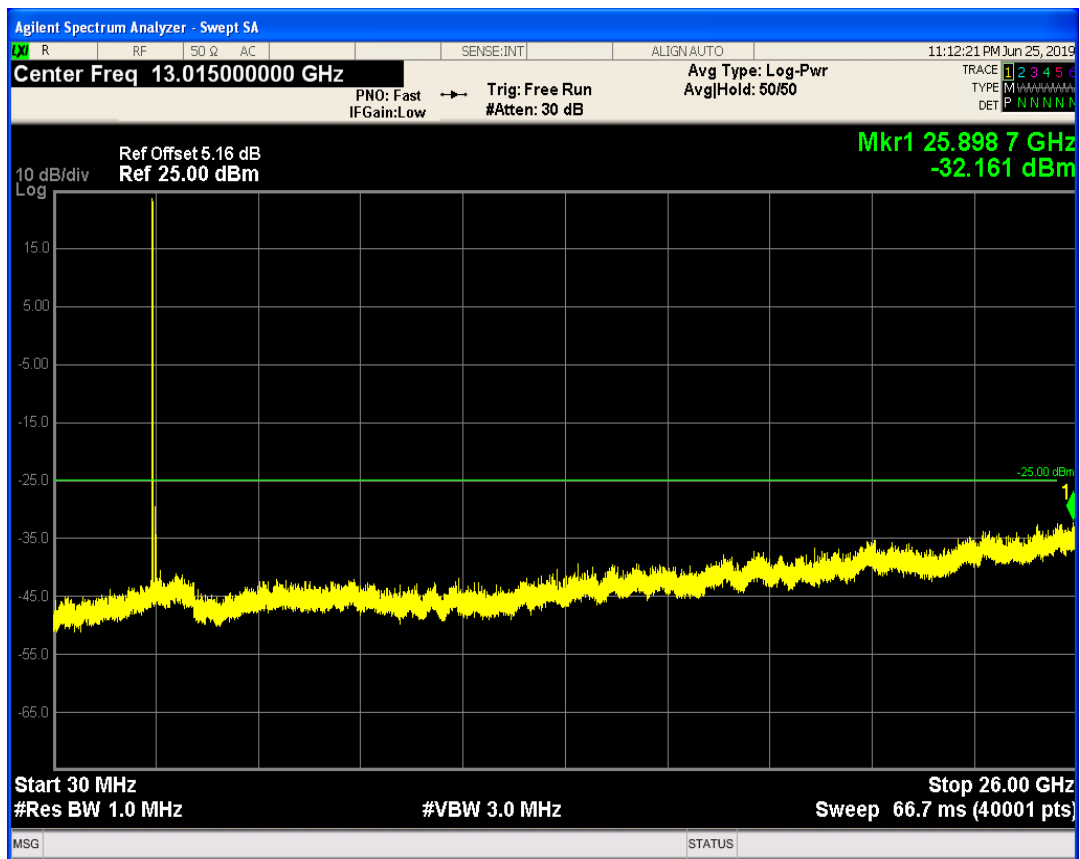
LTE Band41 QAM16 BW=5MHz Channel=40065 RB Size=25 Position=#0
