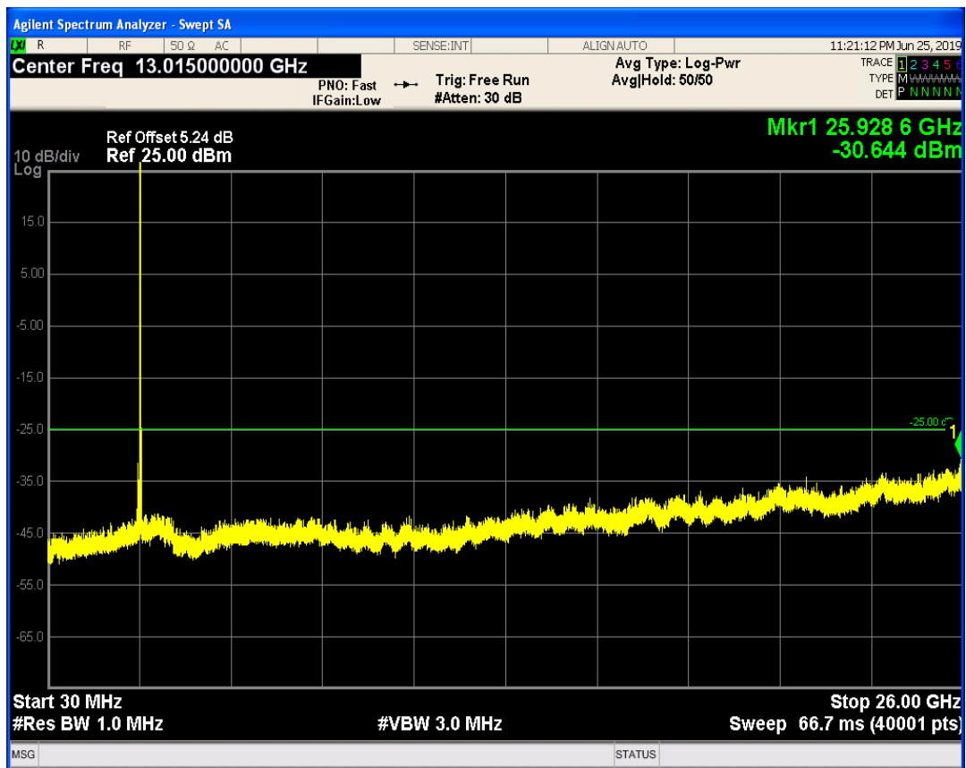
LTE Band41 QPSK BW=10MHz Channel=41190 RB Size=1 Position=#Max
