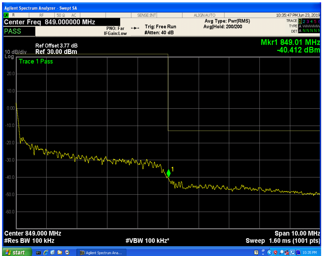
LTE Band5 QPSK BW=10MHz Channel=20600 RB Size=25 Position=#Max
