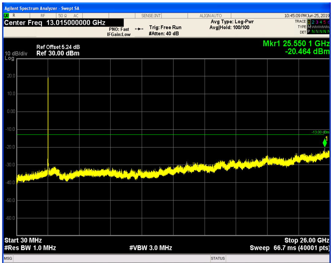
LTE Band41 QPSK BW=5MHz Channel=41215 RB Size=25 Position=#0
