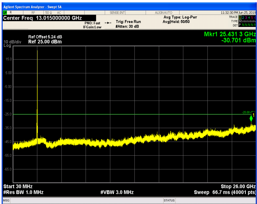
LTE Band41 QAM16 BW=15MHz Channel=41165 RB Size=75 Position=#0
