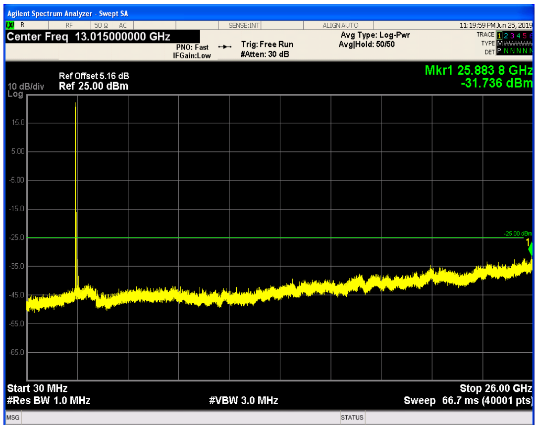
LTE Band41 QAM16 BW=10MHz Channel=40090 RB Size=1 Position=#Max
