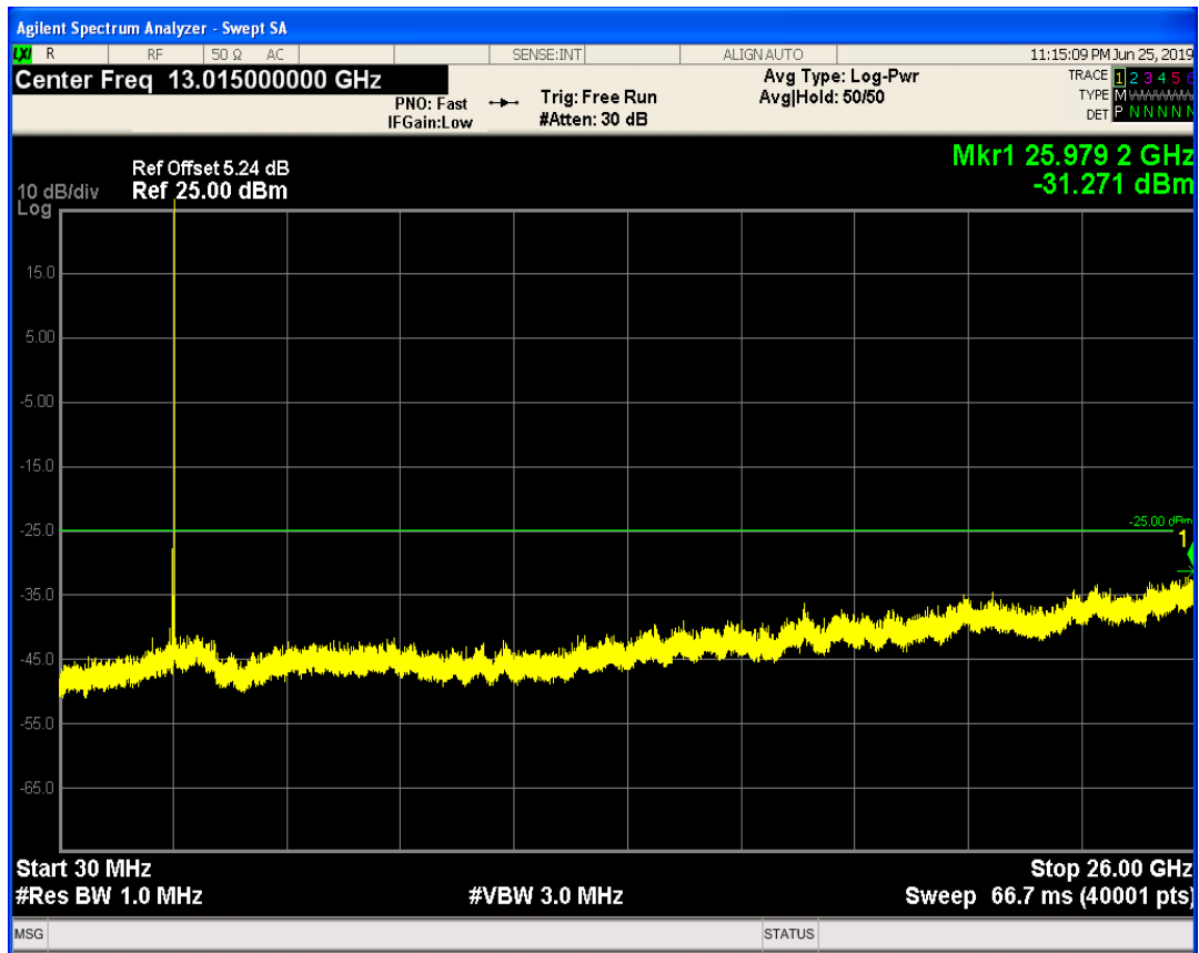
LTE Band41 QAM16 BW=5MHz Channel=41215 RB Size=1 Position=#Max
