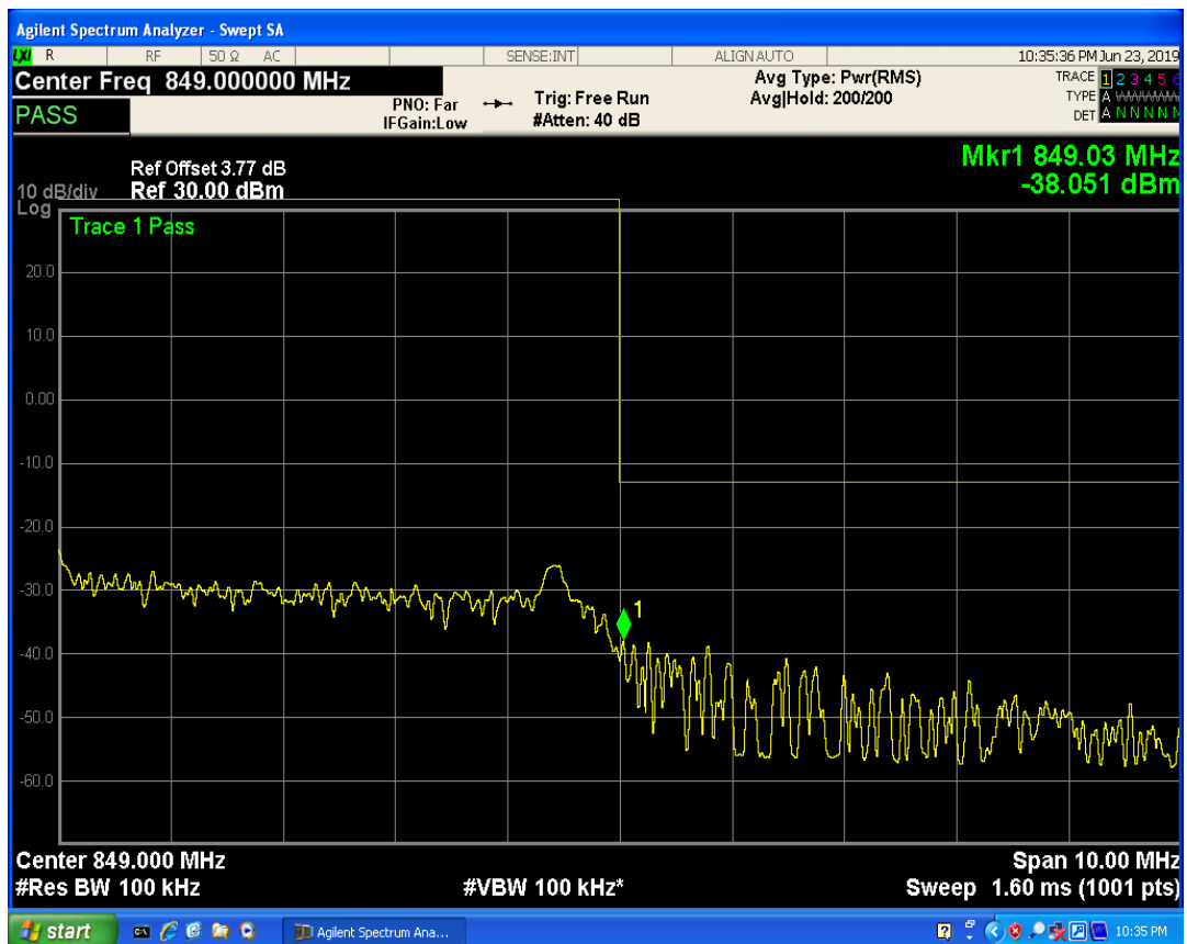
LTE Band5 QPSK BW=10MHz Channel=20600 RB Size=1 Position=#Mid
