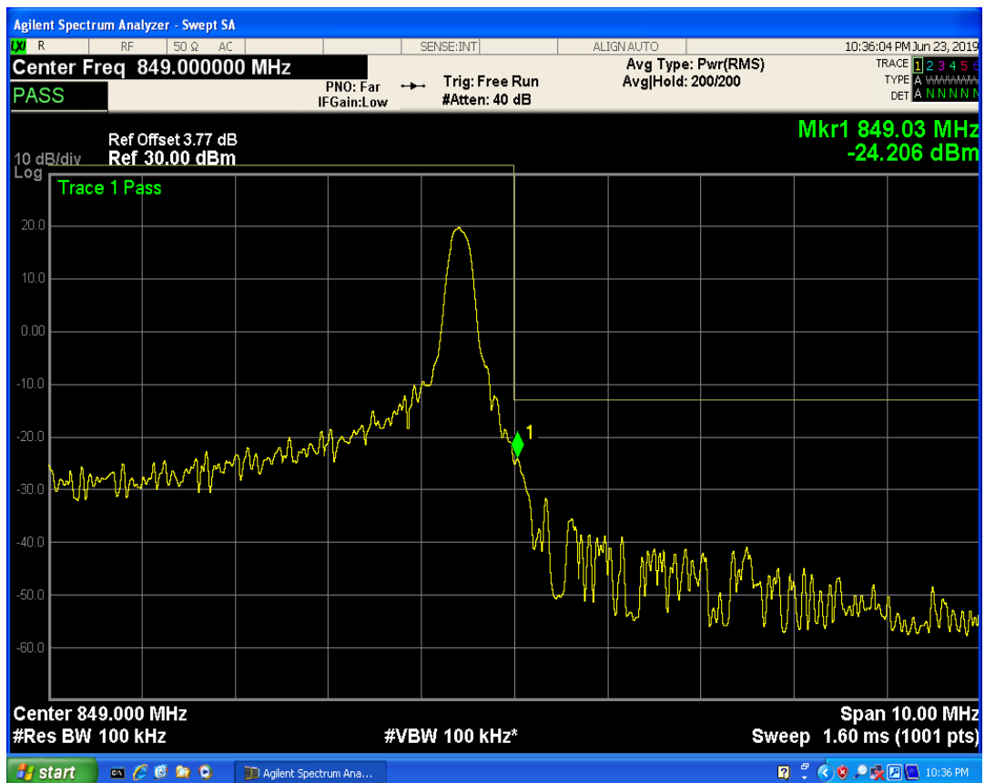
LTE Band5 QAM16 BW=10MHz Channel=20600 RB Size=25 Position=#Max
