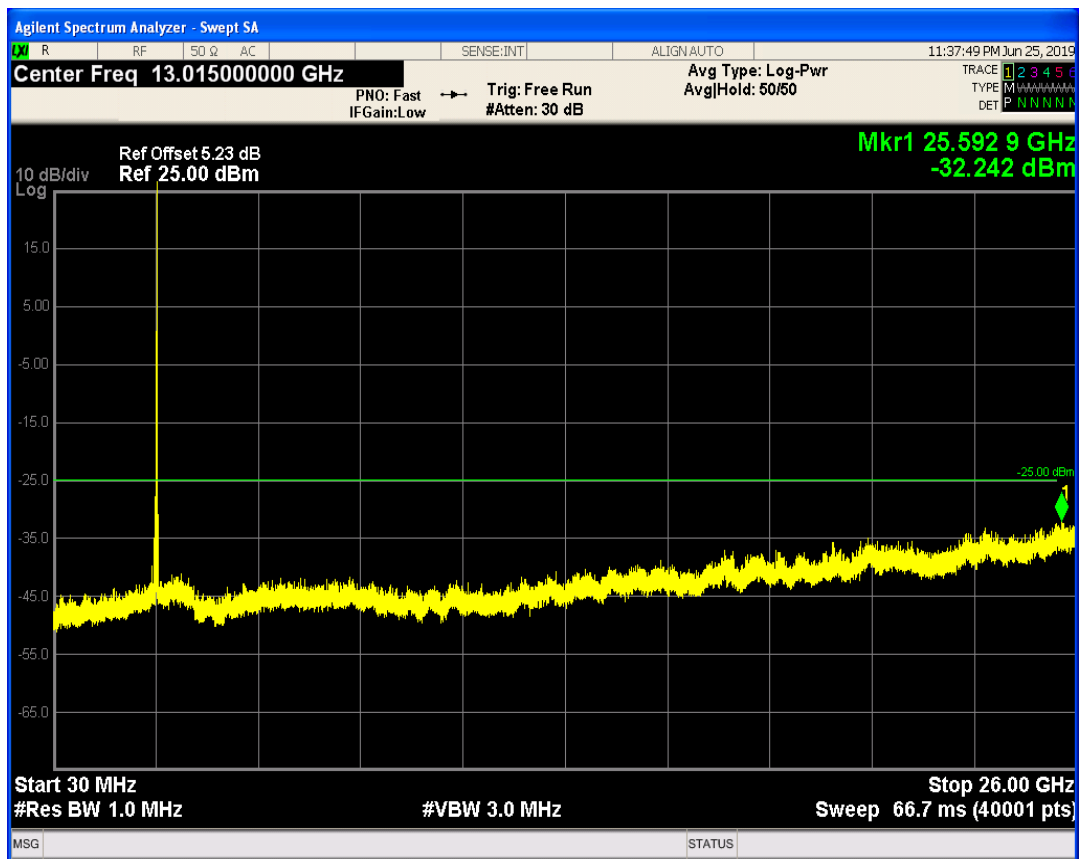
LTE Band41 QPSK BW=20MHz Channel=40140 RB Size=50 Position=#Max
