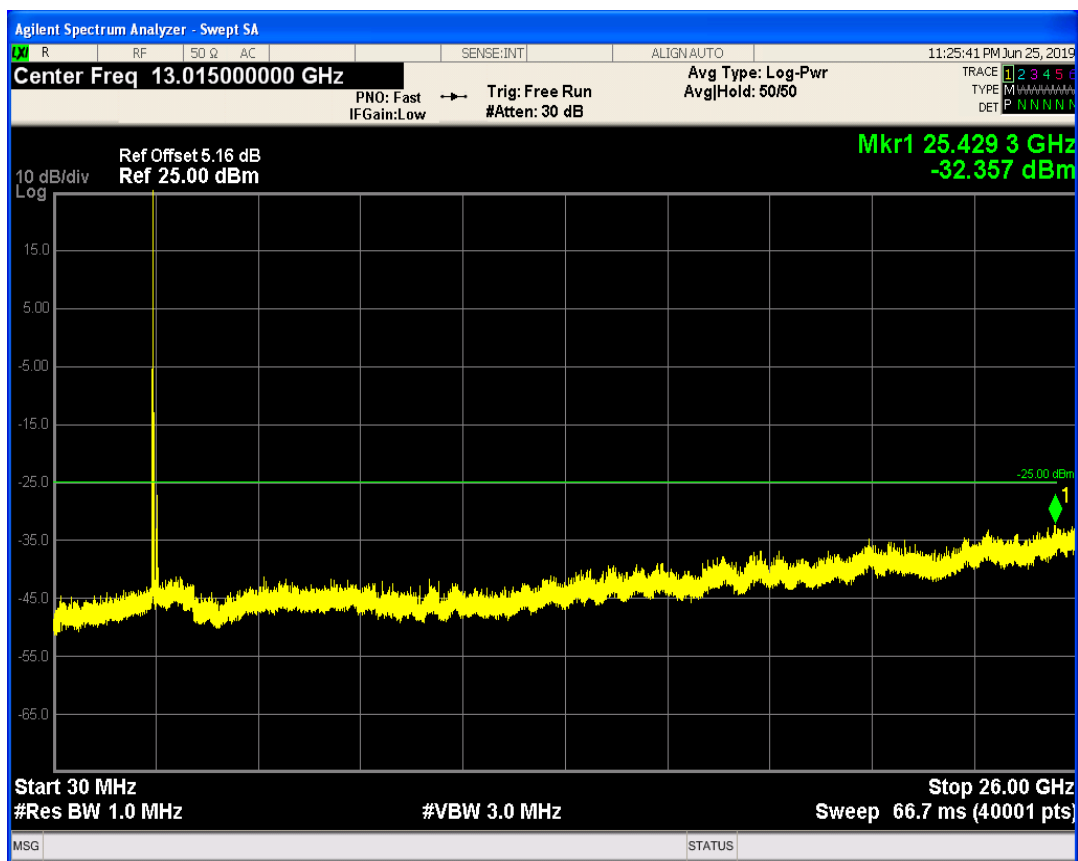
LTE Band41 QPSK BW=10MHz Channel=41190 RB Size=25 Position=#Max
