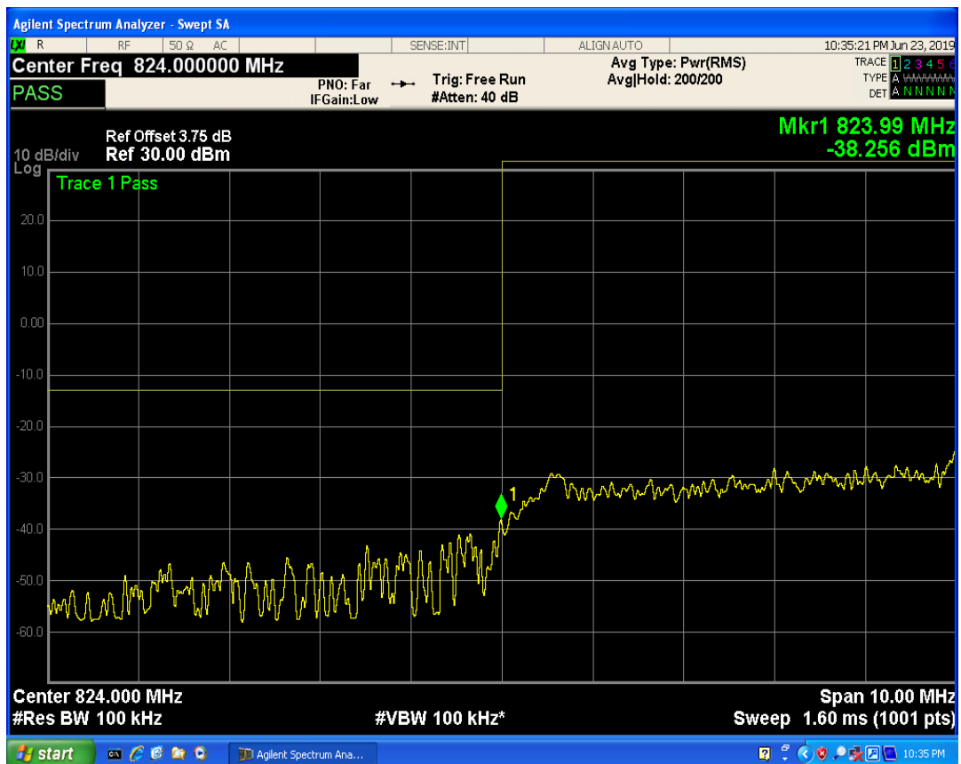
LTE Band5 QAM16 BW=10MHz Channel=20450 RB Size=25 Position=#0
