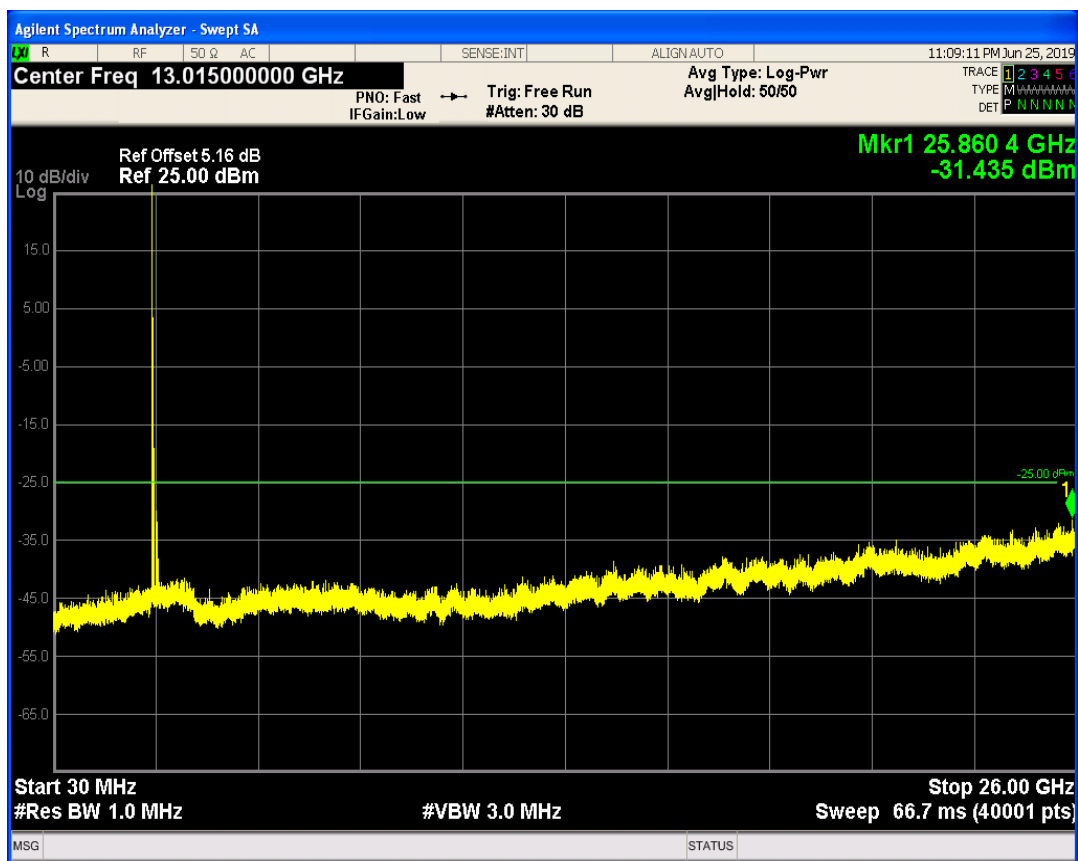
LTE Band41 QPSK BW=5MHz Channel=40065 RB Size=1 Position=#Max
