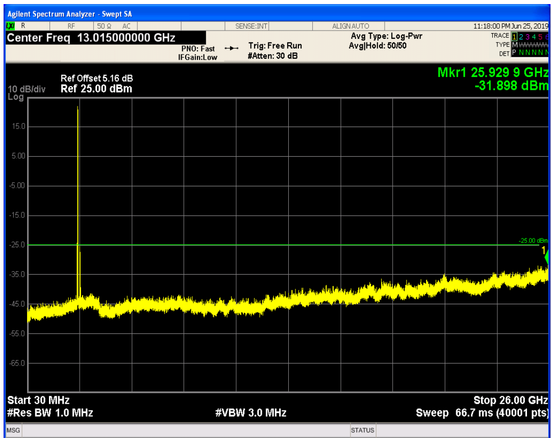
LTE Band41 QAM16 BW=5MHz Channel=41215 RB Size=1 Position=#0
