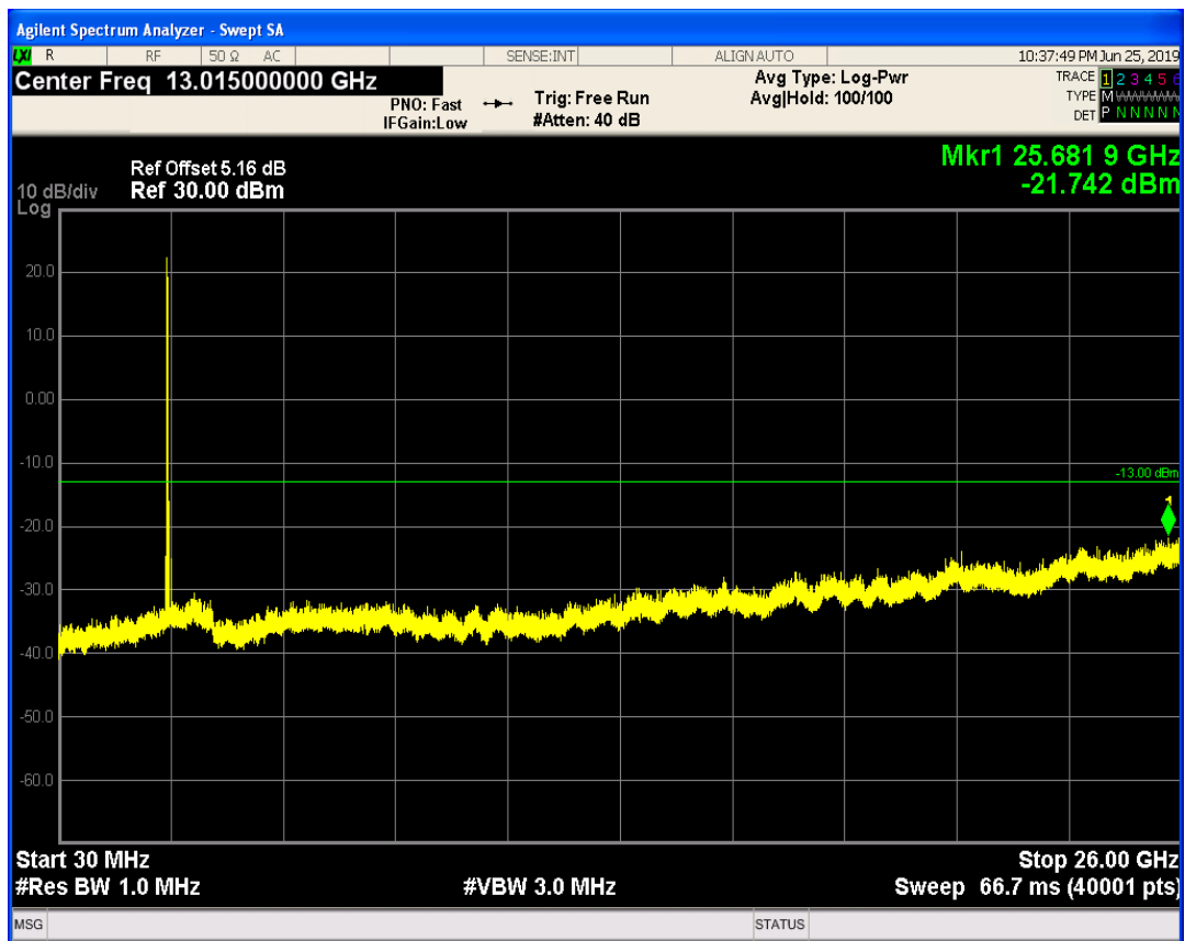
LTE Band41 QAM16 BW=15MHz Channel=40115 RB Size=75 Position=#0
