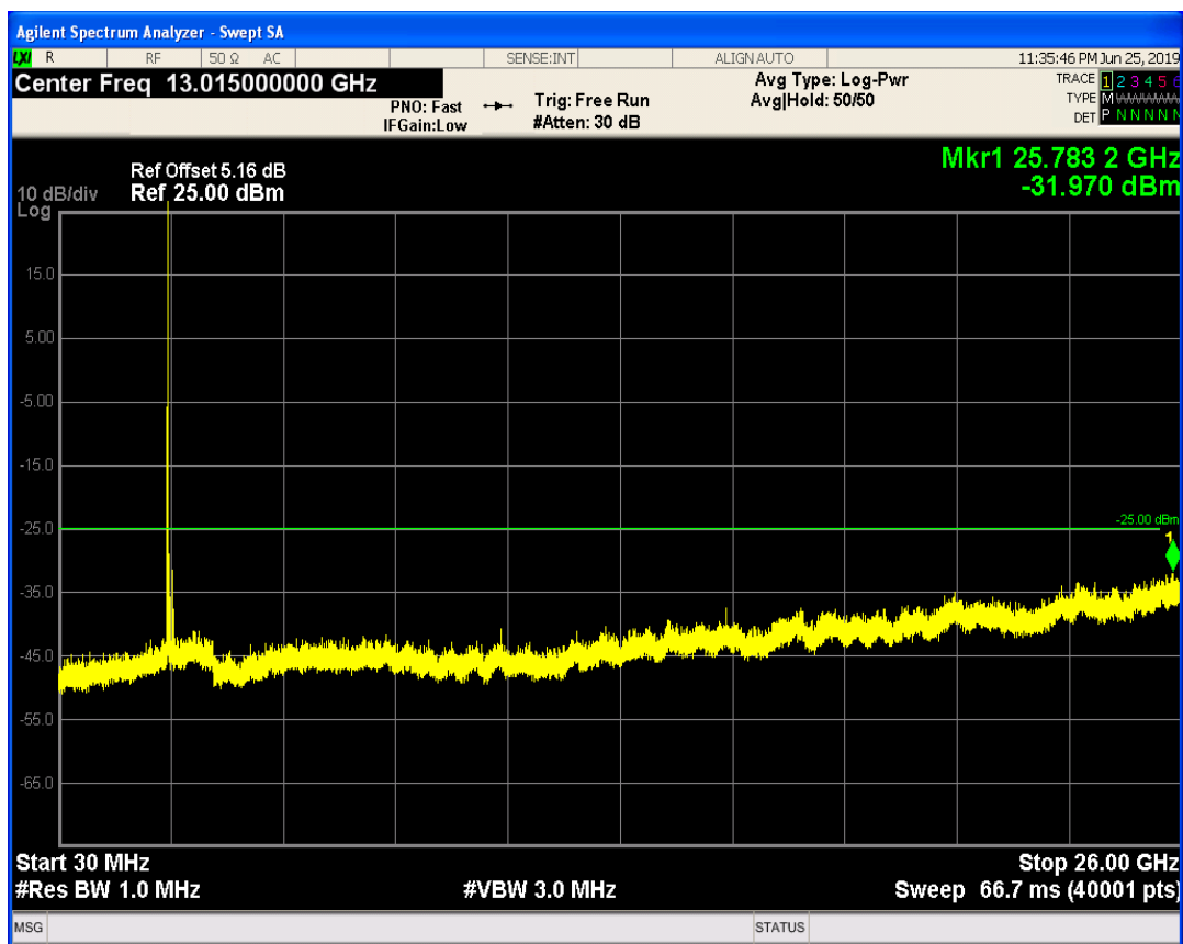
LTE Band41 QAM16 BW=20MHz Channel=40140 RB Size=100 Position=#0
