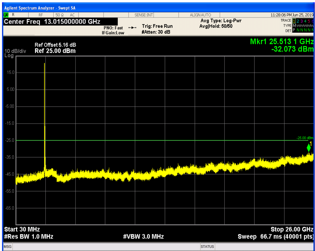
LTE Band41 QAM16 BW=15MHz Channel=40115 RB Size=1 Position=#Max
