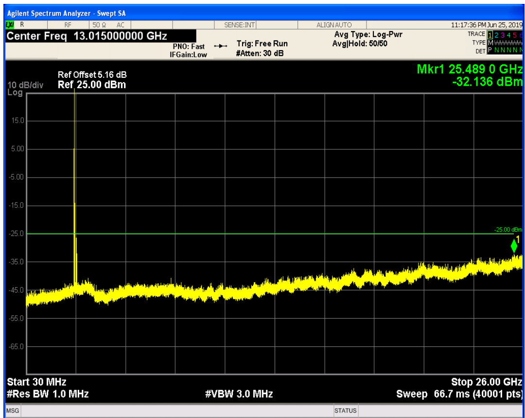
LTE Band41 QAM16 BW=5MHz Channel=41215 RB Size=12 Position=#Max
