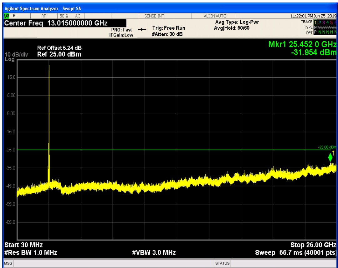
LTE Band41 QAM16 BW=5MHz Channel=40065 RB Size=12 Position=#Max
