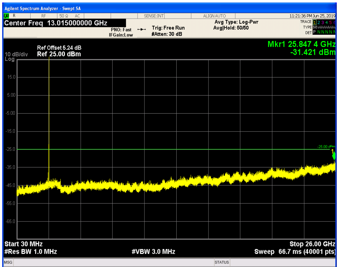
LTE Band41 QPSK BW=10MHz Channel=40090 RB Size=25 Position=#Max
