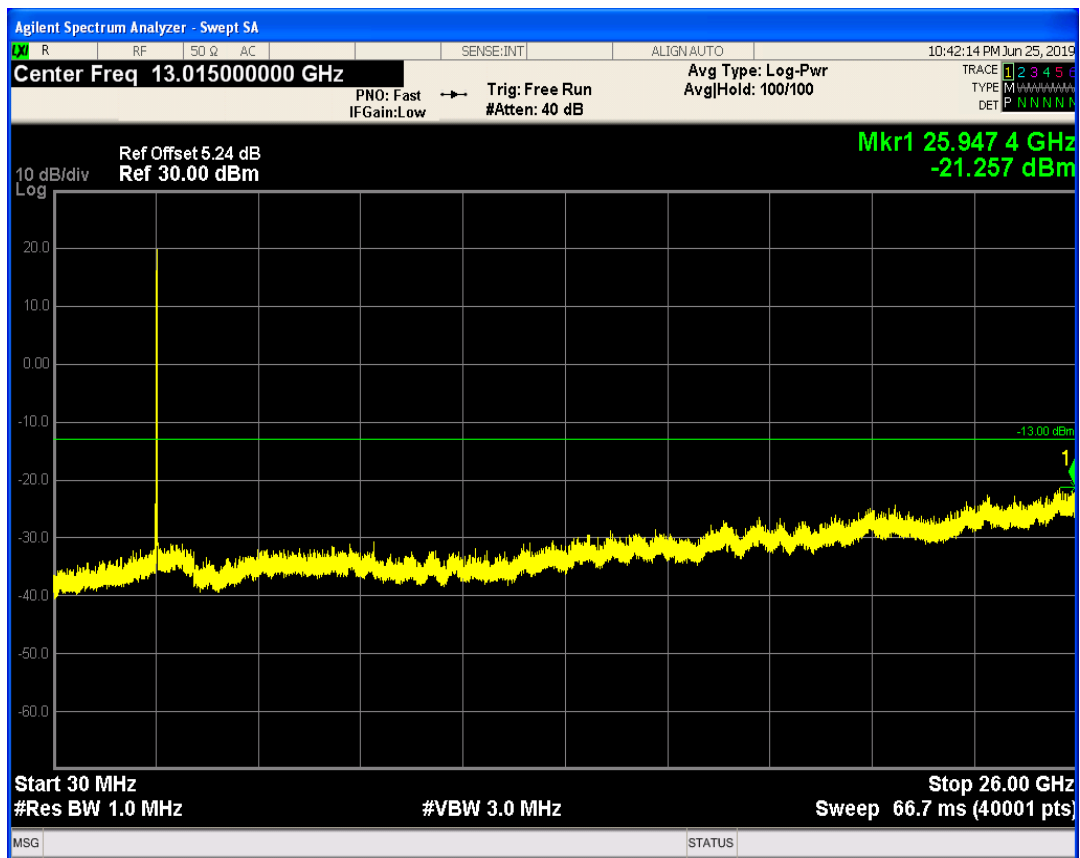
LTE Band41 QAM16 BW=10MHz Channel=40090 RB Size=50 Position=#0
