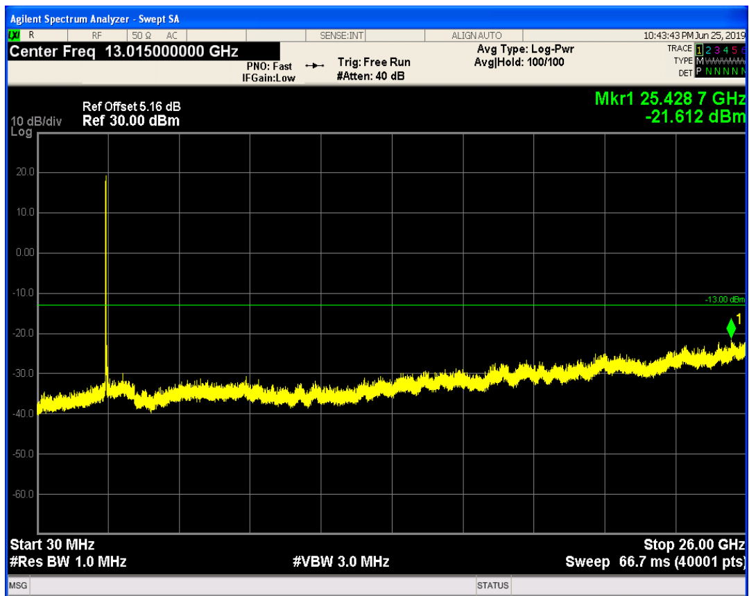
LTE Band41 QAM16 BW=10MHz Channel=41190 RB Size=50 Position=#0
