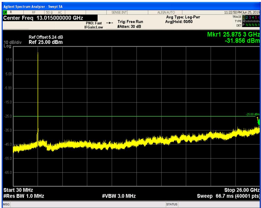
LTE Band41 QPSK BW=10MHz Channel=40090 RB Size=25 Position=#0
