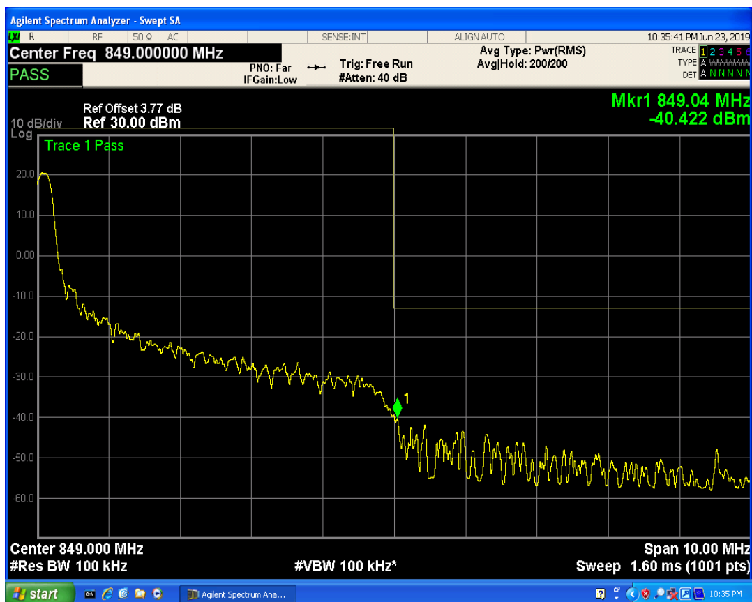
LTE Band5 QPSK BW=10MHz Channel=20600 RB Size=1 Position=#Max
