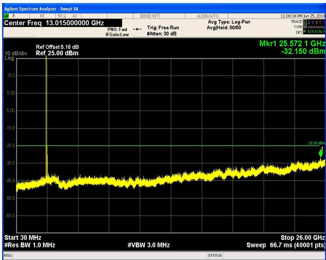
LTE Band41 QPSK BW=20MHz Channel=41140 RB Size=50 Position=#Max
