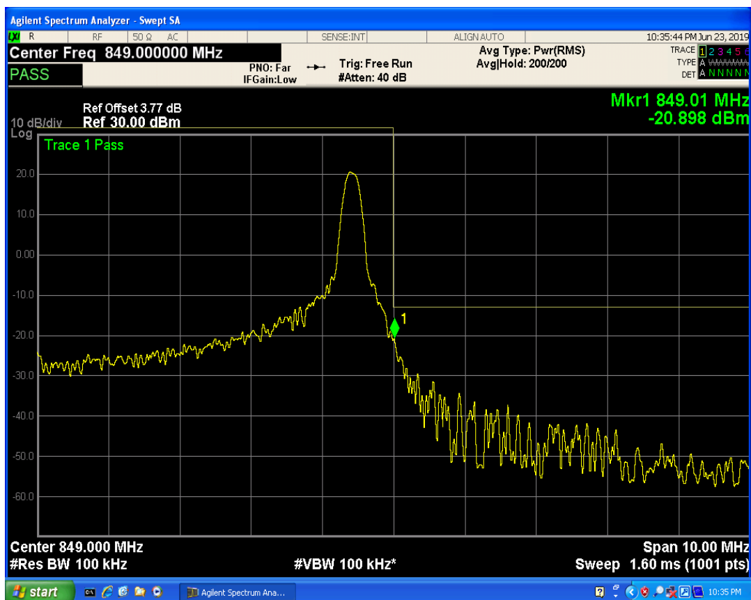
LTE Band5 QPSK BW=10MHz Channel=20600 RB Size=25 Position=#0
