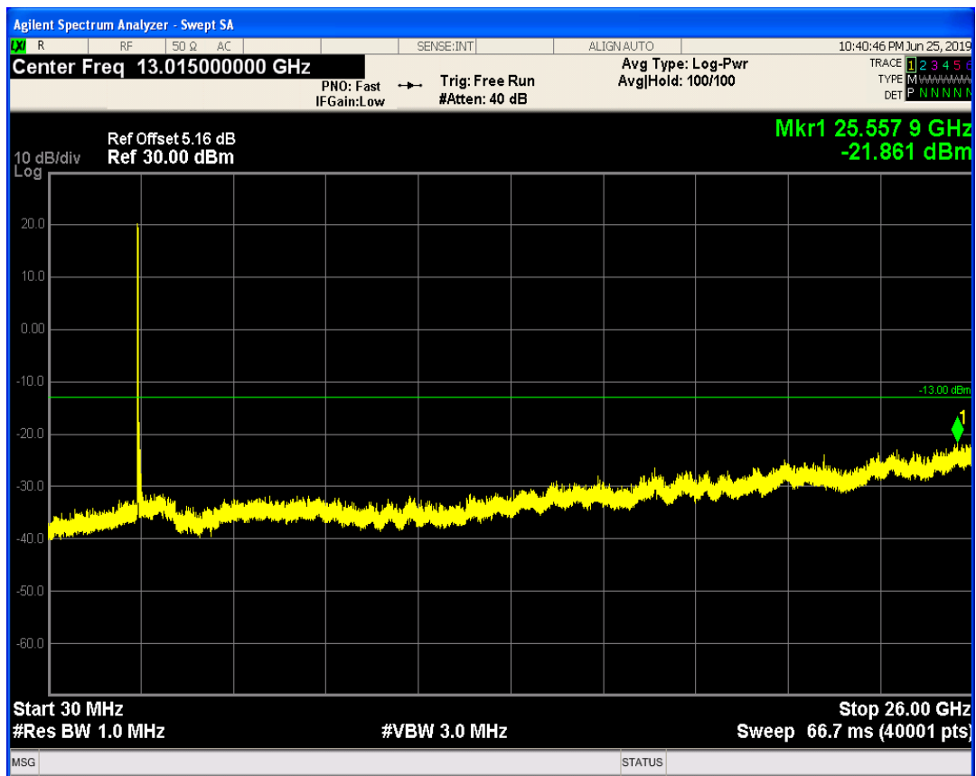
LTE Band41 QAM16 BW=20MHz Channel=41140 RB Size=100 Position=#0
