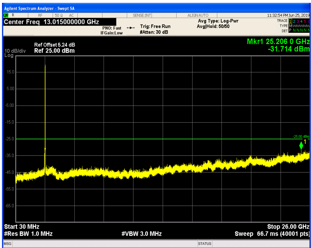
LTE Band41 QPSK BW=10MHz Channel=41190 RB Size=1 Position=#0
