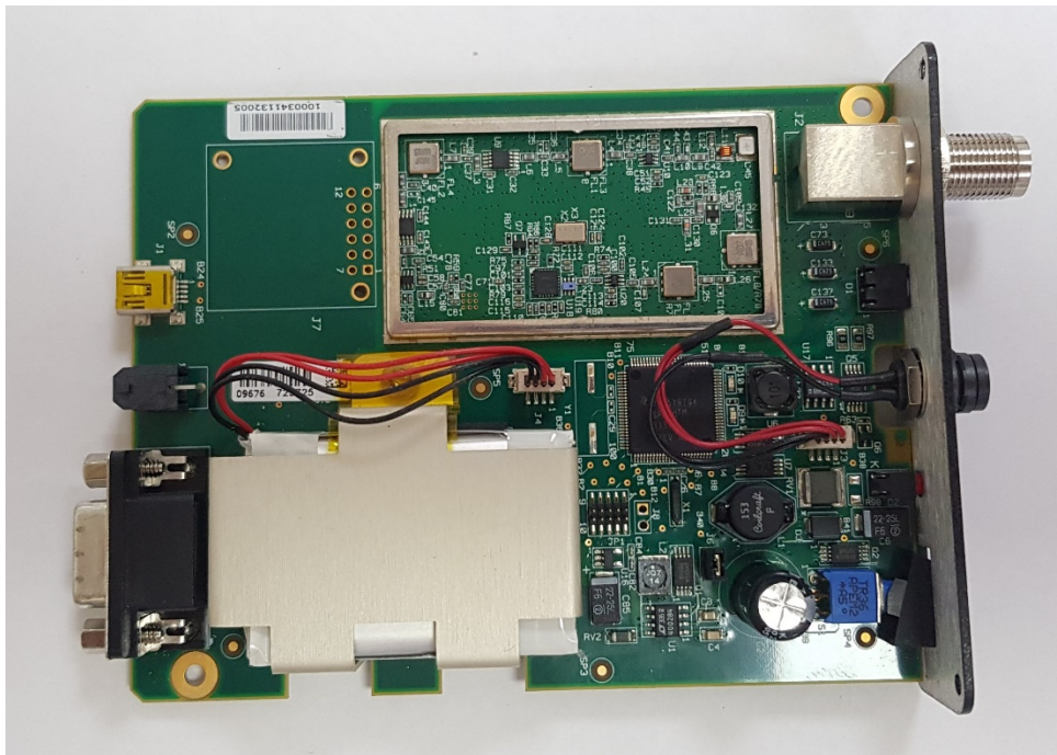
PCB top without RF shield
