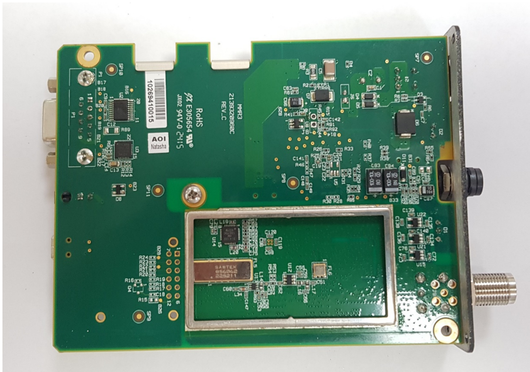
PCB bottom without RF shield
