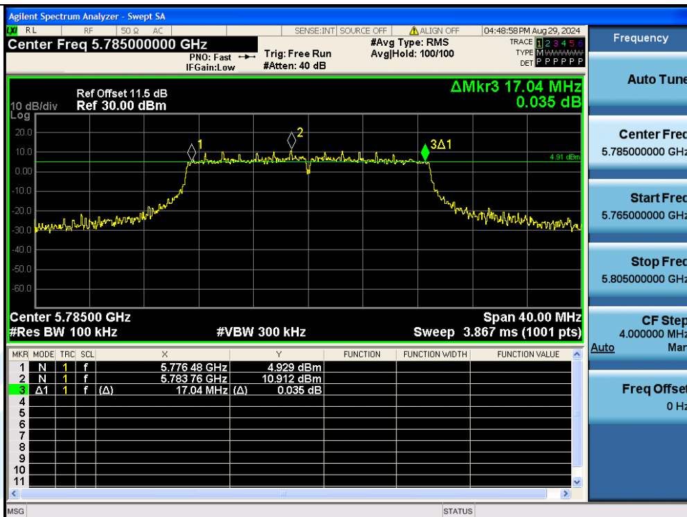
11AC20MIMO-Ant2-5785-PASS
