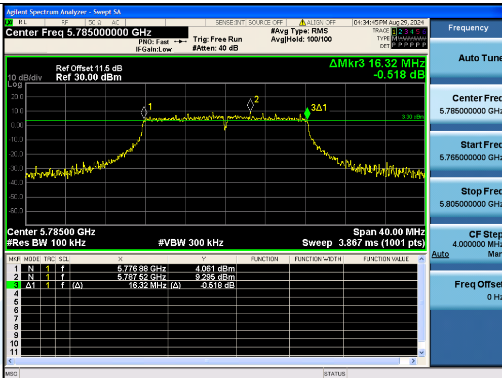
11A-Ant2-5785-PASS
