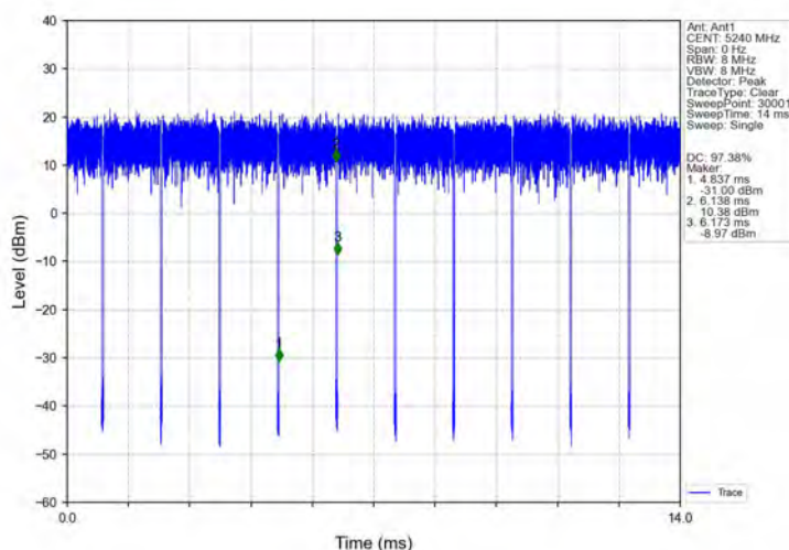
802.11n(HT20)_HCH_5240MHz_Ant1_NTNV
