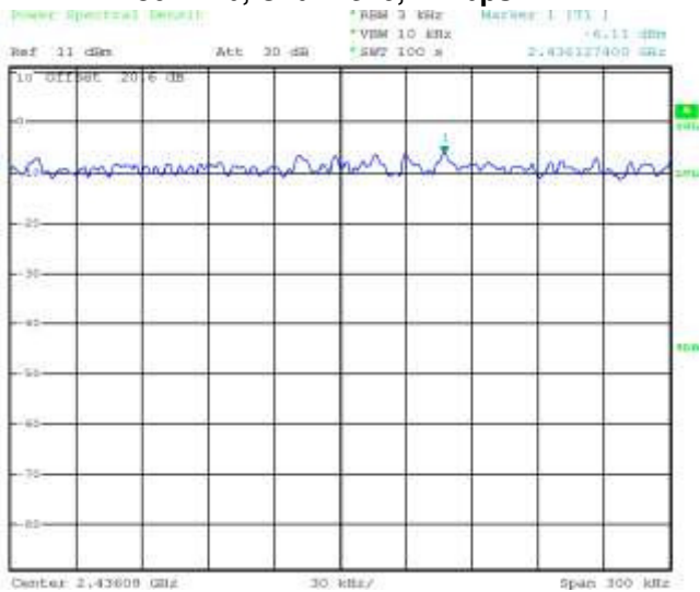
Figure 6-17: Peak Power Spectral Density 802.11b, Channel 6, 1 Mbps
