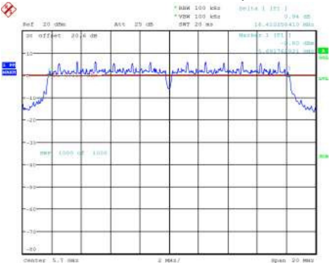
Figure 7-5: 6 dB Bandwidth 802.11a, Channel 140, 6 Mbps
