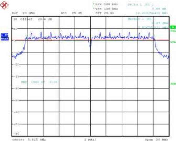
Figure 7-6: 6 dB Bandwidth 802.11a, Channel 165, 6 Mbps
