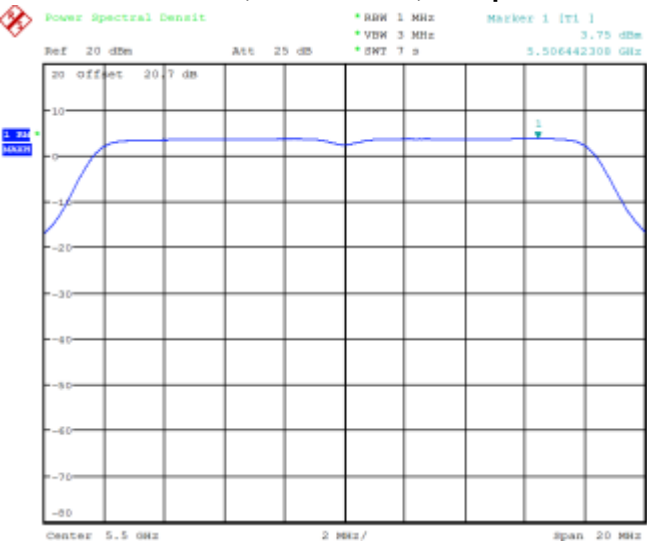
Figure 7-25: Peak Power Spectral Density 802.11a, Channel 100, 6 Mbps
