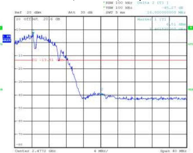
Figure 6-11: Band Edge Compliance 802.11b, Channel 11, 1 Mbps
