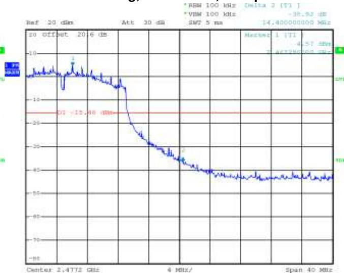
Figure 6-13: Band Edge Compliance 802.11g, Channel 11, 6 Mbps
