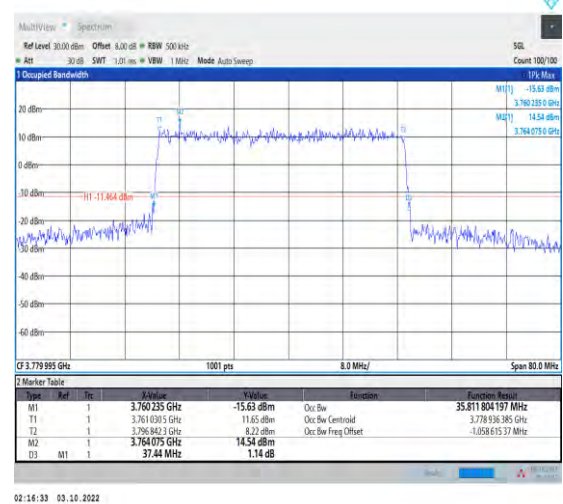
1-N78-3700-3800-PASS-30-40-H-4-DFT-64QAM-Out er_Full-100@0-Ant1-35.812-37.440-≤40-PASS
