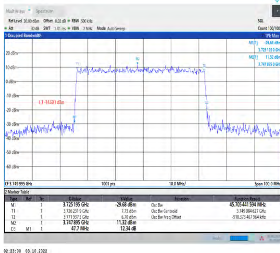
1-N78-3700-3800-PASS-30-50-M-5-DFT-256QAM-Out er_Full-128@0-Ant1-45.705-47.700-≤50-PASS
