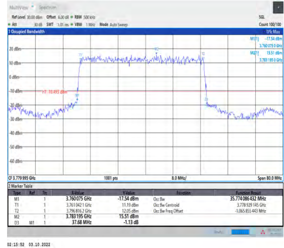
1-N78-3700-3800-PASS-30-40-H-2-DFT-PI2BPSK-O uter_Full-100@0-Ant1-35.774-37.680-≤40-PASS
