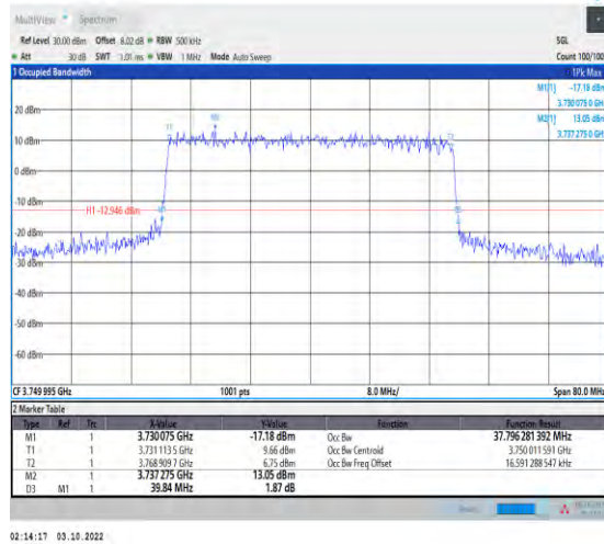
1-N78-3700-3800-PASS-30-40-M-6-CP-QPSK-Outer_Full-106@0-Ant1-37.796-39.840-≤40-PASS
