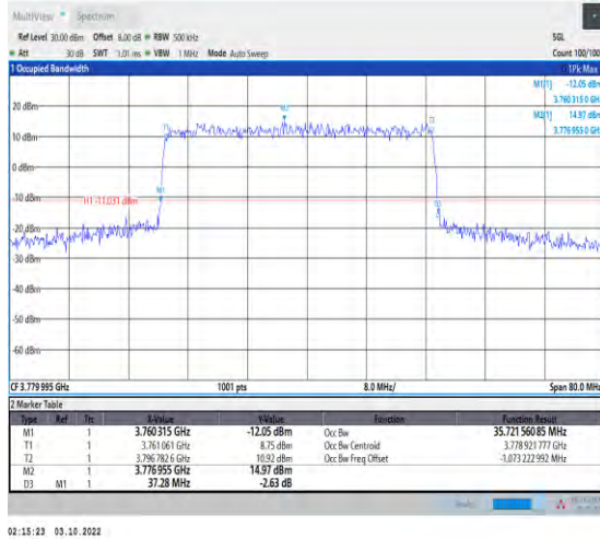
1-N78-3700-3800-PASS-30-40-H-1-DFT-QPSK-Out er_Full-100@0-Ant1-35.722-37.280-≤40-PASS
