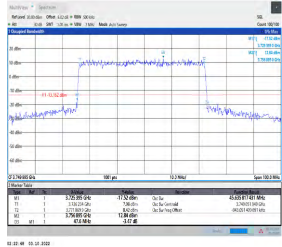
1-N78-3700-3800-PASS-30-50-M-4-DFT-64QAM-Out er_Full-128@0-Ant1-45.636-47.600-≤50-PASS
