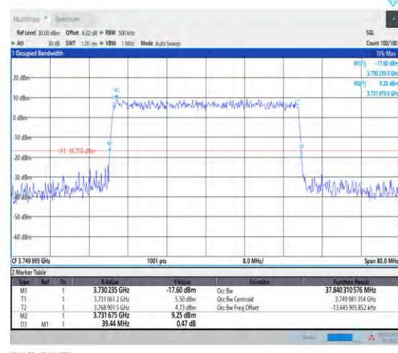
1-N78-3700-3800-PASS-30-40-M-9-CP-256QAM-Outer_Full-106@0-Ant1-37.84-39.440-≤40-PASS
