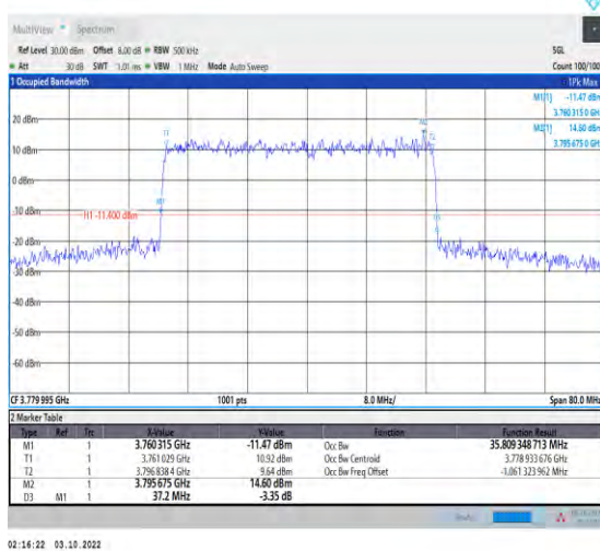
1-N78-3700-3800-PASS-30-40-H-3-DFT-16QAM-Ou ter_Full-100@0-Ant1-35.809-37.200-≤40-PASS
