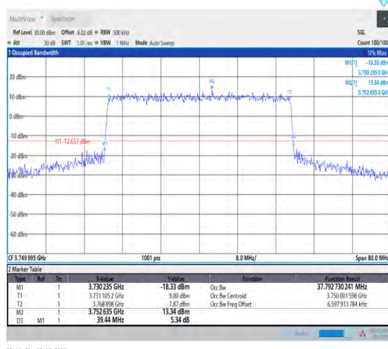
1-N78-3700-3800-PASS-30-40-M-8-CP-64QAM-Outer_Full-106@0-Ant1-37.793-39.440-≤40-PASS
