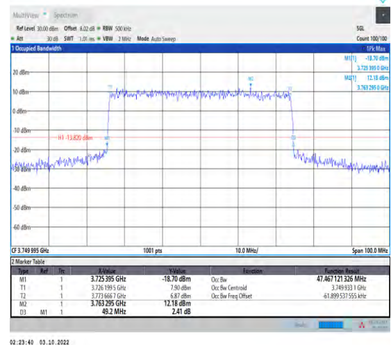
1-N78-3700-3800-PASS-30-50-M-6-CP-QPSK-Outer_Full-133@0-Ant1-47.467-49.200-≤50-PASS
