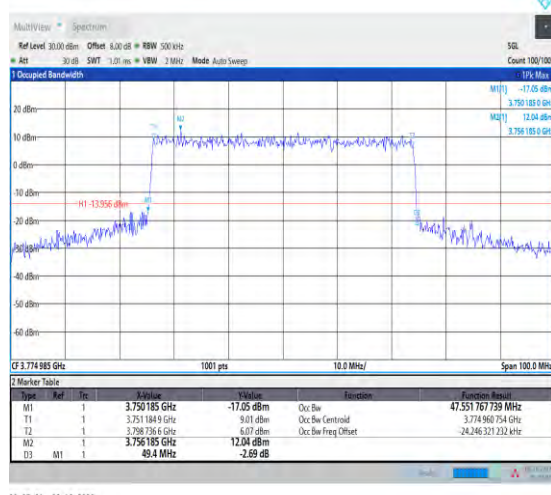
1-N78-3700-3800-PASS-30-50-H-8-CP-64QAM-Outer_Full-133@0-Ant1-47.552-49.400-≤50-PASS
