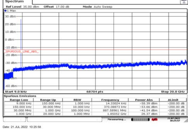
GPRS 1900 CH-Low 9kHz ~ 20GHz
