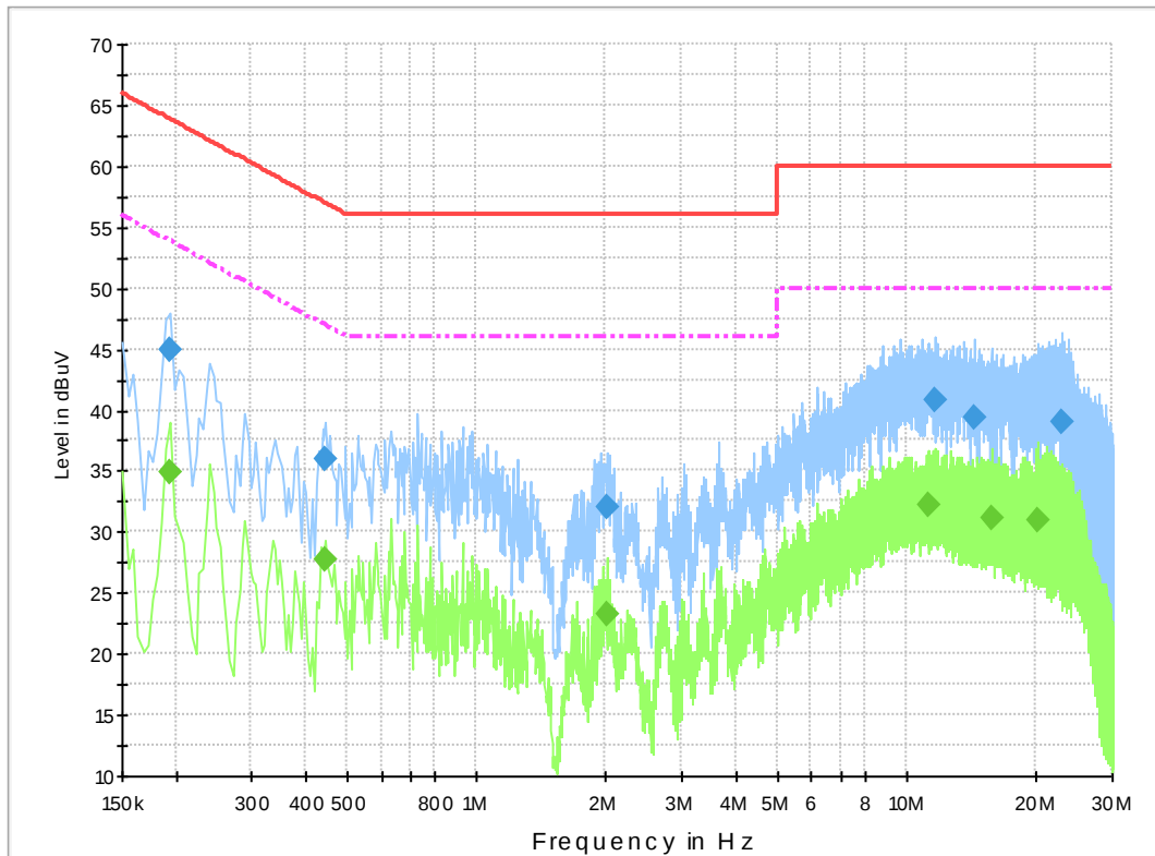
Fig.B.11.2 AC Powerline Conducted Emission-Idle
