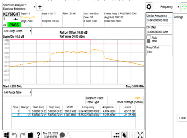
802.11ax_20MHz_Chain0_5845MHz
