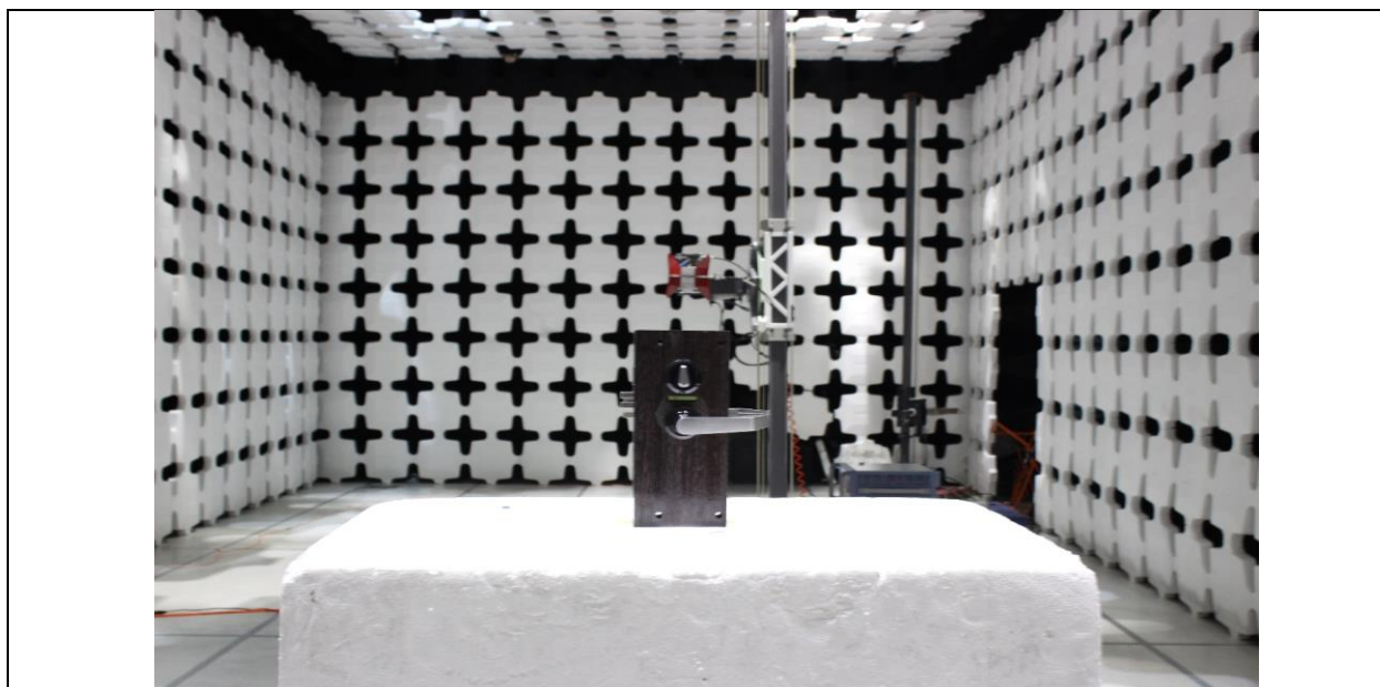
Radiated Emission Test Above 1GHz Front View
