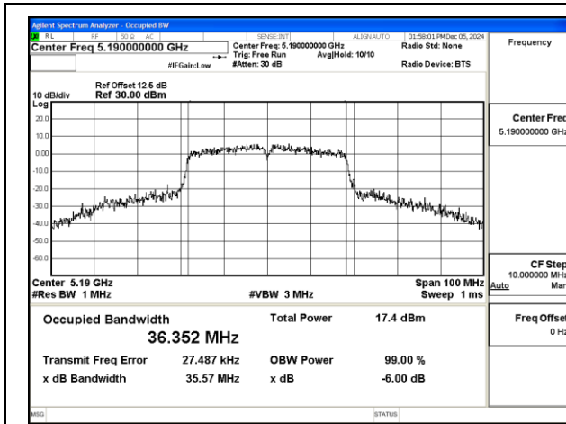
Mode:802.11n HT40 Frequency:5190MHz Ant:Chain1
