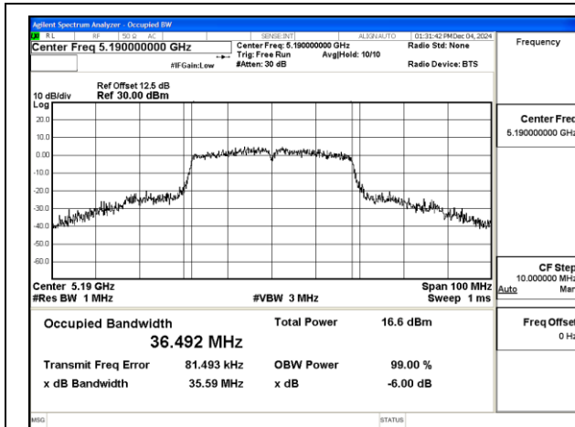
Mode:802.11ac VHT40 Frequency:5190MHz Ant:Chain0
