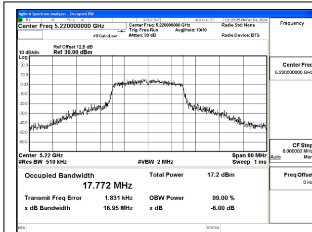
Mode:802.11ac VHT20 Frequency:5220MHz Ant:Chain1
