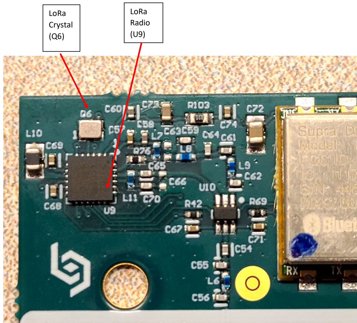
Photo 4 – Closeup of LoRa Crystal and Radio
