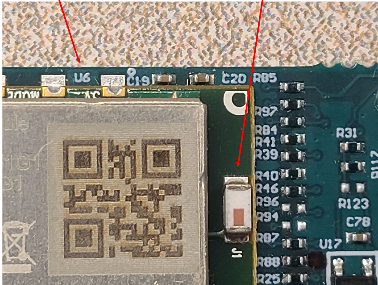
Photo 5 – Closeup of Bluetooth module, including Antenna
