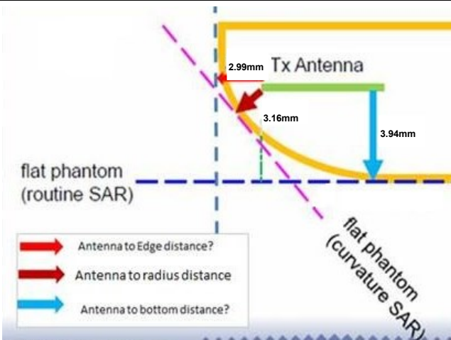
X=2.99mm, Y=3.94mm, Z=3.16mm Exterior Radius Dimension For WLAN
