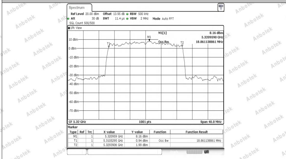
11AX20SISO-Ant1-5320
