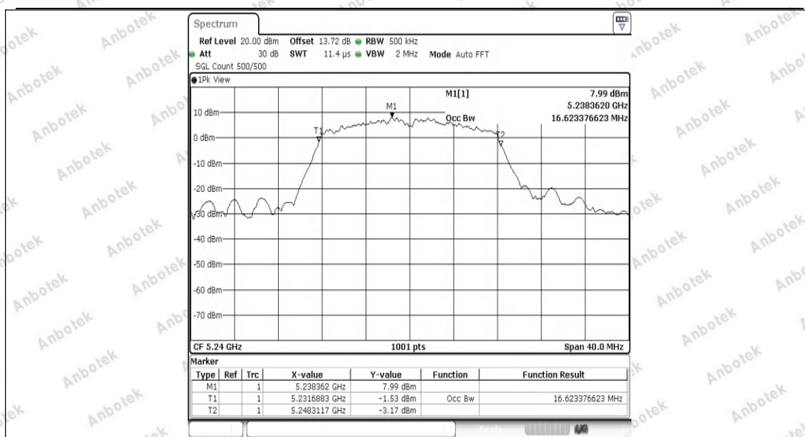
11A-Ant1-5240
