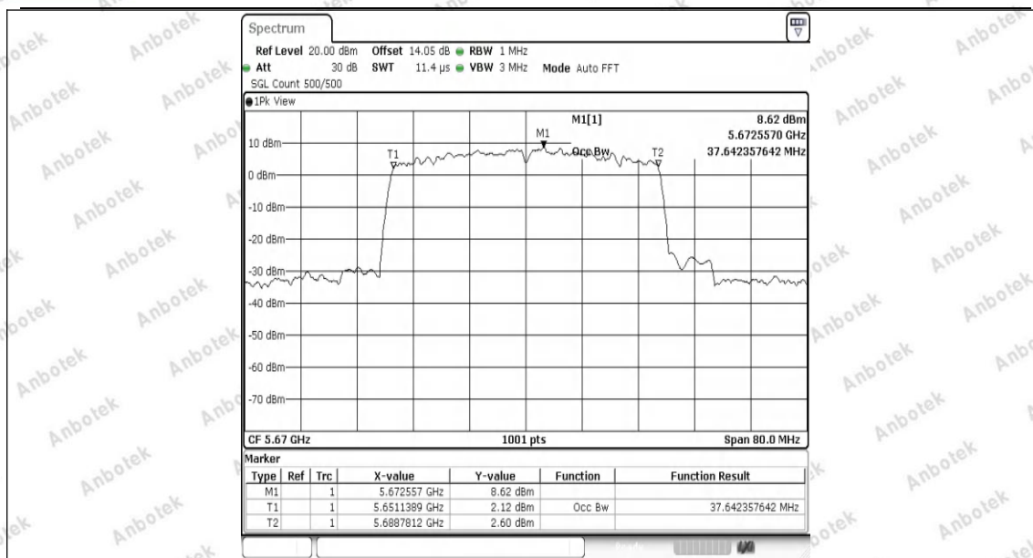
11AX40SISO-Ant1-5670
