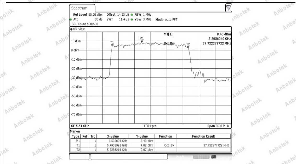
11AX40SISO-Ant1-5510
