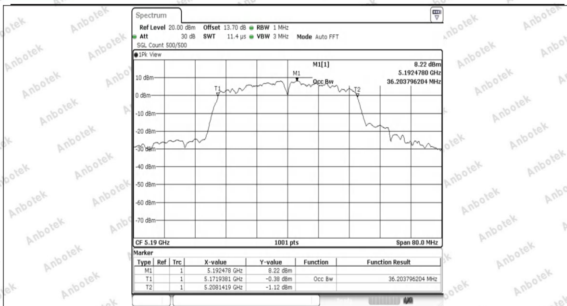
11N40SISO-Ant1-5190
