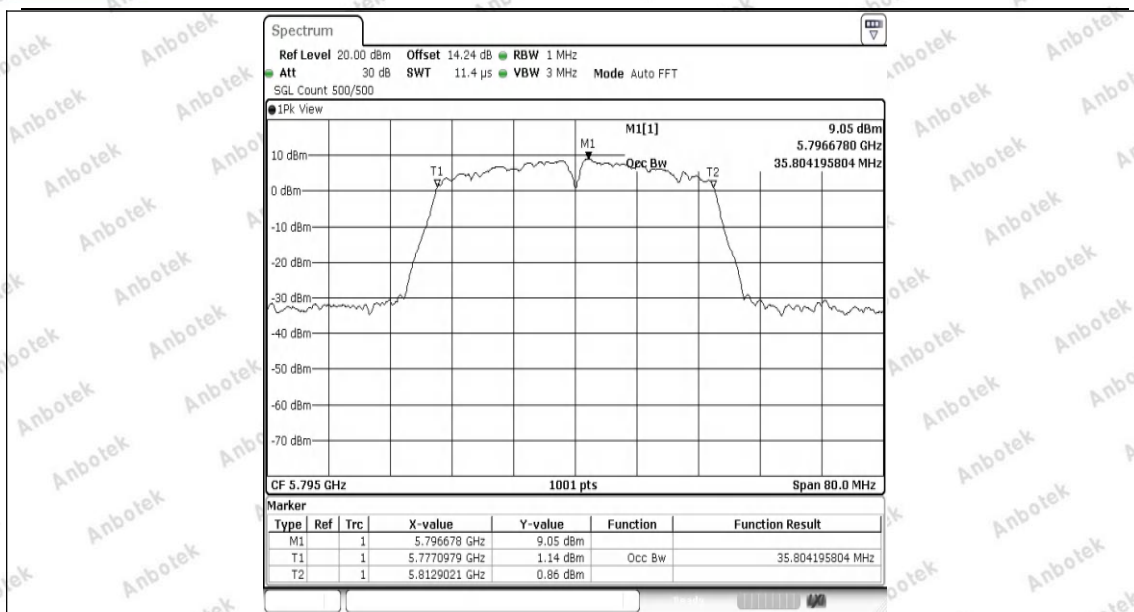
11N40SISO-Ant1-5795
