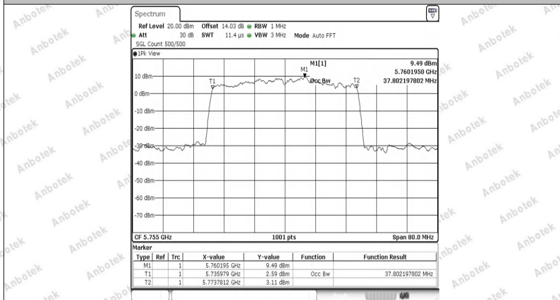
11AX40SISO-Ant1-5755
