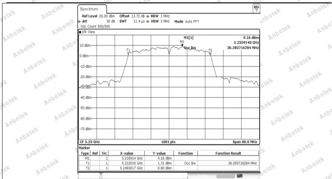
11AC40SISO-Ant1-5230
