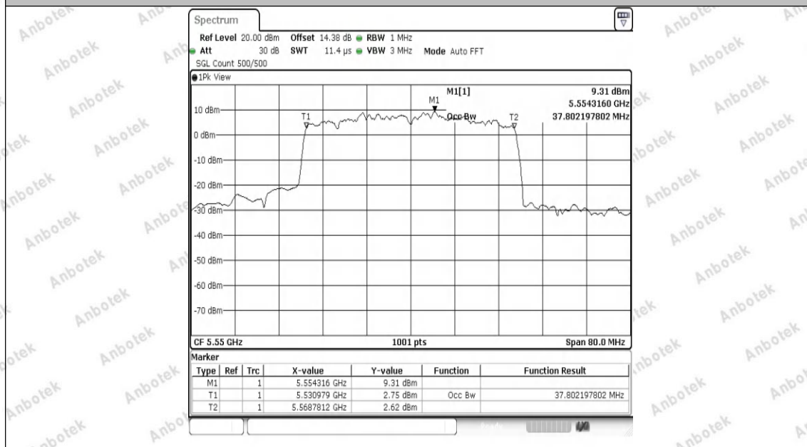
11AX40SISO-Ant1-5550
