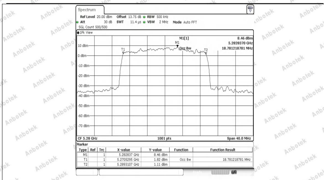
11AX20SISO-Ant1-5280
