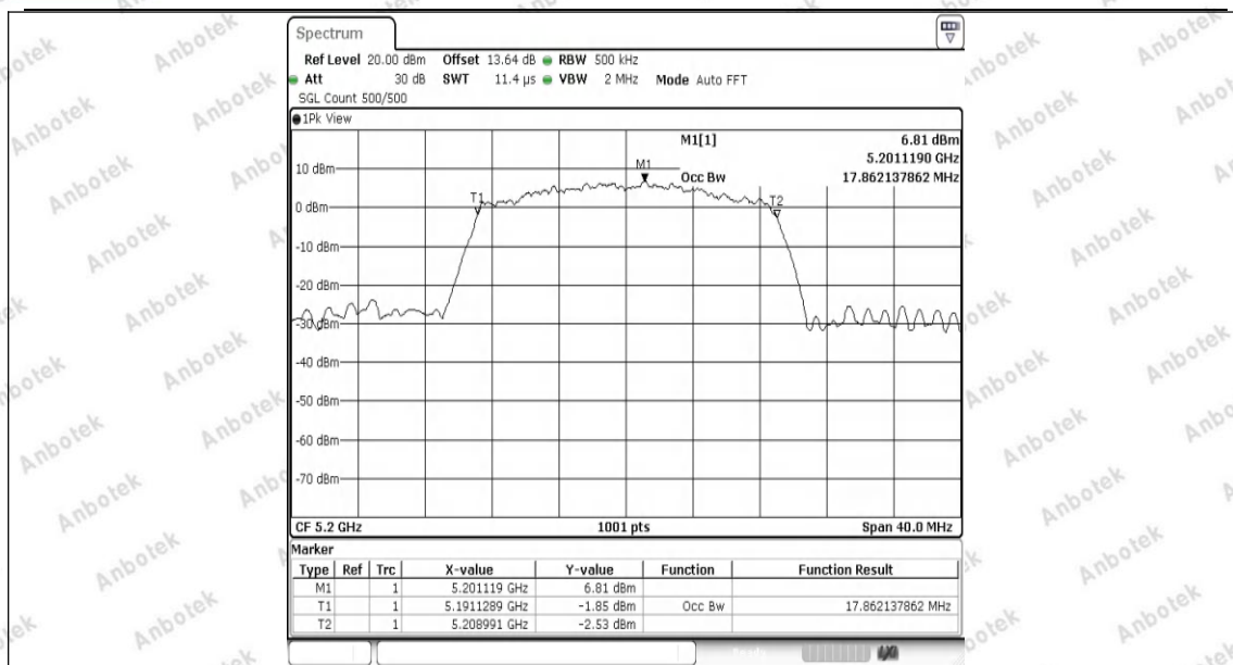
11AC20SISO-Ant1-5200
