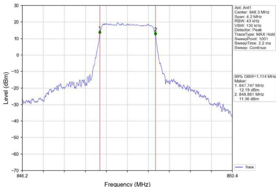
Band5_1.4MHz_16QAM_HCH_848.3MHz_RB_6_0_NTNV
