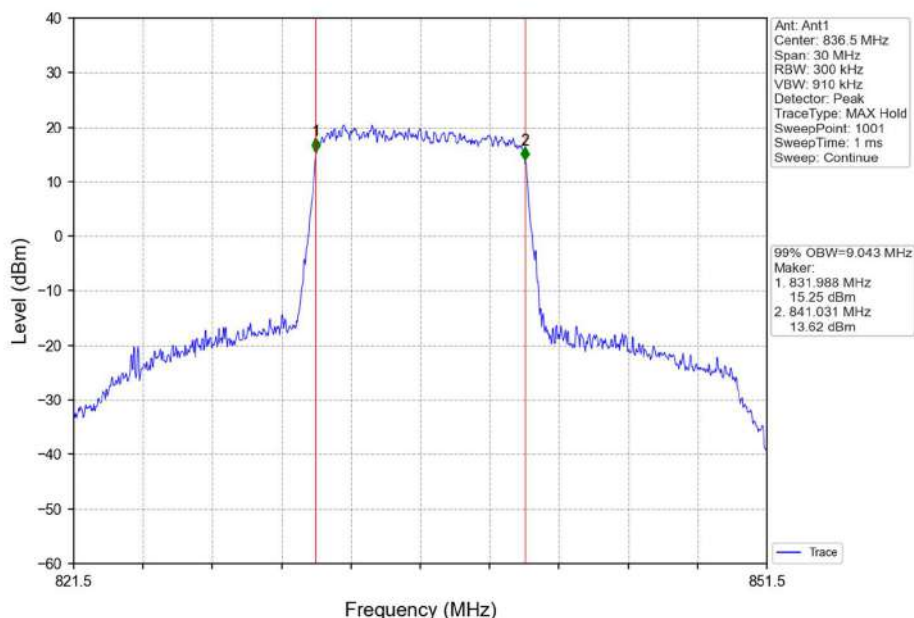
Band5_10MHz_QPSK_MCH_836.5MHz_RB_50_0_NTNV
