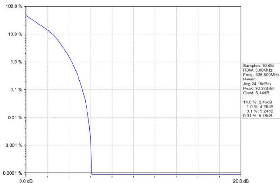
Band5_3MHz_QPSK_MCH_836.5MHz_RB_15_0_NTNV
