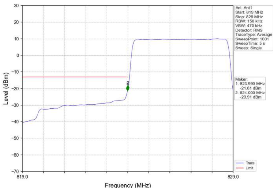
Band5_5MHz_QPSK_LCH_826.5MHz_RB_25_0_NTNV
