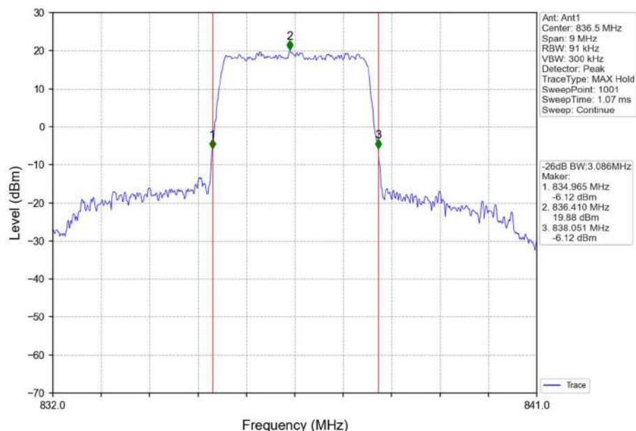
Band5_3MHz_QPSK_MCH_836.5MHz_RB_15_0_NTNV
