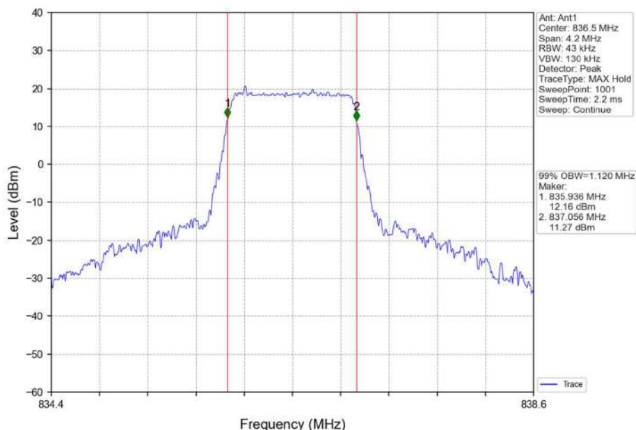
Band5_1.4MHz_16QAM_MCH_836.5MHz_RB_6_0_NTNV
