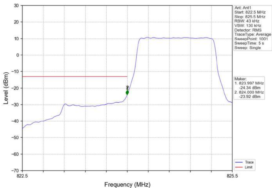
Band5_1.4MHz_QPSK_LCH_824.7MHz_RB_6_0_NTNV
