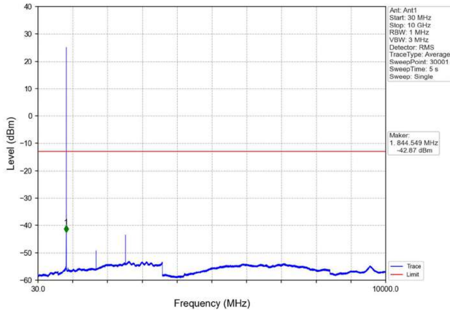
Band5_1.4MHz_QPSK_HCH_848.3MHz_RB_1_0_NTNV
