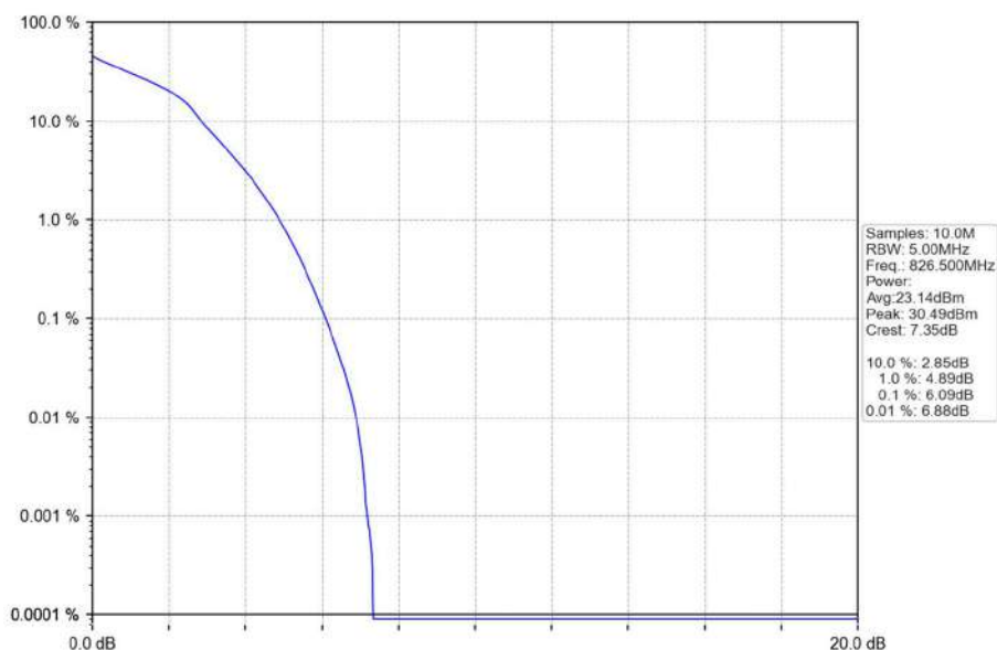
Band5_5MHz_16QAM_LCH_826.5MHz_RB_25_0_NTNV
