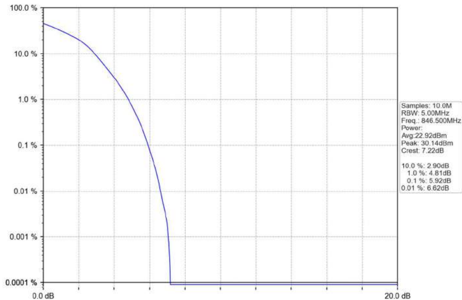
Band5_5MHz_16QAM_HCH_846.5MHz_RB_25_0_NTNV
