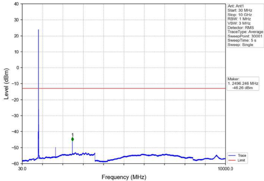
Band5_10MHz_16QAM_MCH_836.5MHz_RB_1_0_NTNV
