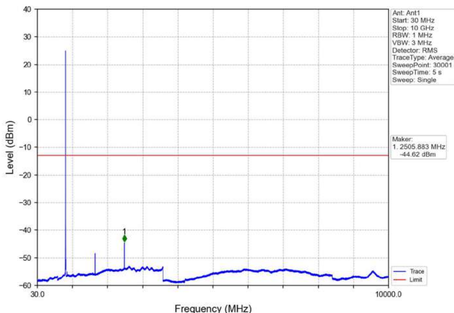
Band5_3MHz_QPSK_MCH_836.5MHz_RB_1_0_NTNV
