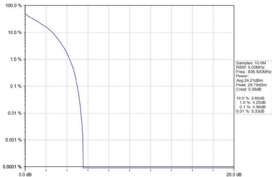
Band5_1.4MHz_QPSK_MCH_836.5MHz_RB_6_0_NTNV
