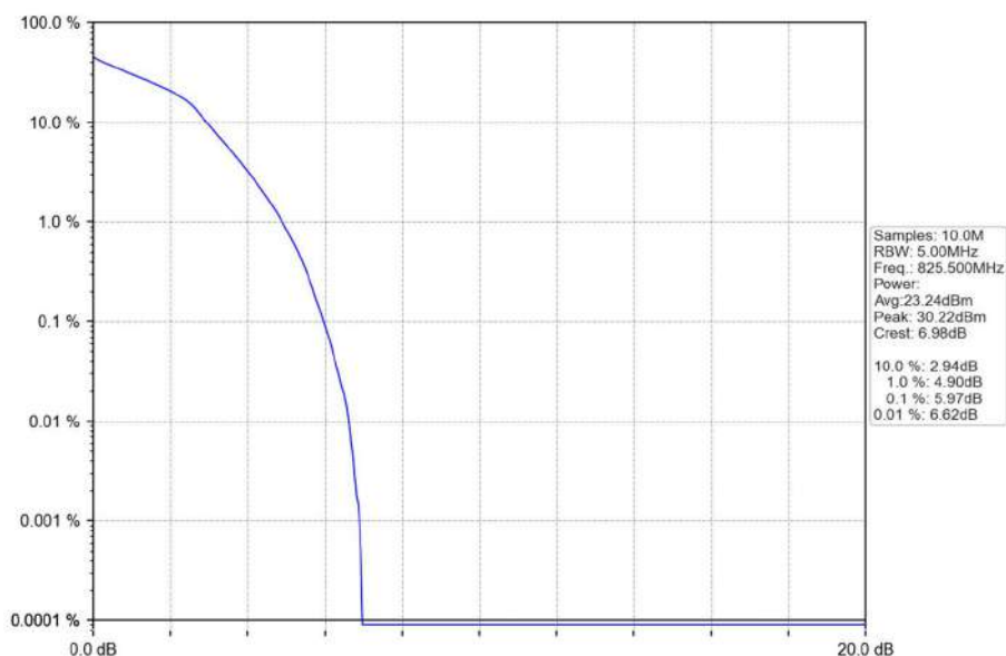
Band5_3MHz_16QAM_LCH_825.5MHz_RB_15_0_NTNV
