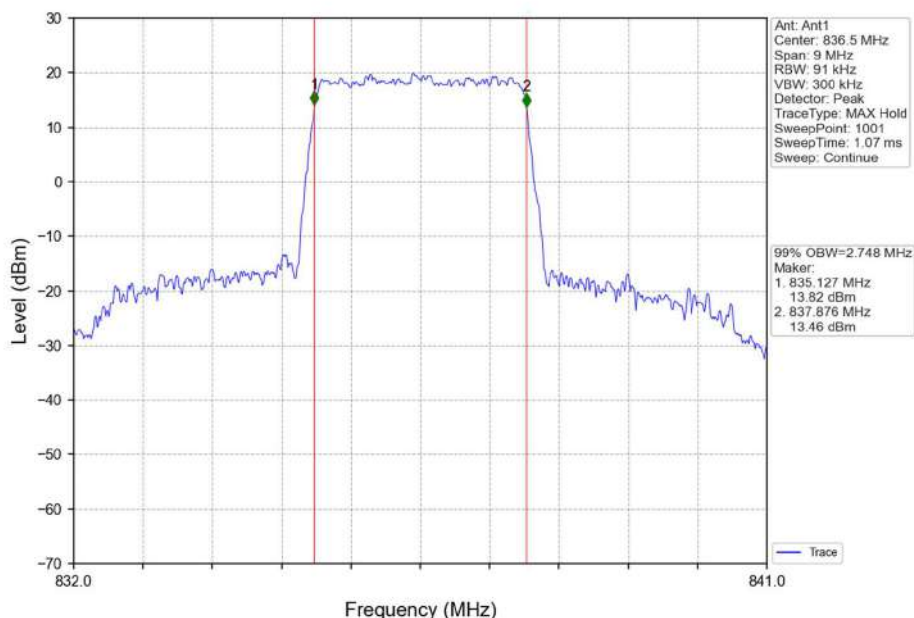
Band5_3MHz_QPSK_MCH_836.5MHz_RB_15_0_NTNV
