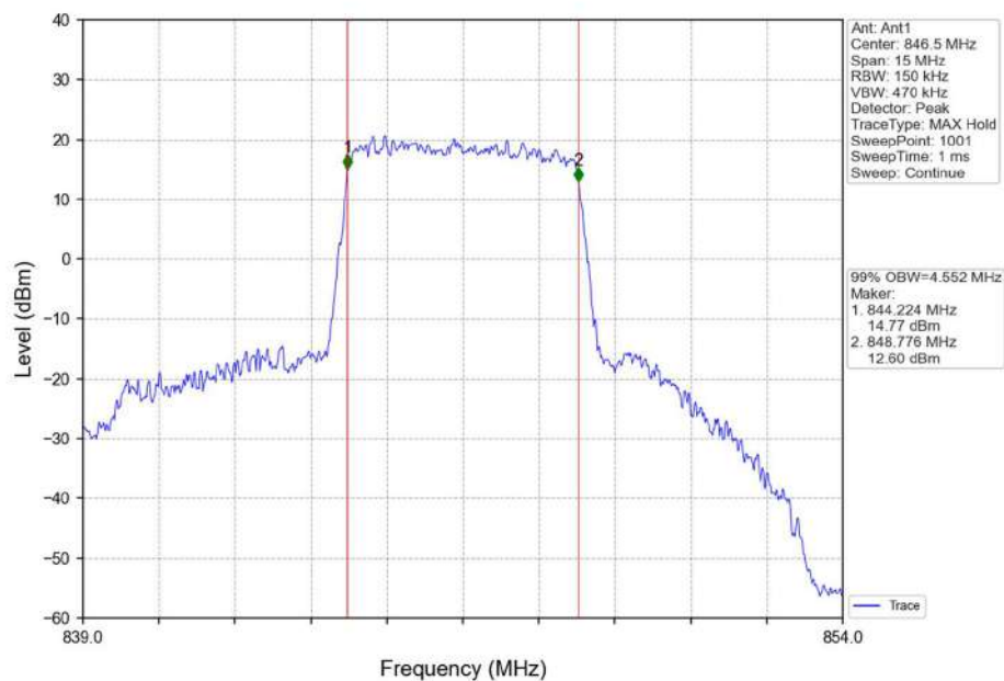
Band5_5MHz_QPSK_HCH_846.5MHz_RB_25_0_NTNV
