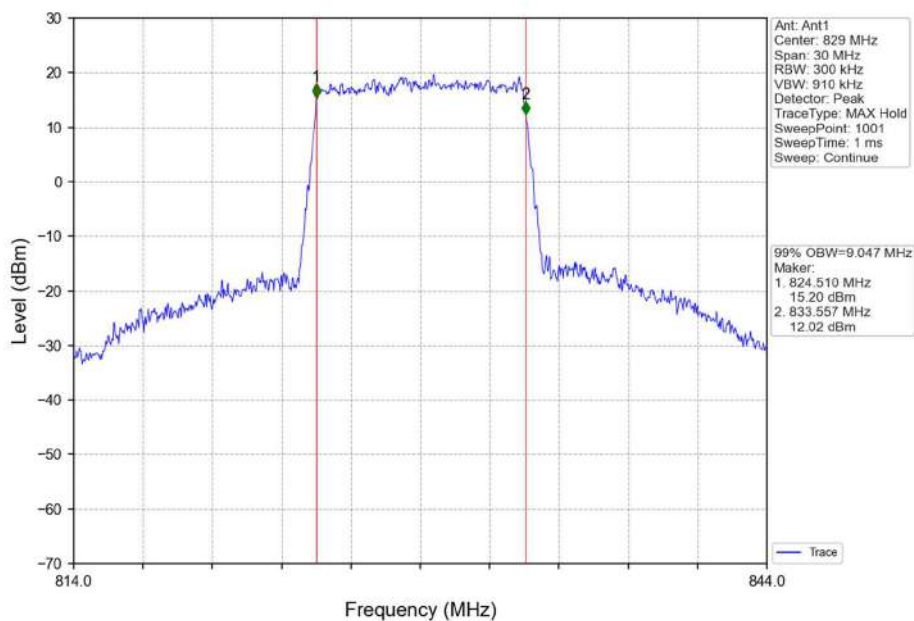
Band5_10MHz_16QAM_LCH_829MHz_RB_50_0_NTNV
