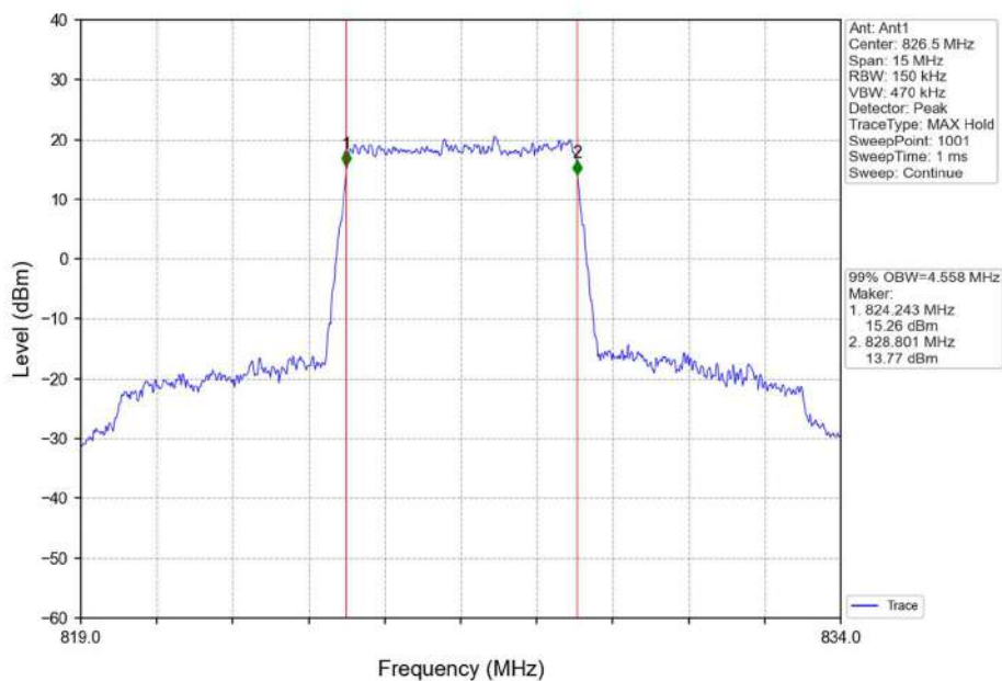
Band5_5MHz_QPSK_LCH_826.5MHz_RB_25_0_NTNV
