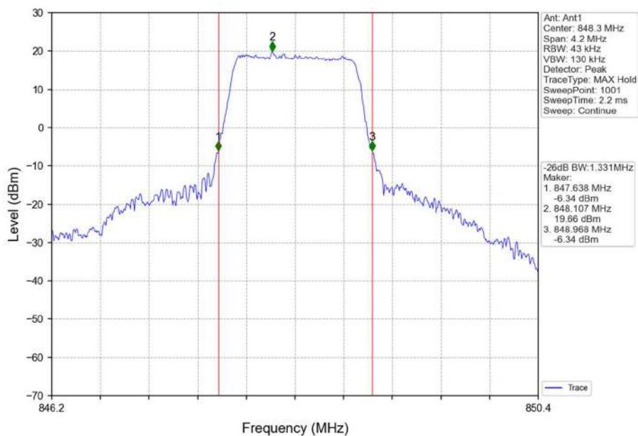
Band5_1.4MHz_16QAM_HCH_848.3MHz_RB_6_0_NTNV
