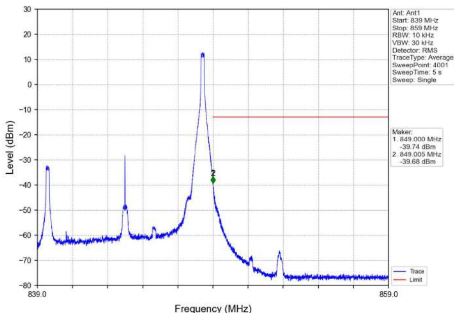
Band5_10MHz_16QAM_HCH_844MHz_RB_1_49_NTNV
