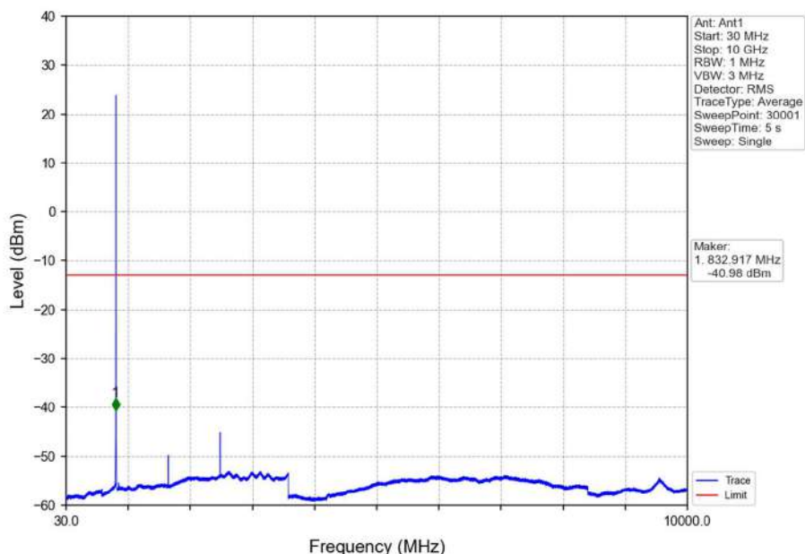
Band5_1.4MHz_16QAM_MCH_836.5MHz_RB_1_0_NTNV
