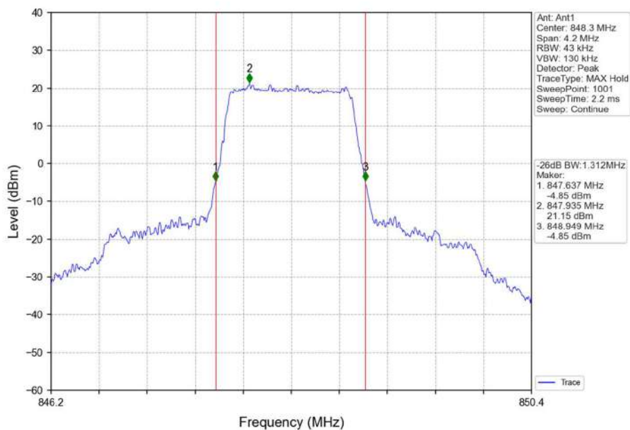
Band5_1.4MHz_QPSK_HCH_848.3MHz_RB_6_0_NTNV
