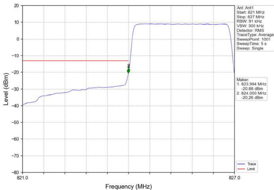
Band5_3MHz_16QAM_LCH_825.5MHz_RB_15_0_NTNV
