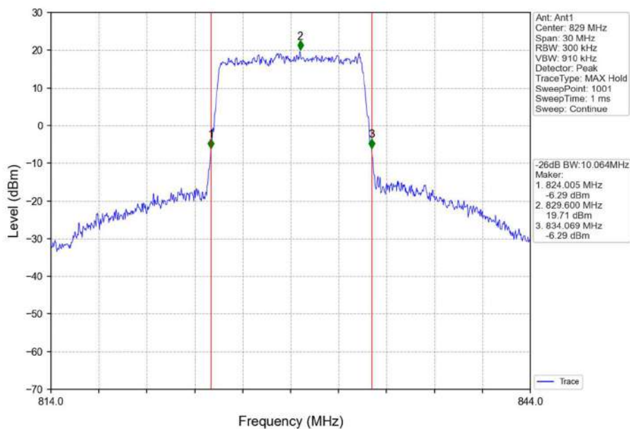
Band5_10MHz_16QAM_LCH_829MHz_RB_50_0_NTNV
