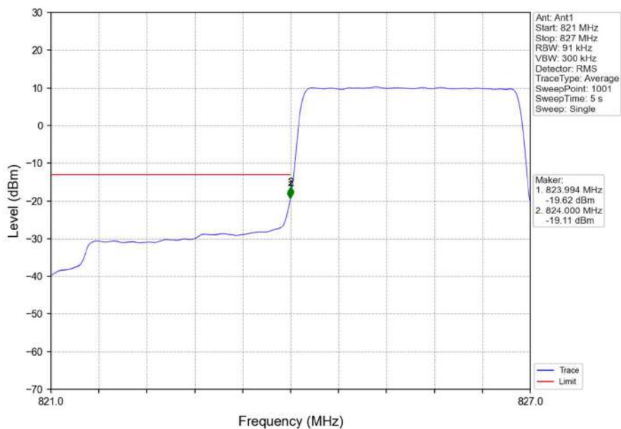
Band5_3MHz_QPSK_LCH_825.5MHz_RB_15_0_NTNV
