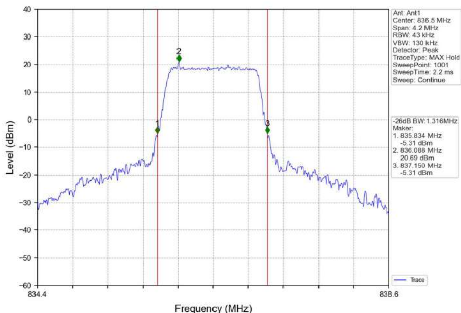
Band5_1.4MHz_16QAM_MCH_836.5MHz_RB_6_0_NTNV
