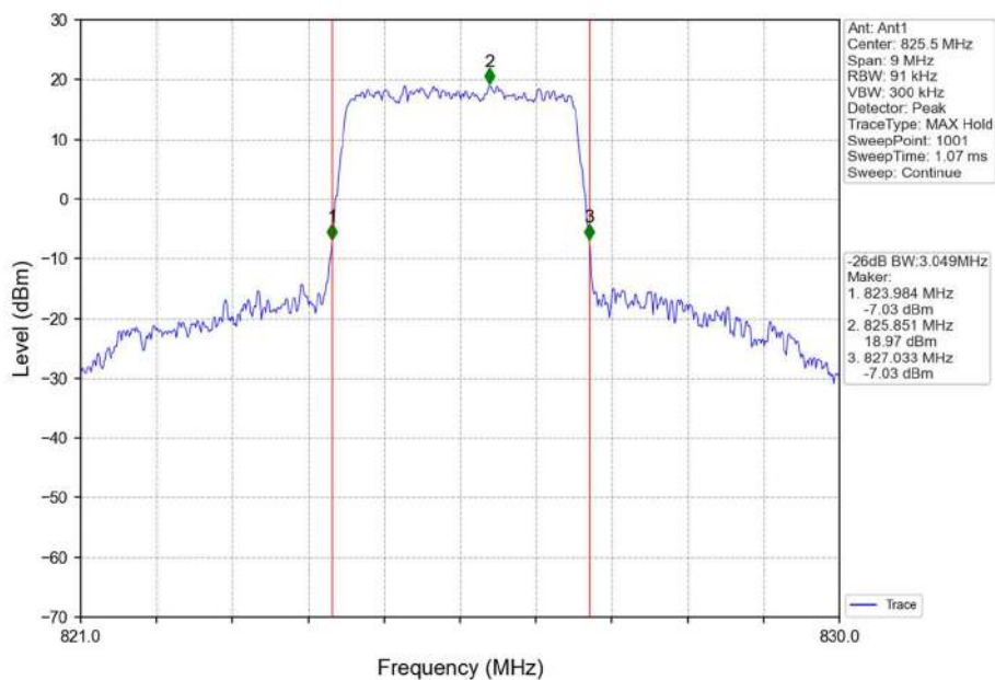
Band5_3MHz_16QAM_LCH_825.5MHz_RB_15_0_NTNV
