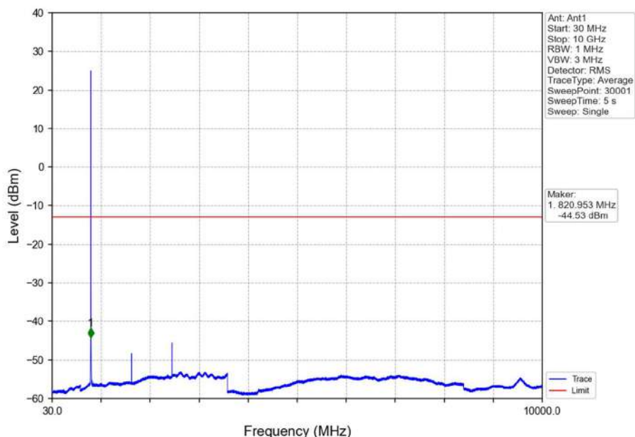
Band5_1.4MHz_QPSK_LCH_824.7MHz_RB_1_0_NTNV
