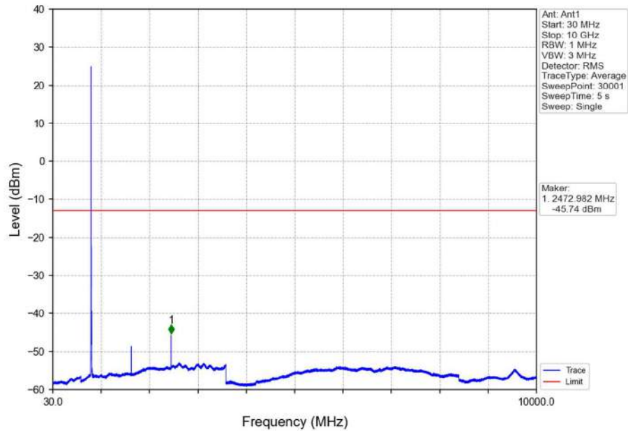
Band5_5MHz_QPSK_LCH_826.5MHz_RB_1_0_NTNV
