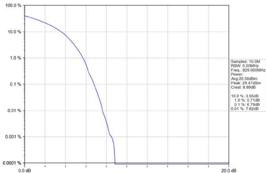
Band5_10MHz_16QAM_LCH_829MHz_RB_50_0_NTNV
