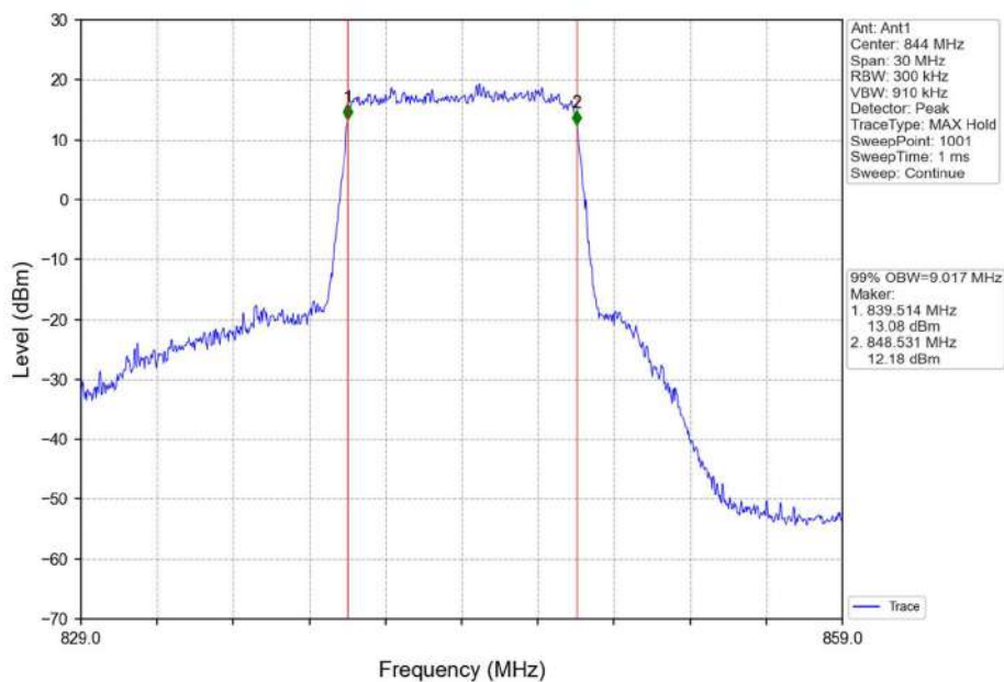
Band5_10MHz_16QAM_HCH_844MHz_RB_50_0_NTNV
