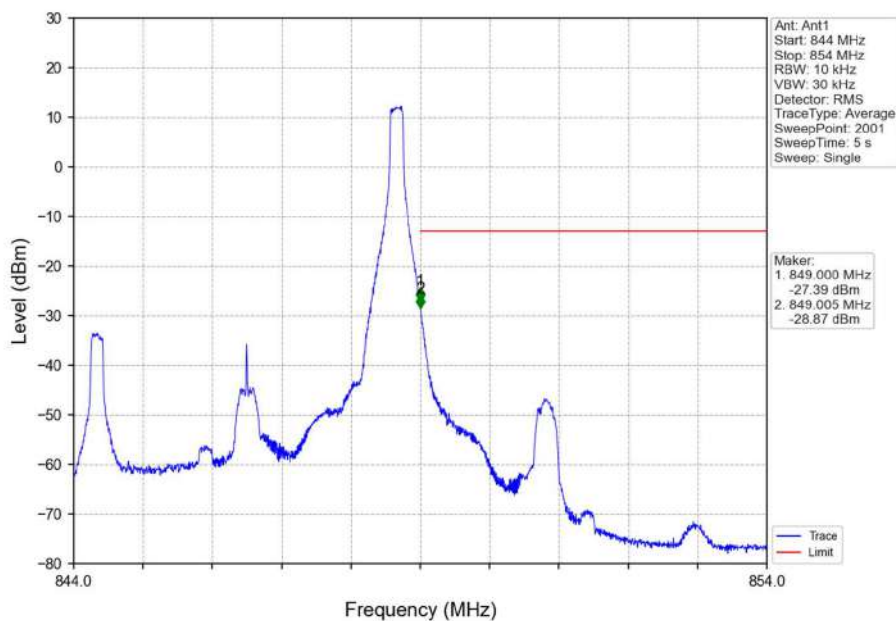
Band5_5MHz_16QAM_HCH_846.5MHz_RB_1_24_NTNV
