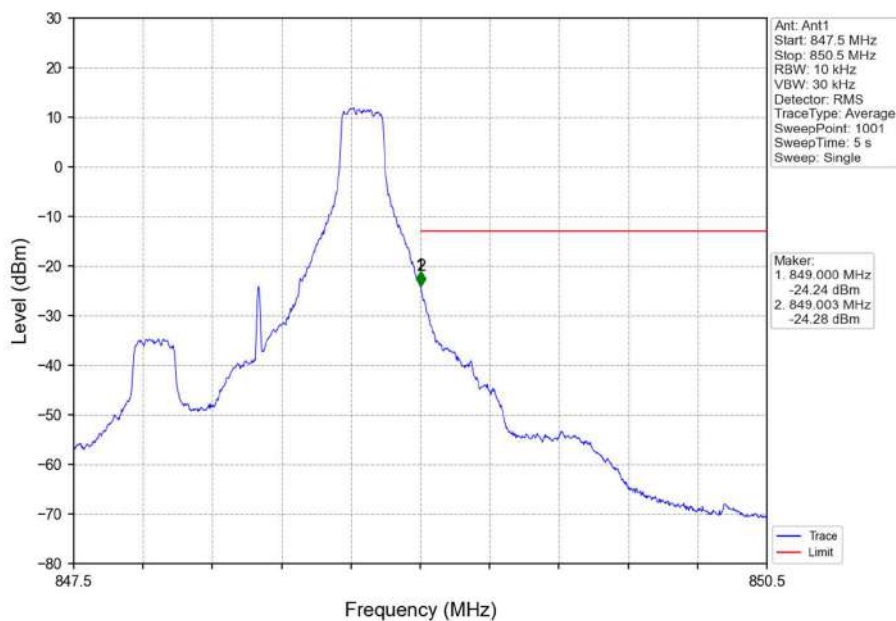
Band5_1.4MHz_QPSK_HCH_848.3MHz_RB_1_5_NTNV
