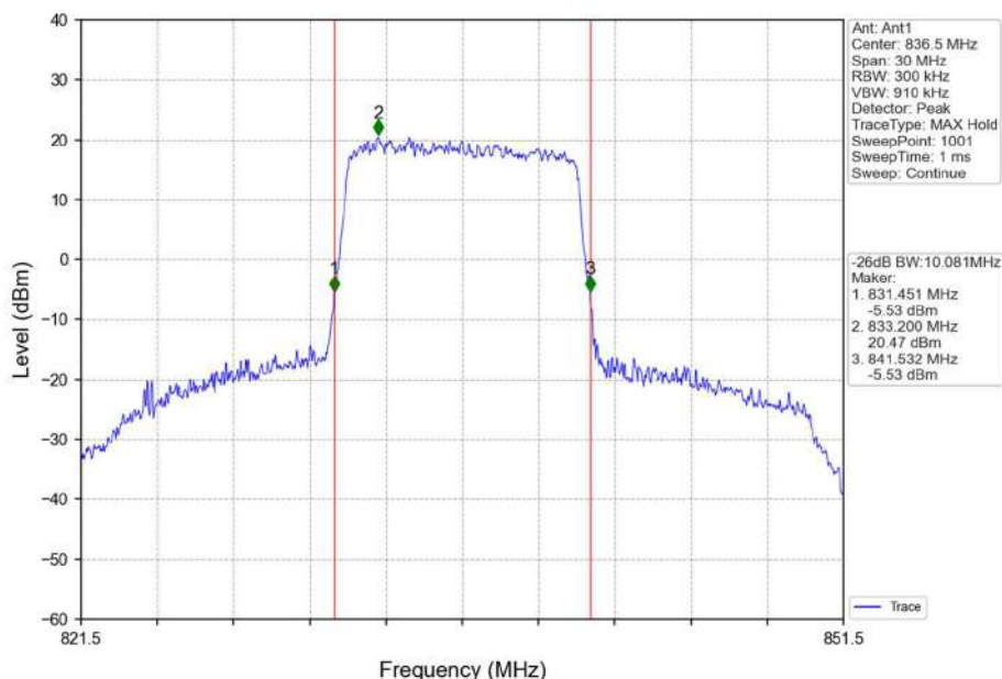
Band5_10MHz_QPSK_MCH_836.5MHz_RB_50_0_NTNV
