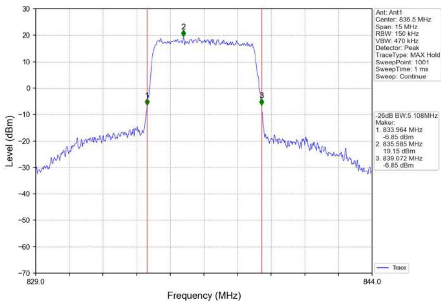
Band5_5MHz_16QAM_MCH_836.5MHz_RB_25_0_NTNV
