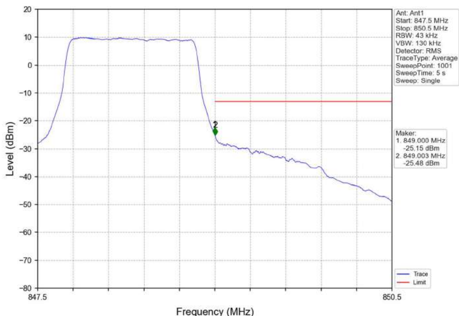
Band5_1.4MHz_16QAM_HCH_848.3MHz_RB_6_0_NTNV
