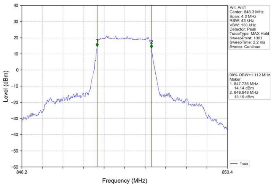
Band5_1.4MHz_QPSK_HCH_848.3MHz_RB_6_0_NTNV
