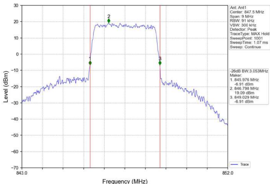
Band5_3MHz_16QAM_HCH_847.5MHz_RB_15_0_NTNV
