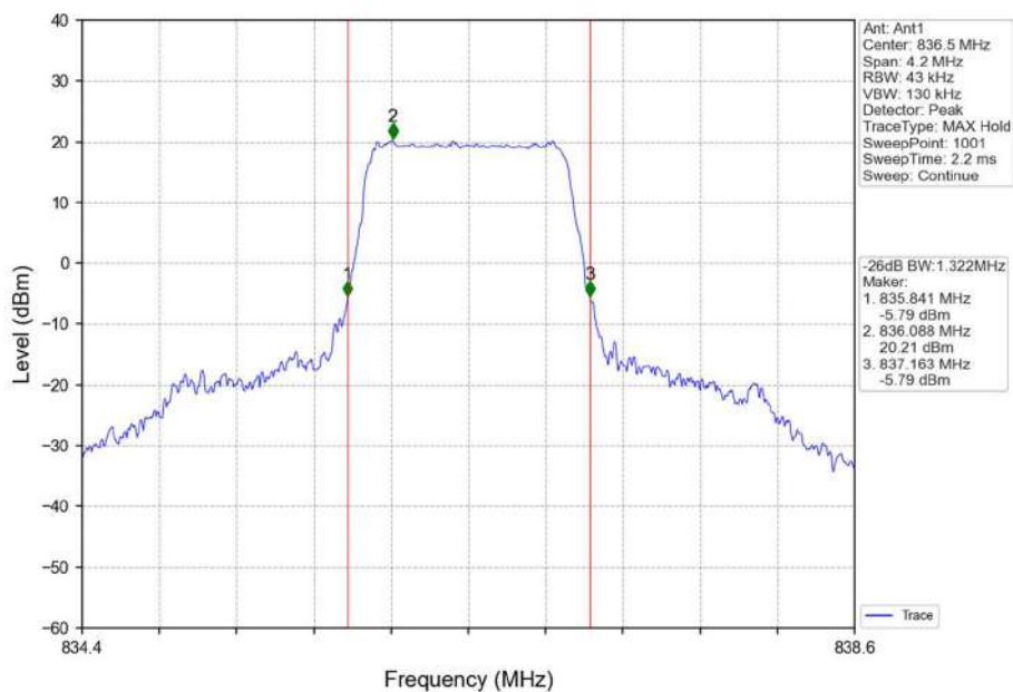
Band5_1.4MHz_QPSK_MCH_836.5MHz_RB_6_0_NTNV
