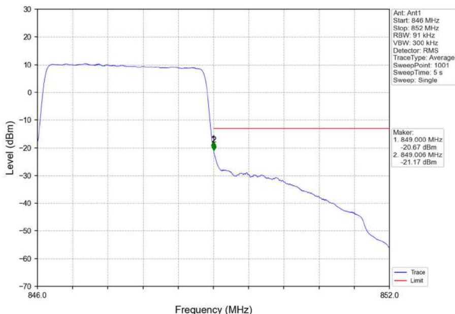
Band5_3MHz_QPSK_HCH_847.5MHz_RB_15_0_NTNV
