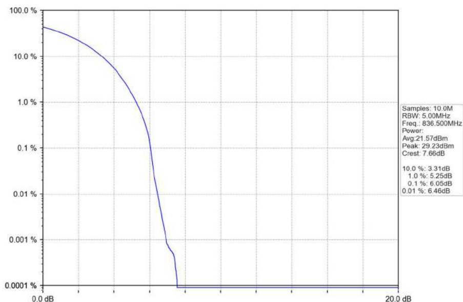
Band5_10MHz_QPSK_MCH_836.5MHz_RB_50_0_NTNV
