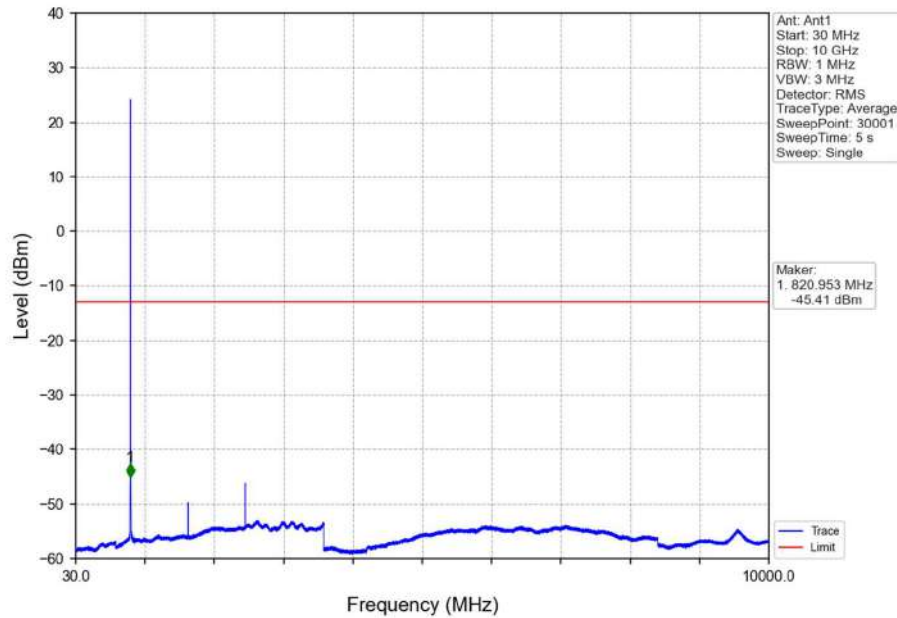
Band5_1.4MHz_16QAM_LCH_824.7MHz_RB_1_0_NTNV
