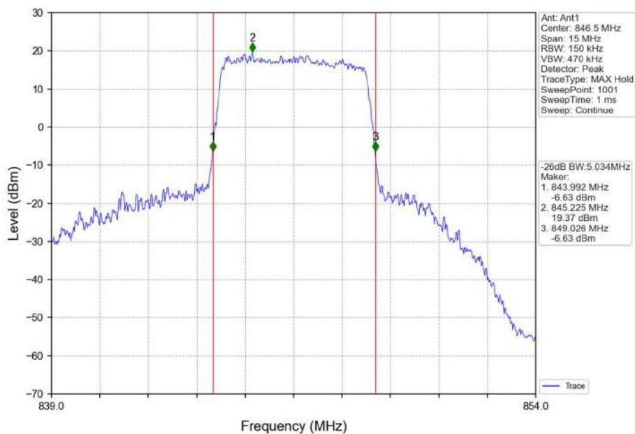
Band5_5MHz_16QAM_HCH_846.5MHz_RB_25_0_NTNV
