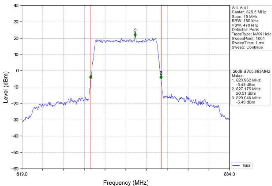
Band5_5MHz_QPSK_LCH_826.5MHz_RB_25_0_NTNV
