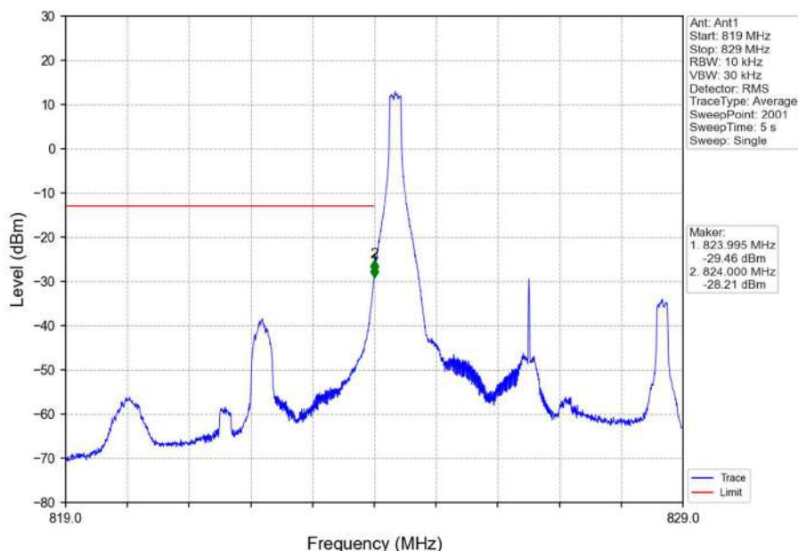
Band5_5MHz_16QAM_LCH_826.5MHz_RB_1_0_NTNV
