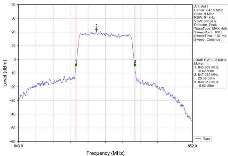
Band5_3MHz_QPSK_HCH_847.5MHz_RB_15_0_NTNV
