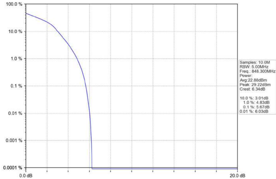
Band5_1.4MHz_16QAM_HCH_848.3MHz_RB_6_0_NTNV
