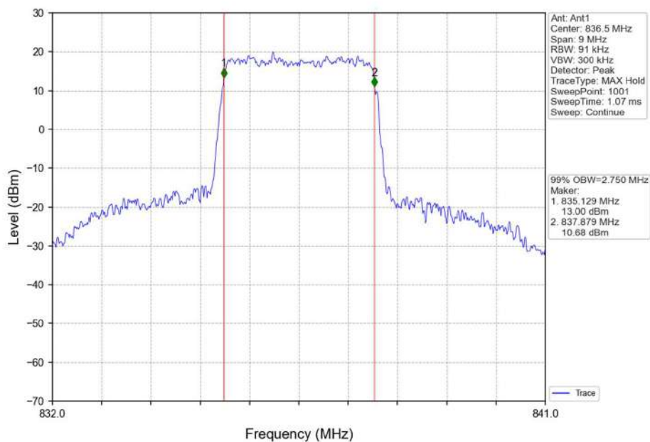
Band5_3MHz_16QAM_MCH_836.5MHz_RB_15_0_NTNV
