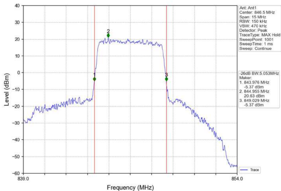
Band5_5MHz_QPSK_HCH_846.5MHz_RB_25_0_NTNV
