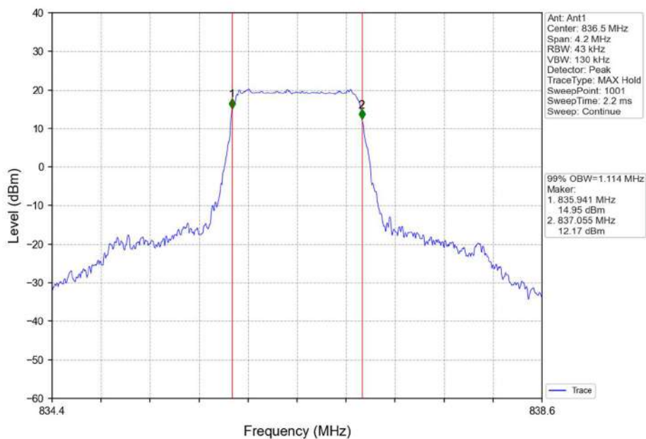
Band5_1.4MHz_QPSK_MCH_836.5MHz_RB_6_0_NTNV
