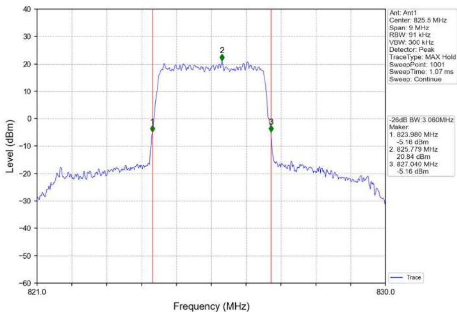
Band5_3MHz_QPSK_LCH_825.5MHz_RB_15_0_NTNV
