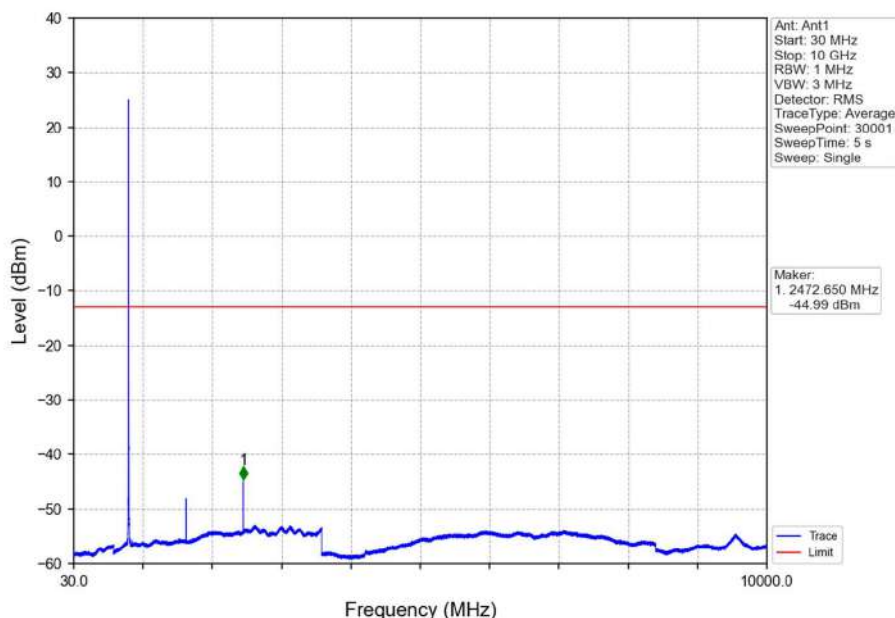
Band5_3MHz_QPSK_LCH_825.5MHz_RB_1_0_NTNV
