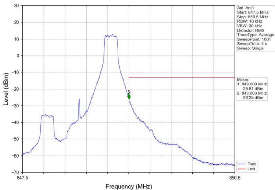
Band5_1.4MHz_16QAM_HCH_848.3MHz_RB_1_5_NTNV
