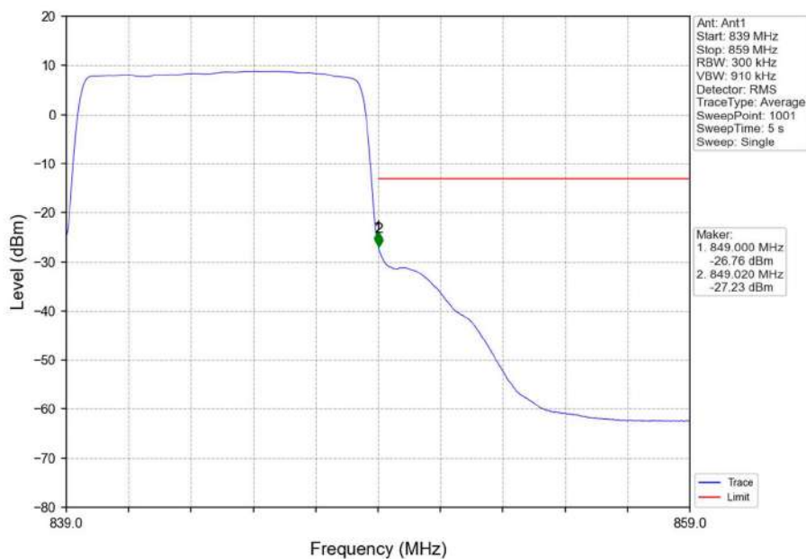
Band5_10MHz_16QAM_HCH_844MHz_RB_50_0_NTNV
