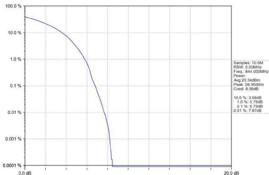
Band5_10MHz_16QAM_HCH_844MHz_RB_50_0_NTNV
