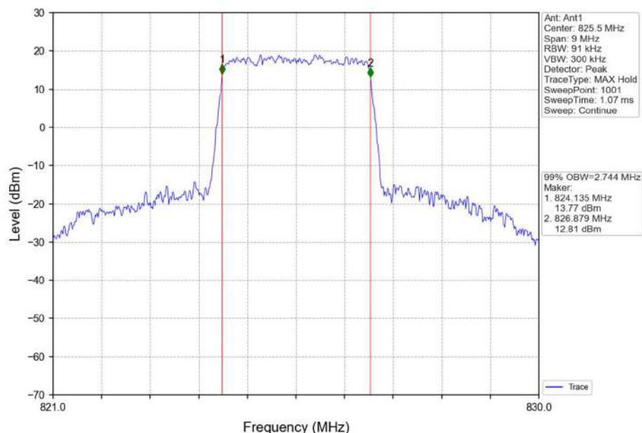
Band5_3MHz_16QAM_LCH_825.5MHz_RB_15_0_NTNV
