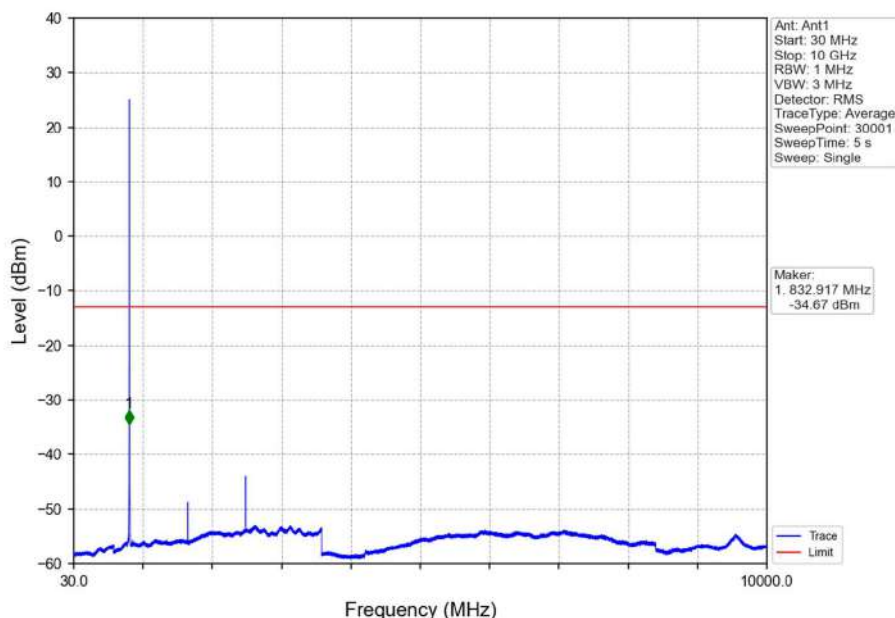
Band5_1.4MHz_QPSK_MCH_836.5MHz_RB_1_0_NTNV
