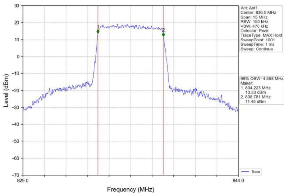
Band5_5MHz_16QAM_MCH_836.5MHz_RB_25_0_NTNV
