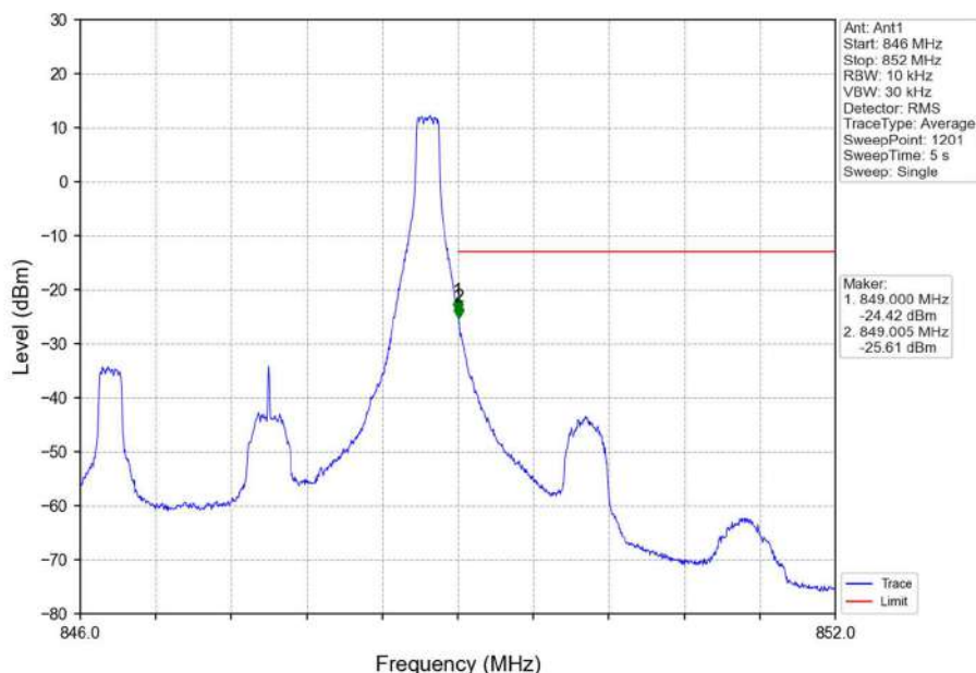
Band5_3MHz_16QAM_HCH_847.5MHz_RB_1_14_NTNV
