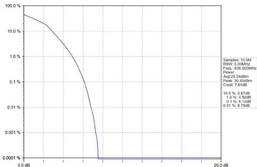
Band5_5MHz_16QAM_MCH_836.5MHz_RB_25_0_NTNV
