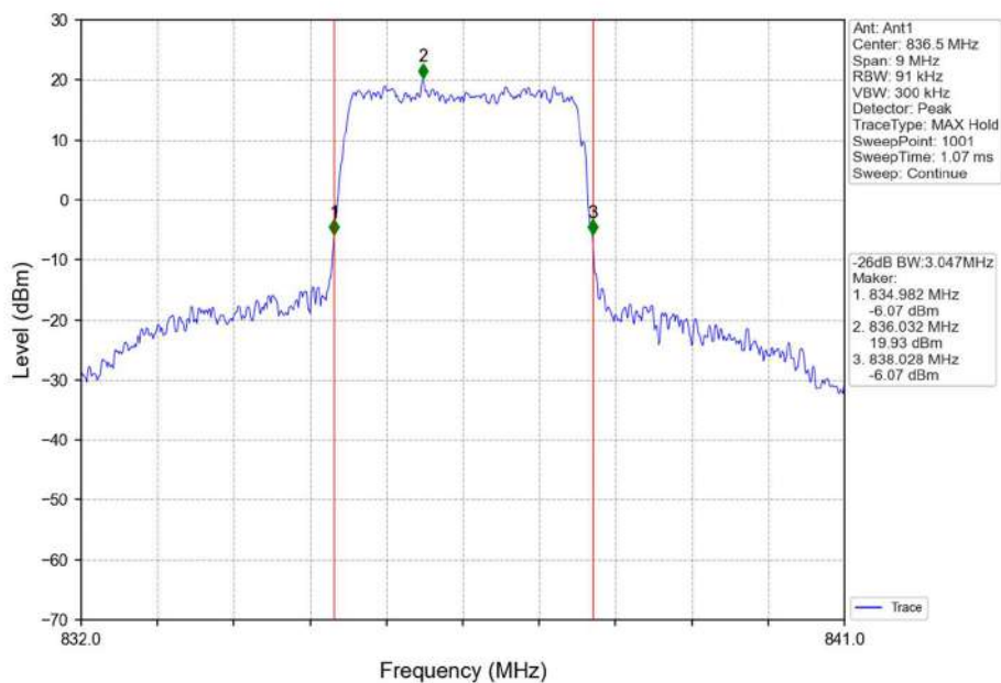
Band5_3MHz_16QAM_MCH_836.5MHz_RB_15_0_NTNV
