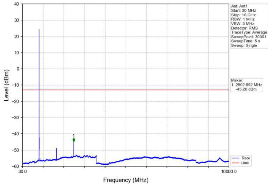
Band5_5MHz_16QAM_MCH_836.5MHz_RB_1_0_NTNV
