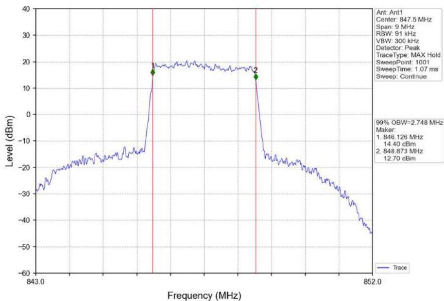
Band5_3MHz_QPSK_HCH_847.5MHz_RB_15_0_NTNV
