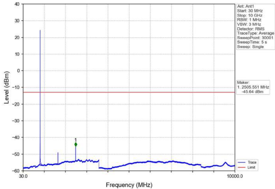
Band5_3MHz_16QAM_MCH_836.5MHz_RB_1_0_NTNV
