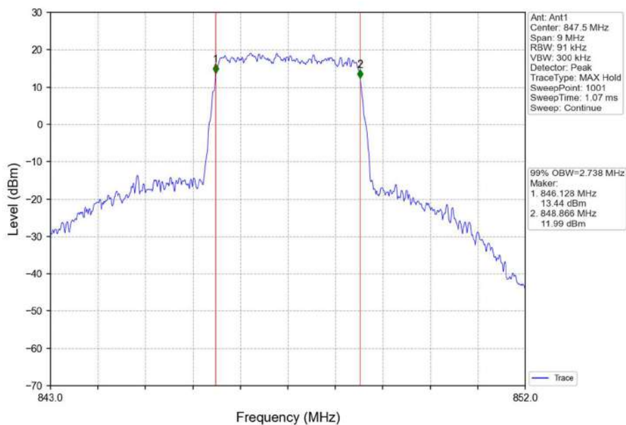
Band5_3MHz_16QAM_HCH_847.5MHz_RB_15_0_NTNV
