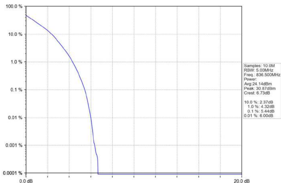
Band5_5MHz_QPSK_MCH_836.5MHz_RB_25_0_NTNV
