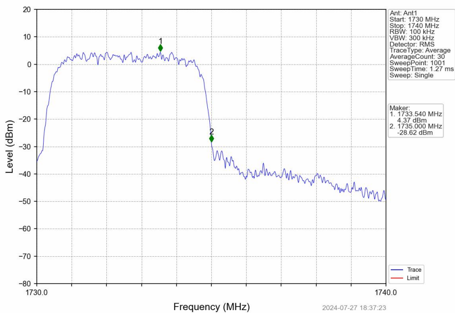
Band4_HSUPA_MCH_1732.6MHz_Subtest 1_NTNV
