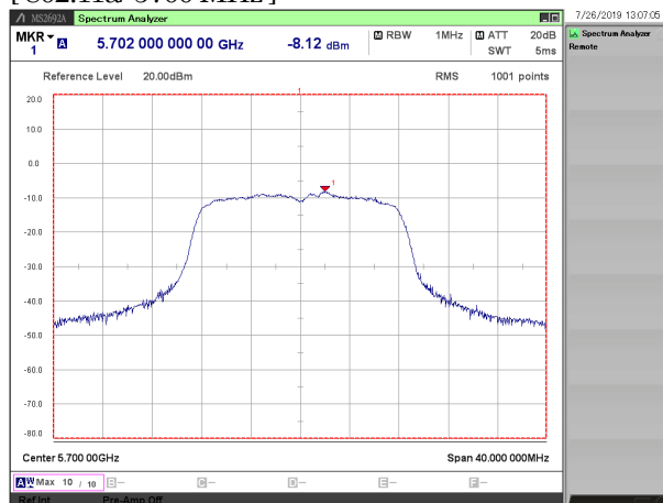
[ 802.11a/ 5700 MHz ]
