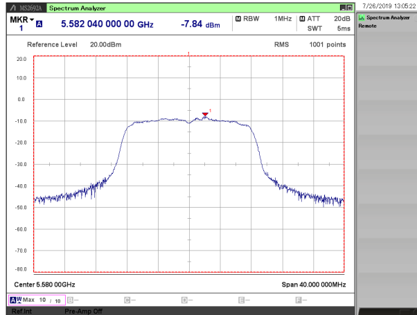
[ 802.11a/ 5580 MHz ]
