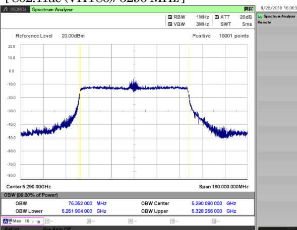
[ 802.11ac (VHT80)/ 5290 MHz ]
