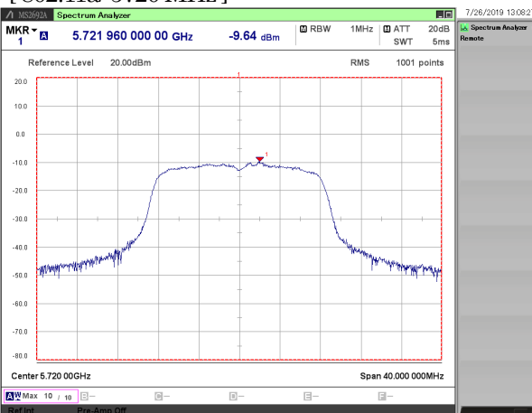
[ 802.11a/ 5720 MHz ]
