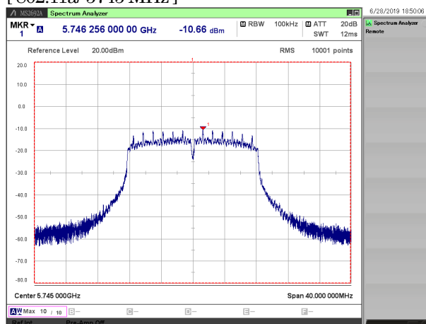
[ 802.11a/ 5745 MHz ]
