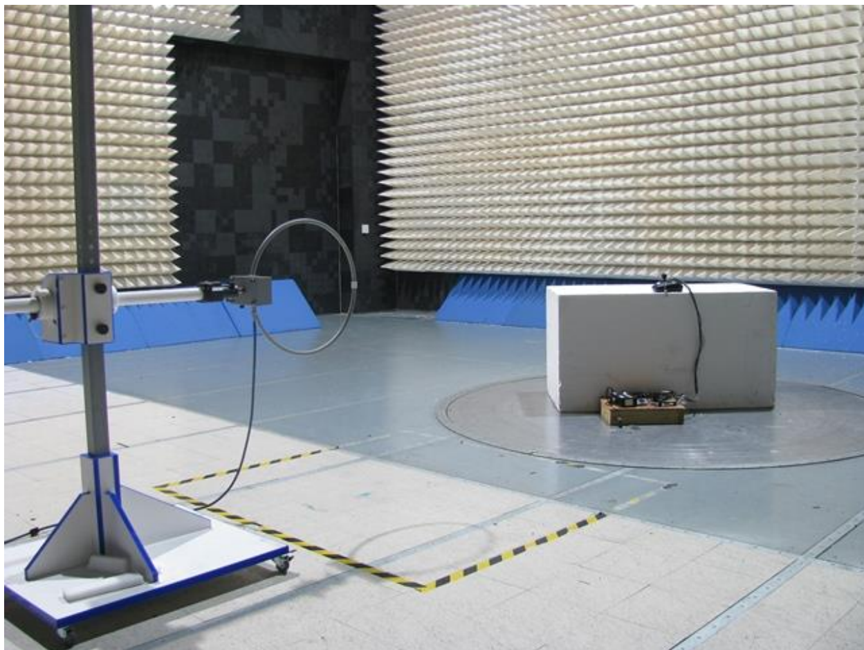
Radiated Emissions – Loop
