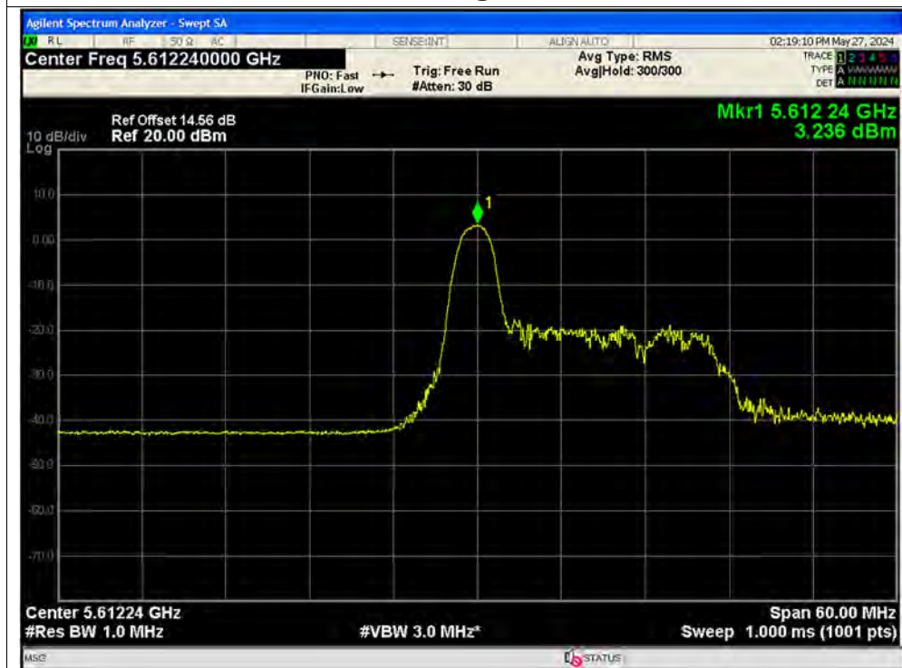
PSD NVNT ax40 26@0 5630MHz Ant2
