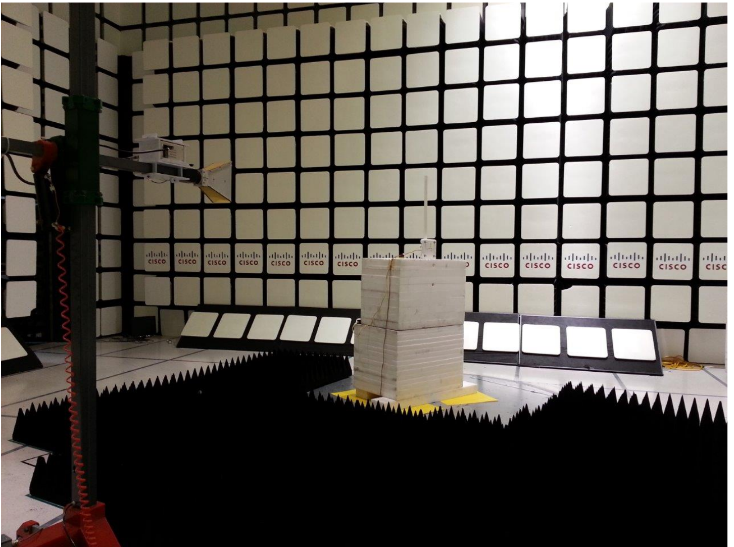
Radiated Test Setup 1GHz-18GHz
