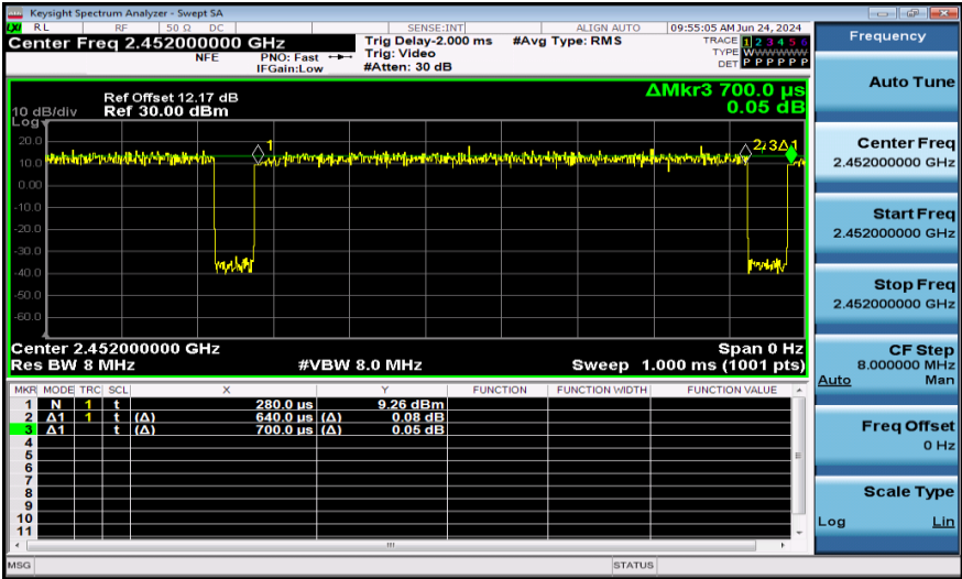
NTNV-11N40MIMO-Ant1-2452
