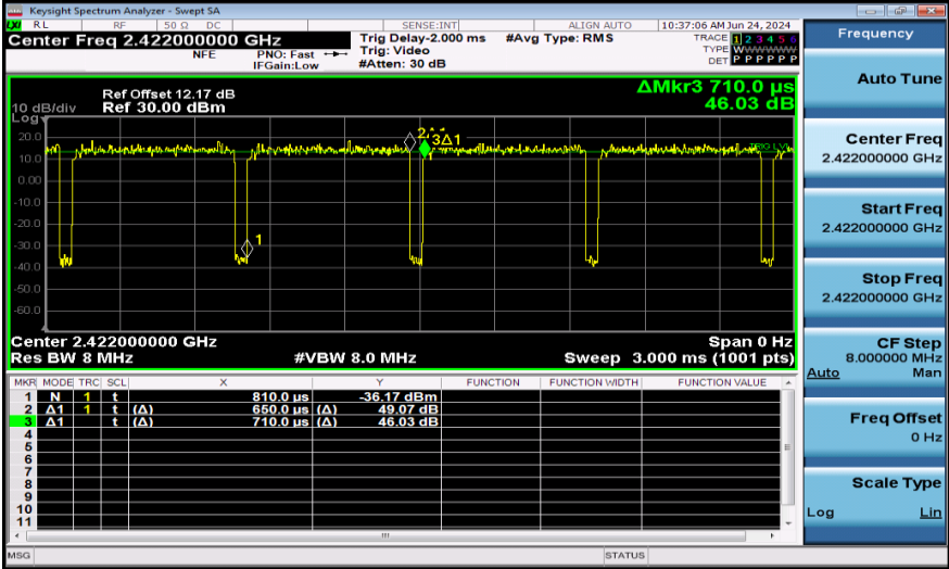
NTNV-11N40MIMO-Ant1-2422
