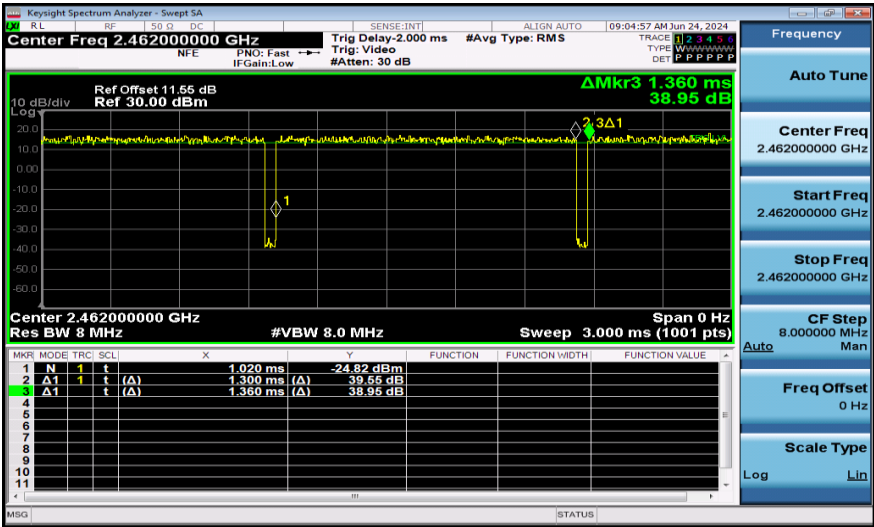
NTNV-11N20MIMO-Ant2-2462
