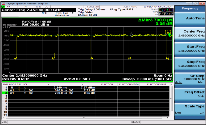
NTNV-11N40MIMO-Ant2-2452
