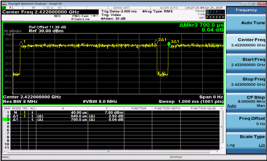
NTNV-11N40MIMO-Ant2-2422
