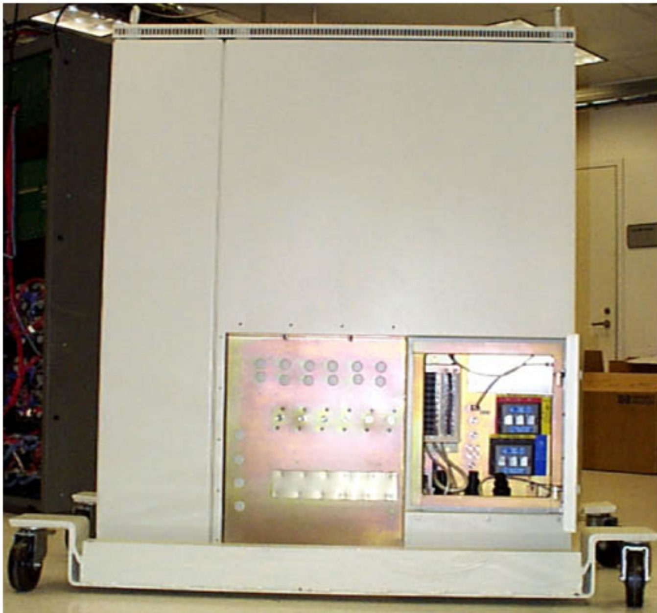
IHET5BQ1 SC4812ET @ 800 MHz Rear View without Panel
