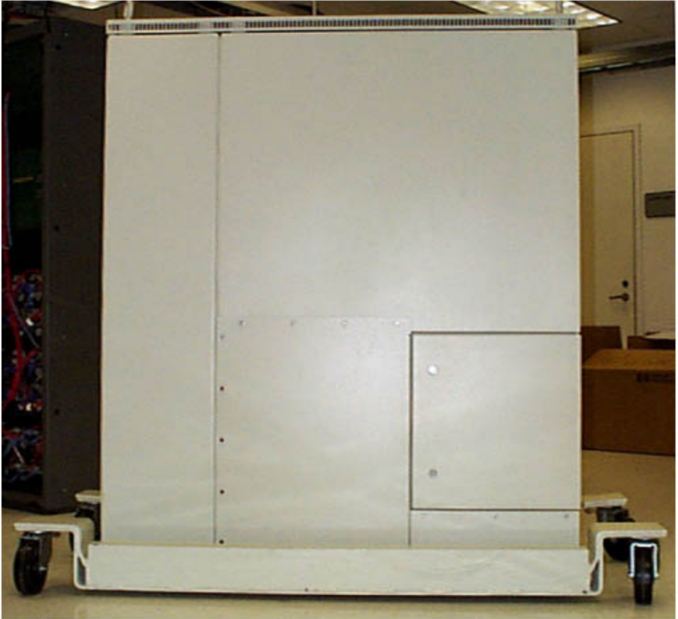
IHET5BQ1 SC4812ET @ 800 MHz Rear View with Panel
