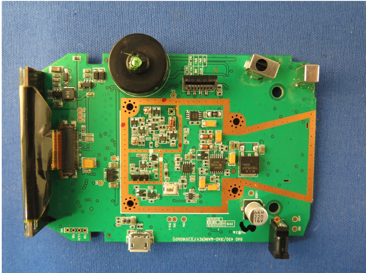
TOP PCB – HORN REMOVED
