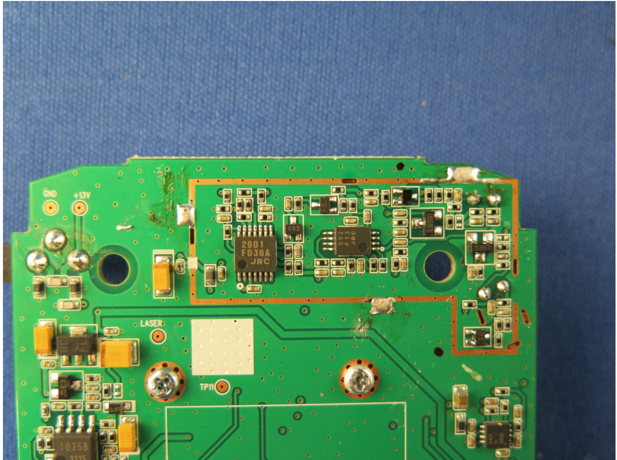
CLOSE UP SHIELD REMOVED
