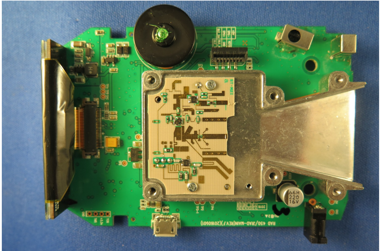
TOP PCB HORN TOP REMOVED
