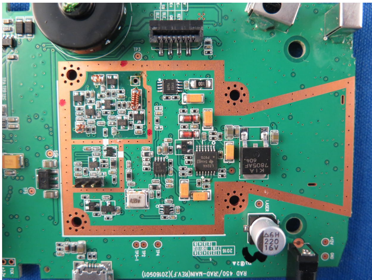
CLOSE UP PCB HORN REMOVED
