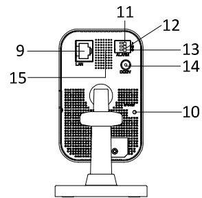
Figure 1-5 Rear View of Type II Cube Camera
