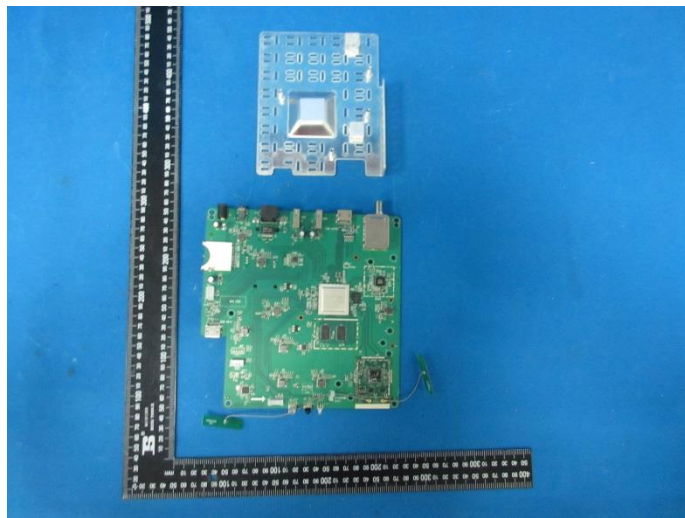
tuner receiver
