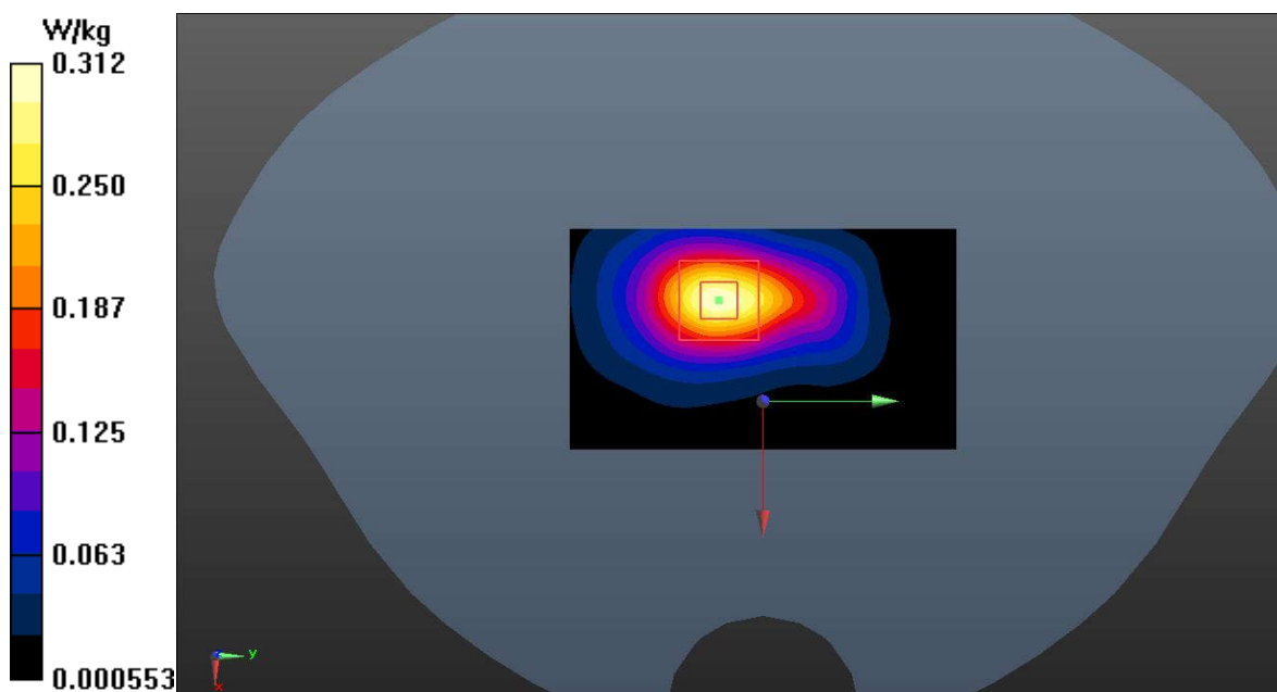
Fig.74 WLAN 2.4GHz Body
