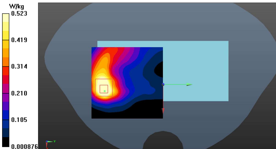
Fig.26 LTE Band 7 Body
