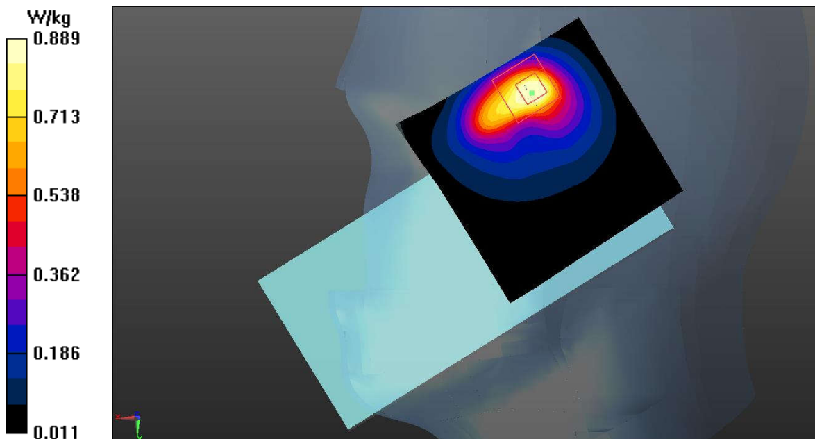
Fig.1 GSM850 Head
