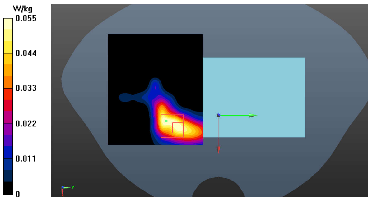
Fig.71 Bluetooth Body
