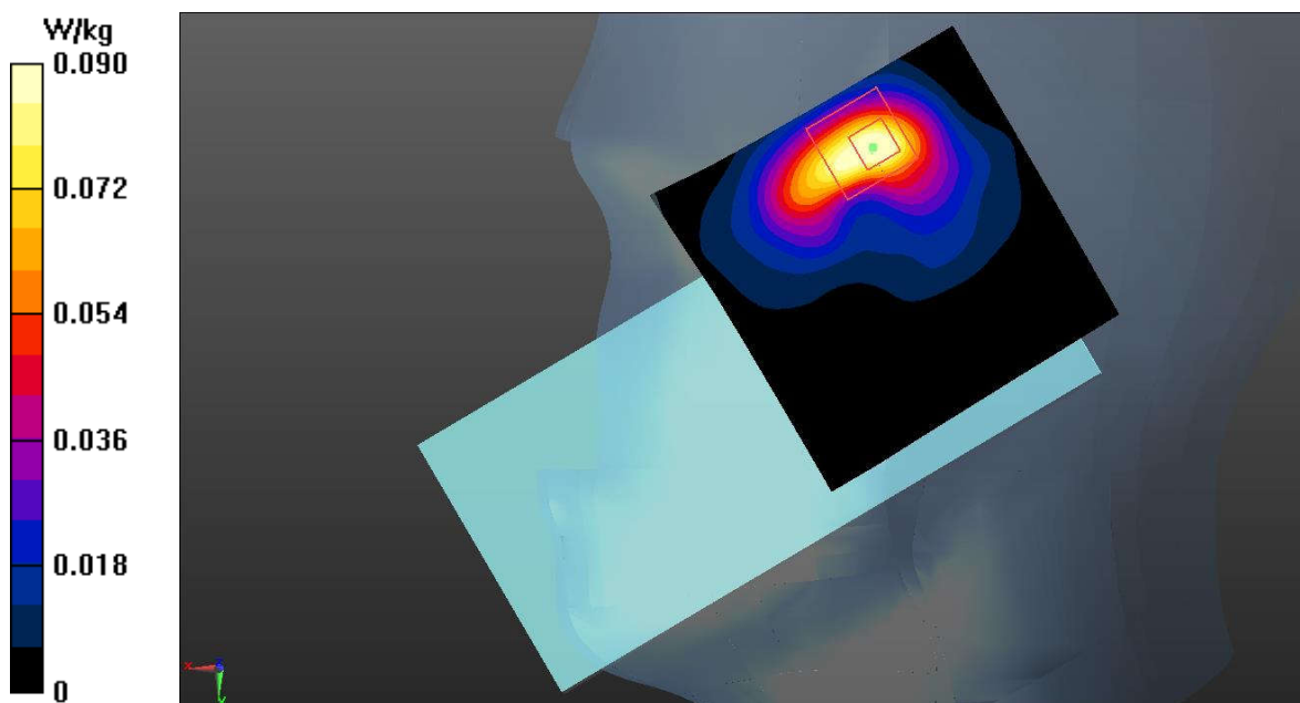
Fig.55 NR n12 Head
