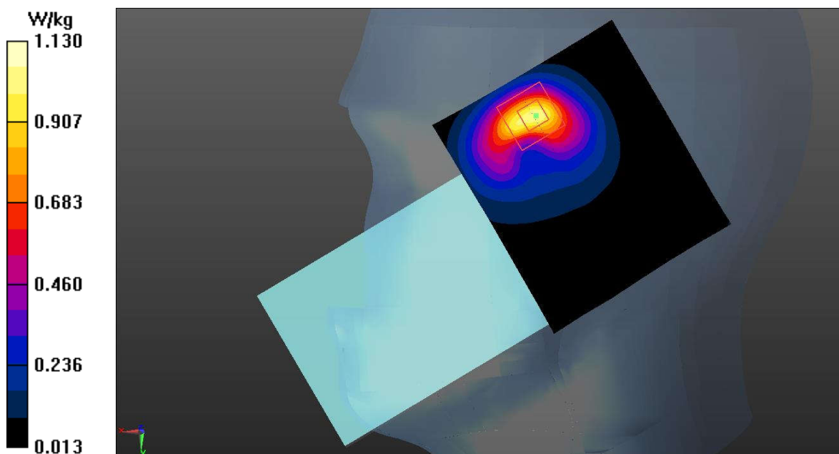
Fig.13 WCDMA Band 5 Head
