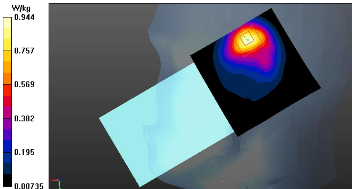
Fig.7 WCDMA Band 2 Head
