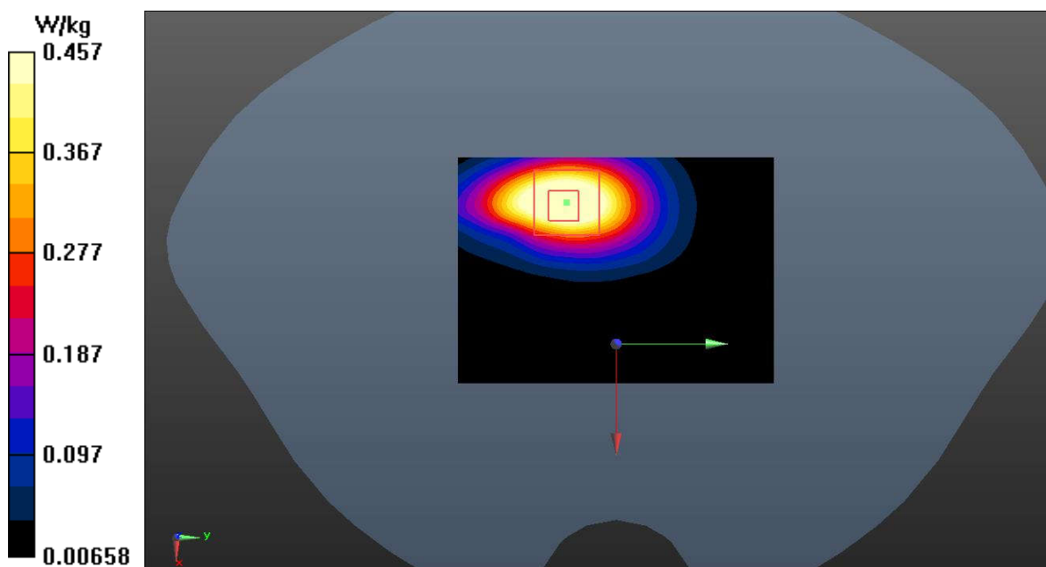
Fig.6 GSM1900 Body
