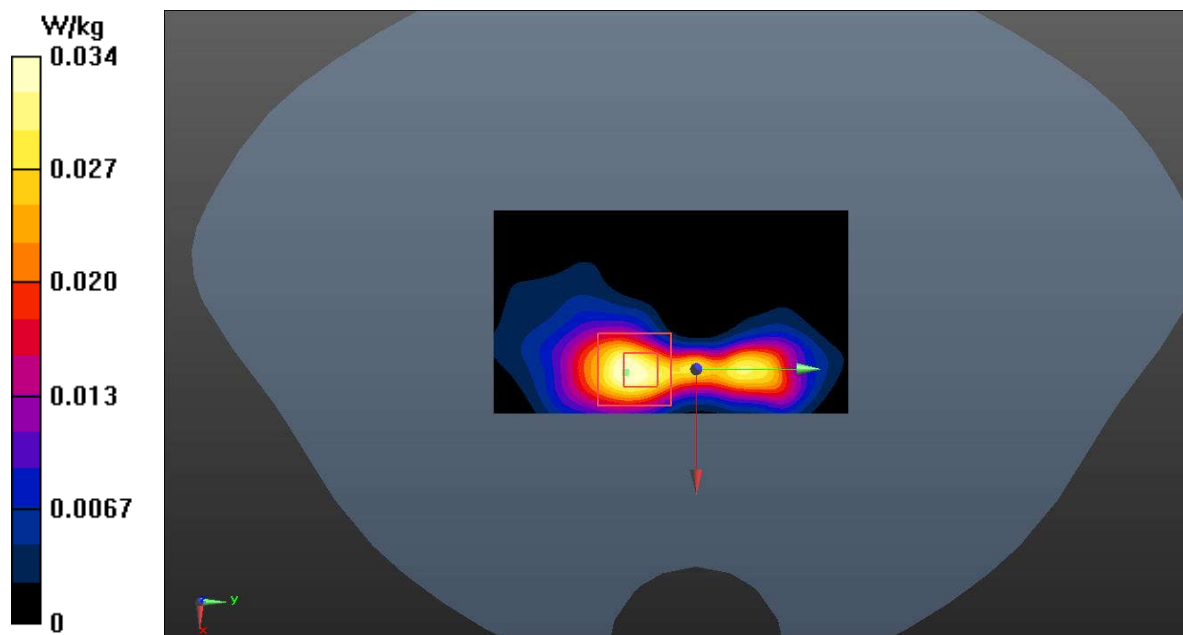
Fig.72 Bluetooth Body
