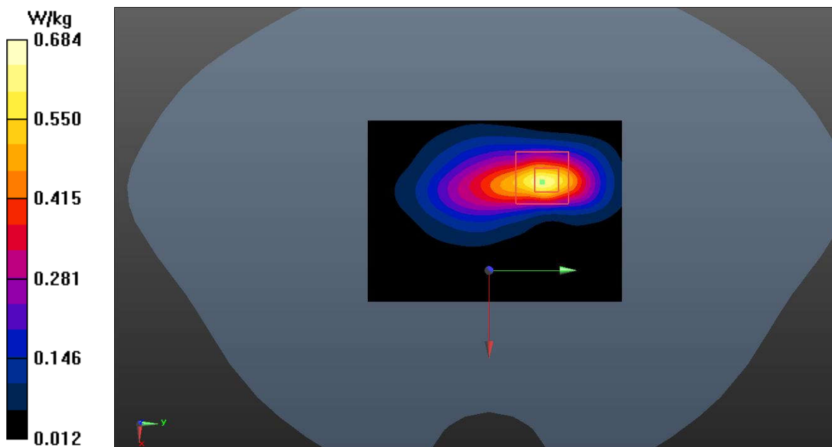
Fig.9 WCDMA Band 2 Body
