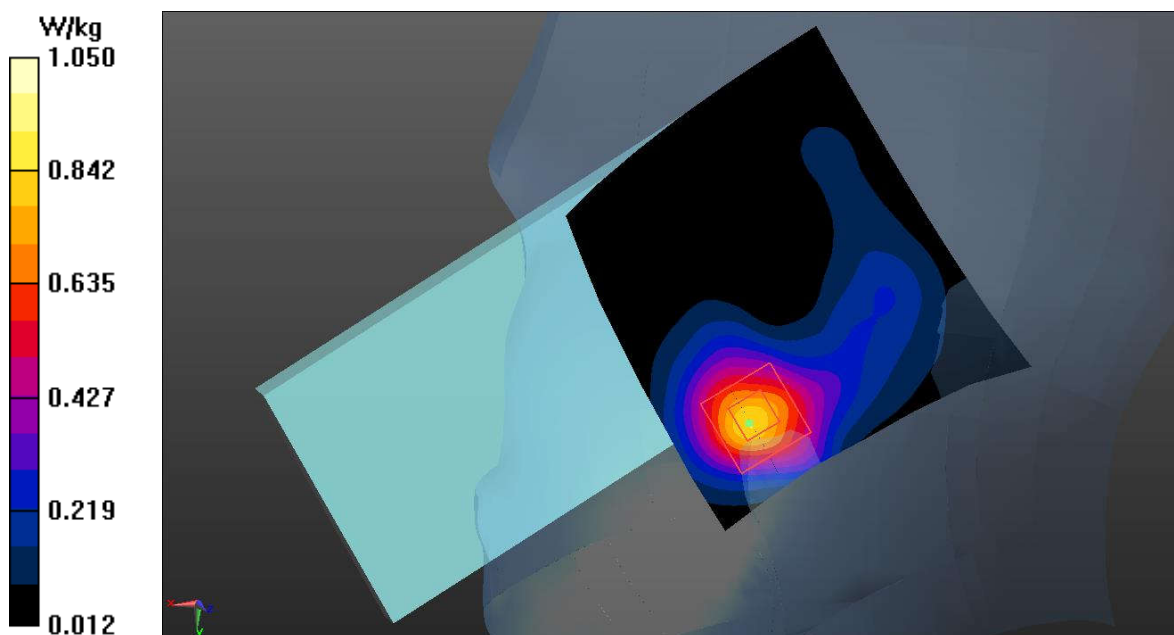
Fig.40 LTE Band 41 Head
