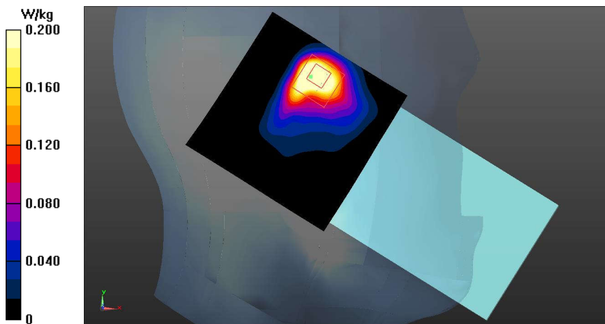
Fig.70 Bluetooth Head
