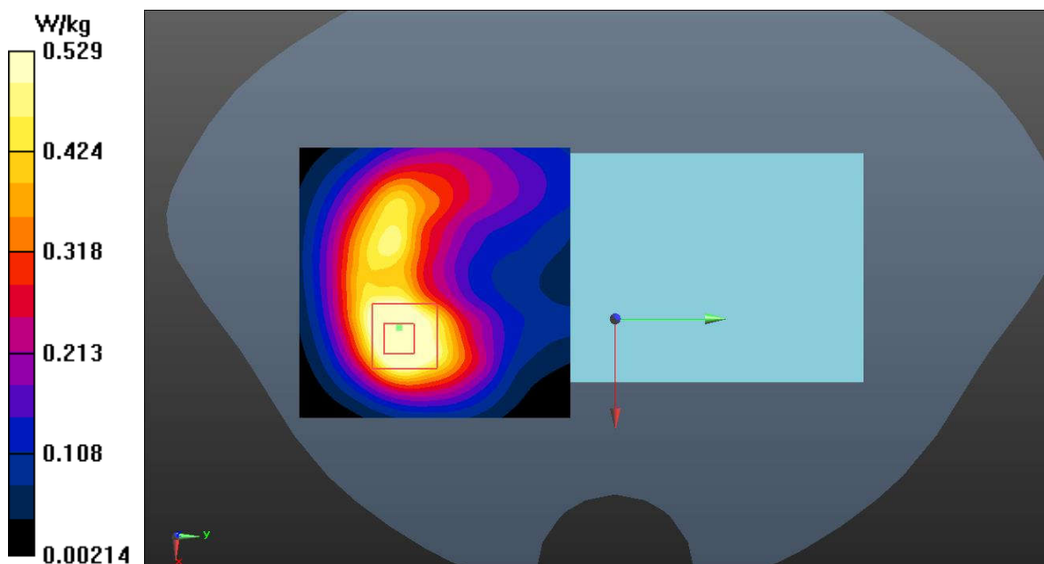
Fig.38 LTE Band 38 Body
