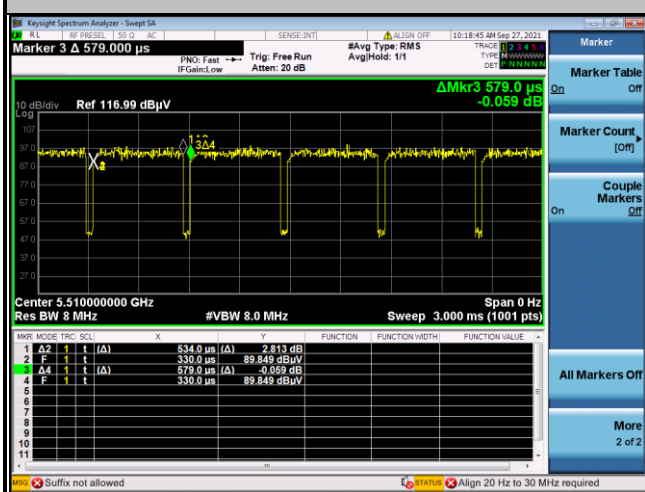
5GHz 802.11ax HE80 Full RU
