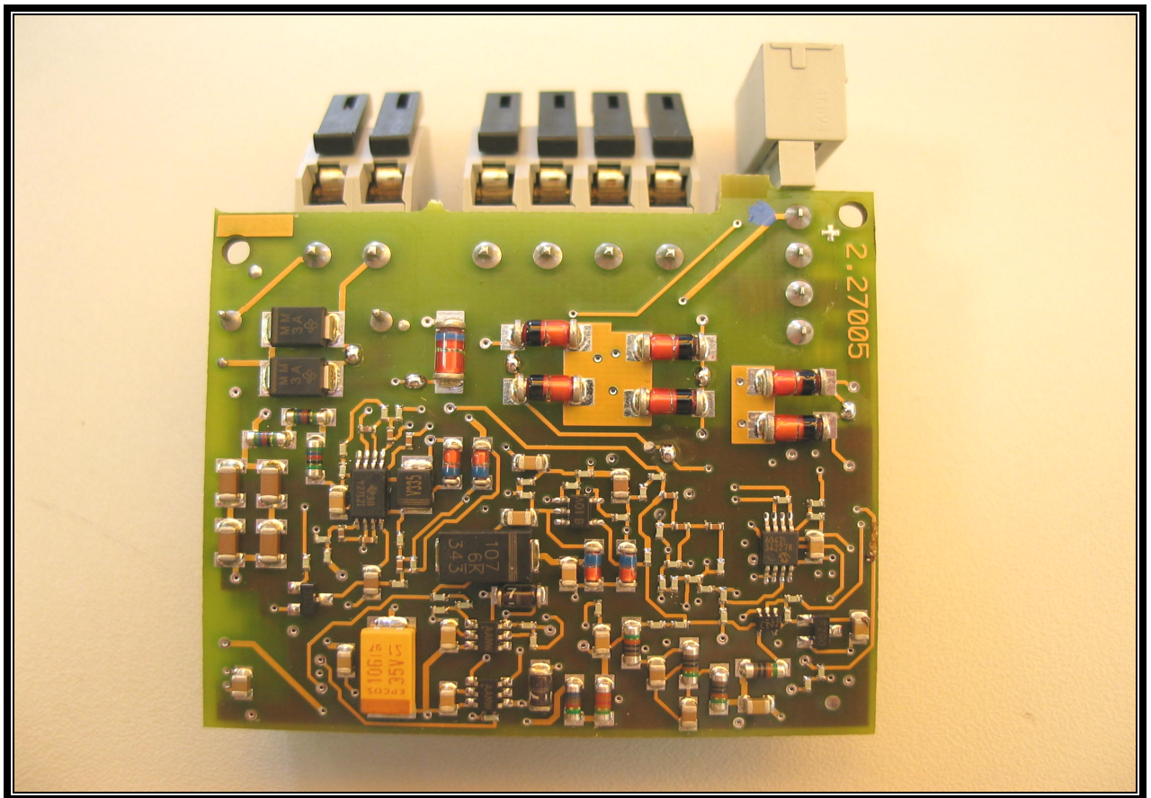
PHOTOGRAPH 31: EUT POWER MODULE PCB1 BOTTOM VIEW
