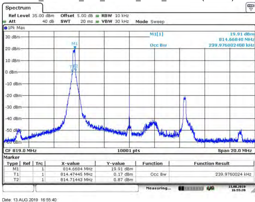
B26_CH26740_10M_16-QAM_1RB0_99% BW (Part 90)
