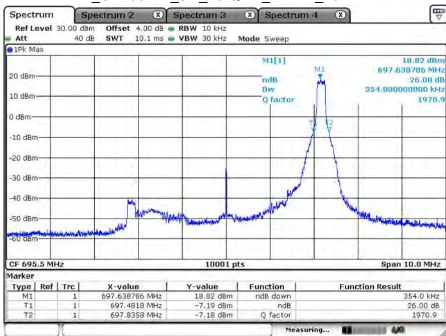
B71_CH133447_5M_16-QAM_1RB24_26dB BW
