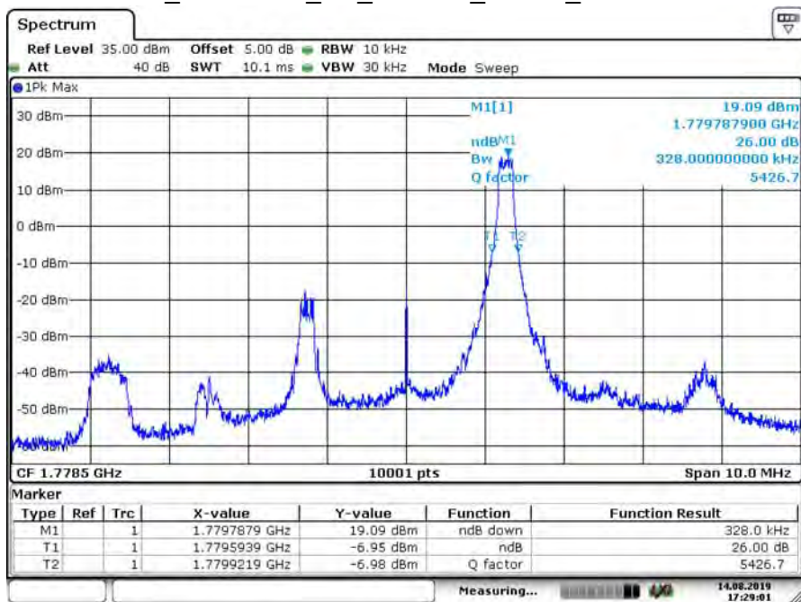
B66_CH132657_3M_16-QAM_1RB14_26dB BW
