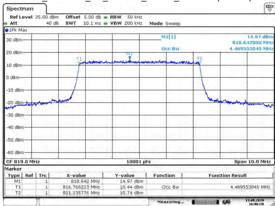
B26_CH26740_5M_16-QAM_25RB0_99% BW (Part 90)
