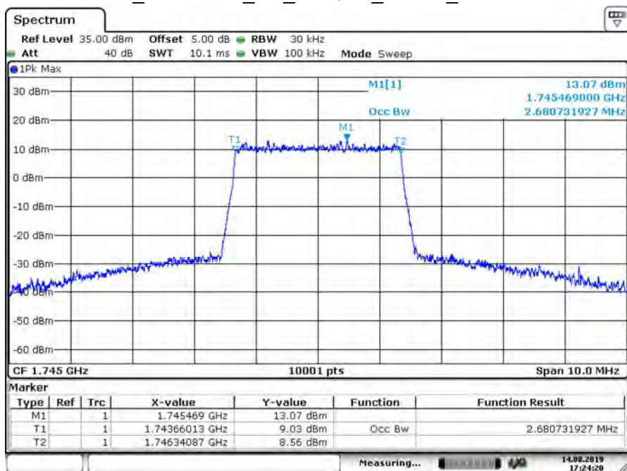
B66_CH132322_3M_16-QAM_15RB0_99% BW
