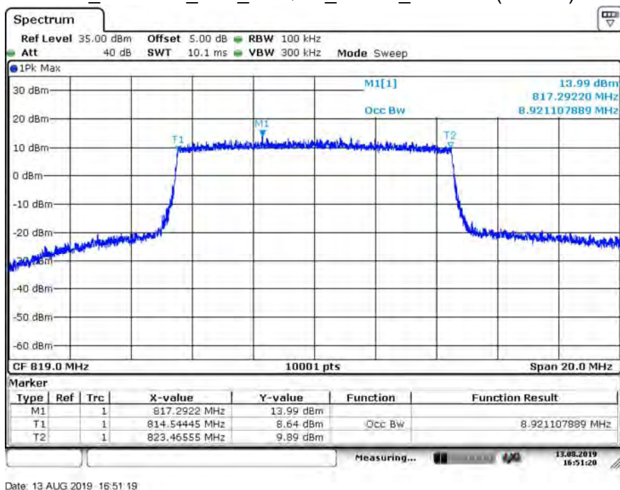
B26_CH26740_10M_16-QAM_50RB0_99% BW (Part 90)
