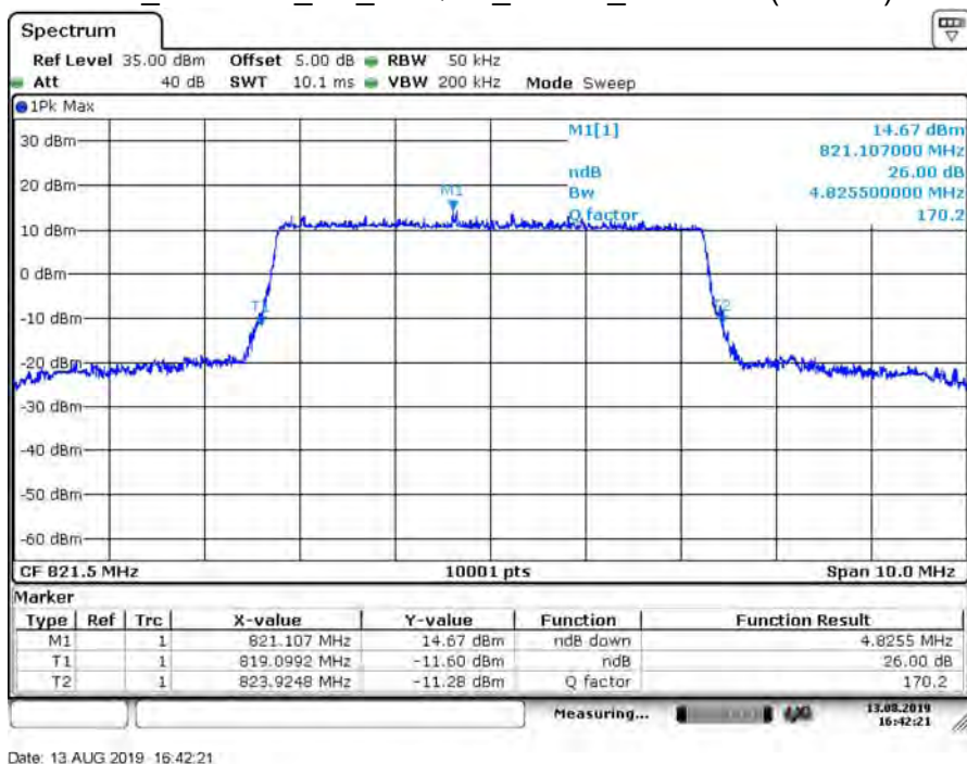
B26_CH26765_5M_16-QAM_25RB0_26dB BW (Part 90)
