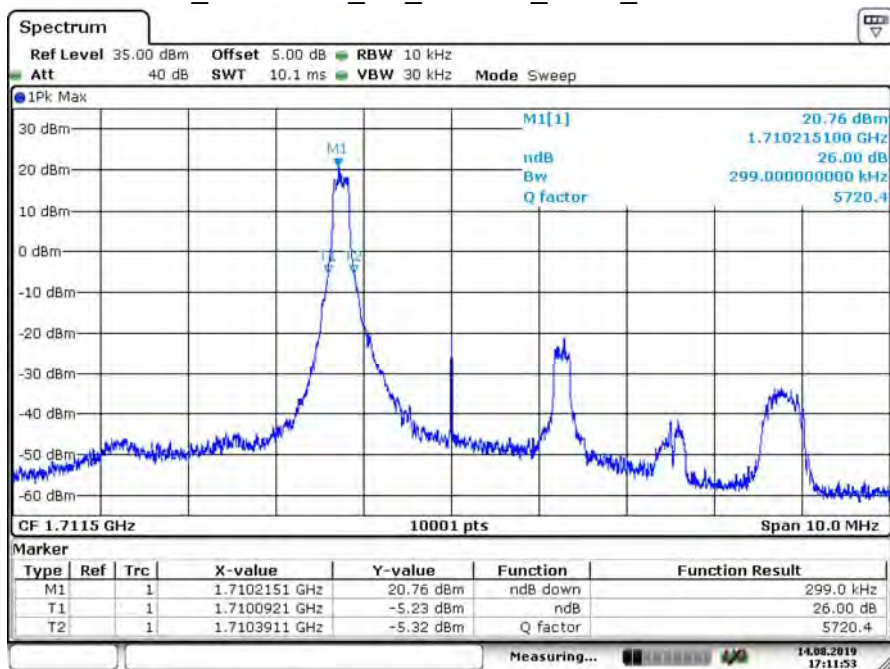
B66_CH131987_3M_16-QAM_1RB0_26dB BW
