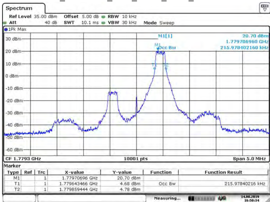
B66_CH132665_1.4M_QPSK_1RB5_99% BW
