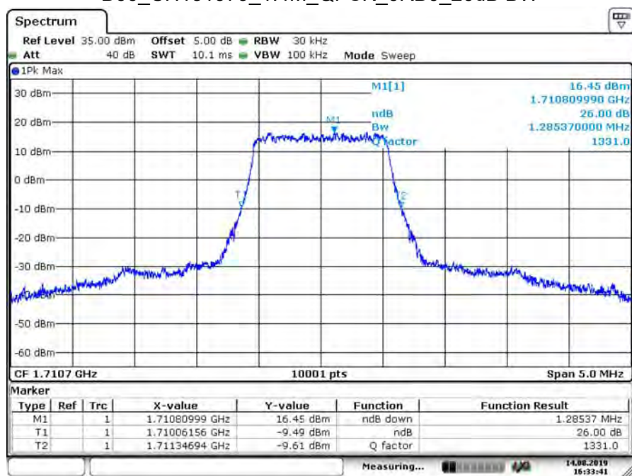
B66_CH131979_1.4M_QPSK_6RB0_26dB BW
