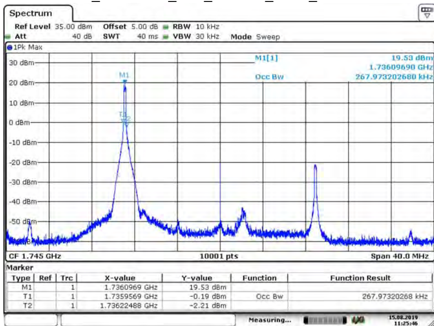
B66_CH132322_20M_16-QAM_1RB0_99% BW
