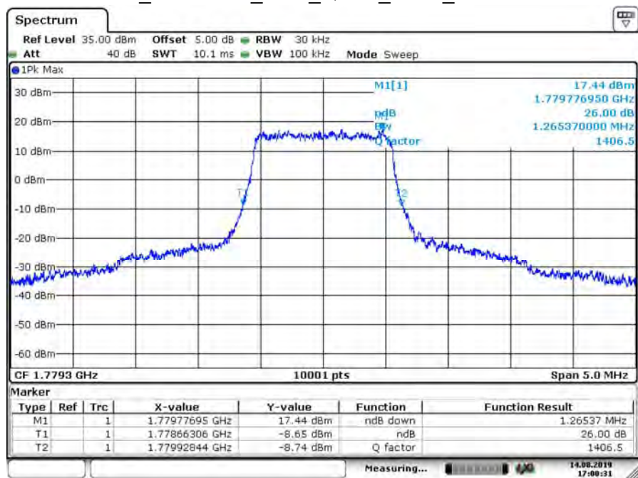
B66_CH132665_1.4M_QPSK_6RB0_26dB BW
