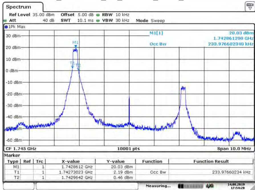
B66_CH132322_5M_16-QAM_1RB0_99% BW
