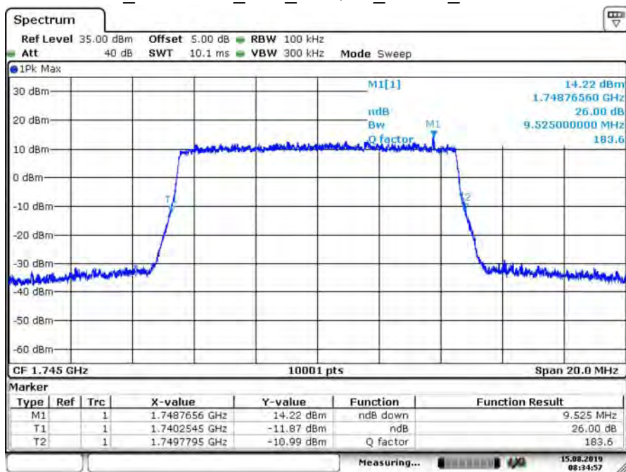
B66_CH132322_10M_16-QAM_50RB0_26dB BW
