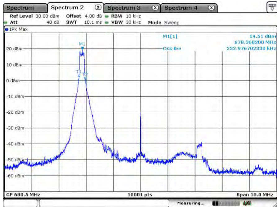
B71_CH133297_5M_16-QAM_1RB0_99% BW
