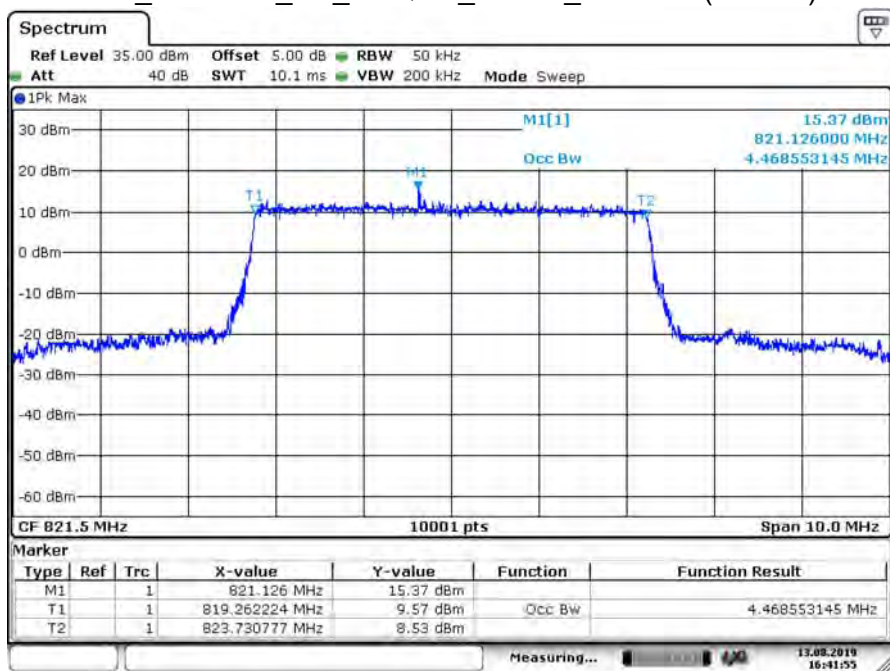
B26_CH26765_5M_16-QAM_25RB0_99% BW (Part 90)
