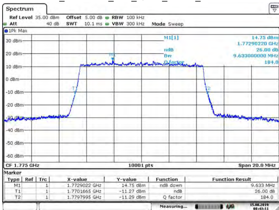
B66_CH132622_10M_QPSK_50RB0_26dB BW
