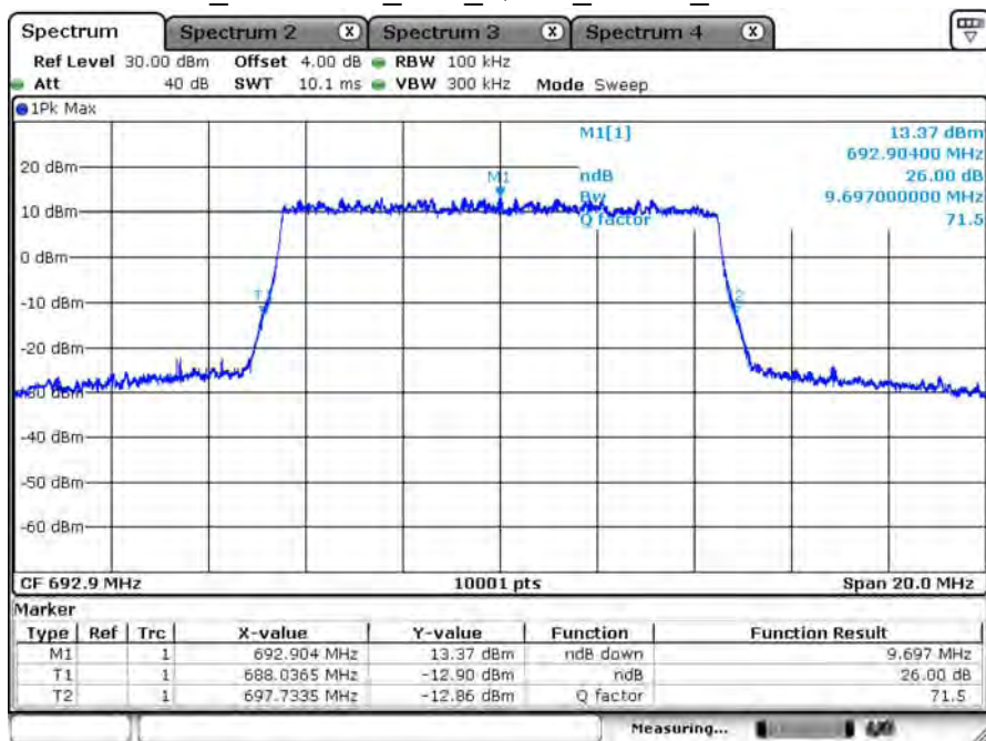
B71_CH133421_10M_QPSK_50RB0_26dB BW
