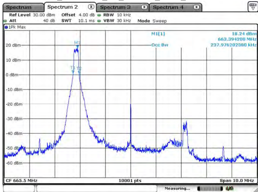
B71_CH133147_5M_16-QAM_1RB0_99% BW
