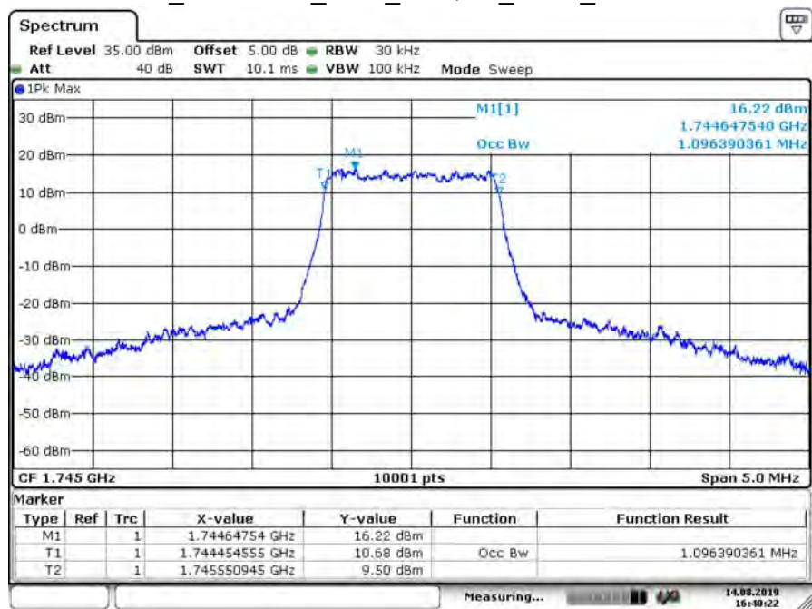
B66_CH132322_1.4M_16-QAM_6RB0_99% BW
