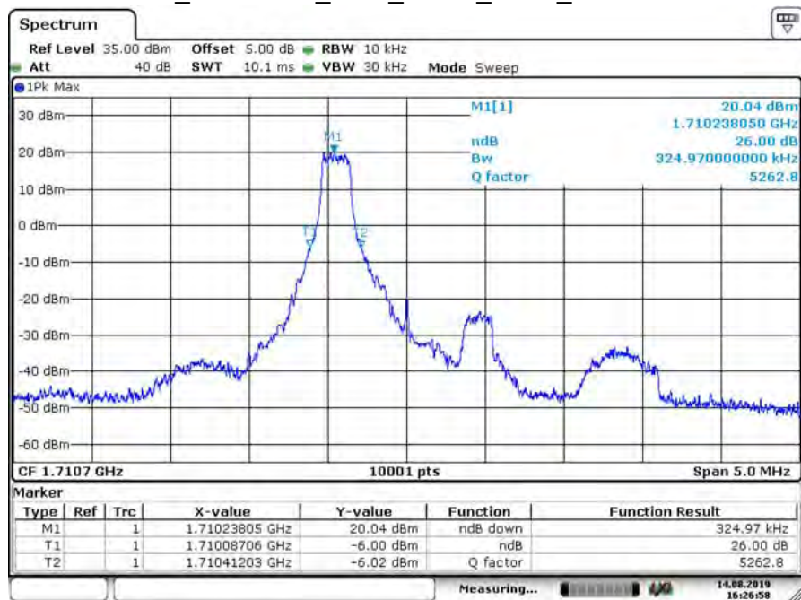
B66_CH131979_1.4M_QPSK_1RB0_26dB BW
