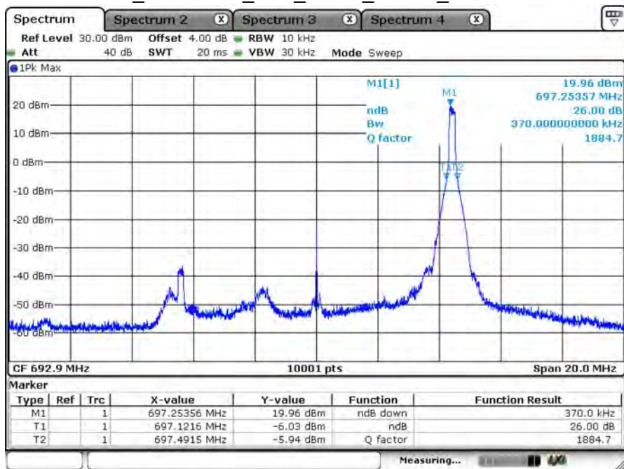
B71_CH133421_10M_QPSK_1RB49_26dB BW
