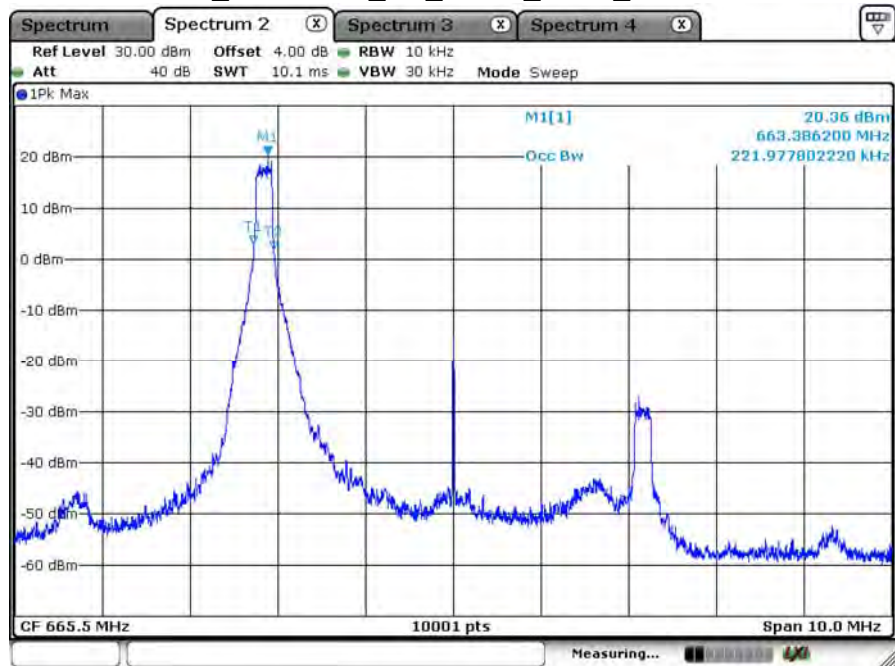
B71_CH133147_5M_QPSK_1RB0_99% BW
