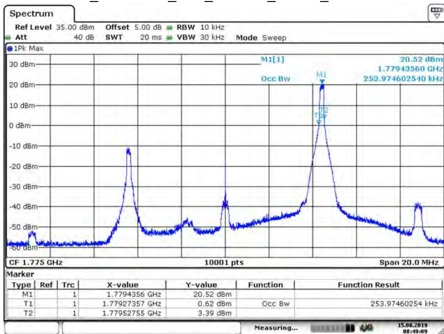
B66_CH132622_10M_16-QAM_1RB49_99% BW
