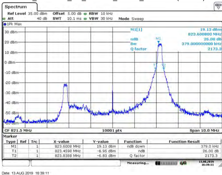
B26_CH26765_5M_16-QAM_1RB24_26dB BW (Part 90)
