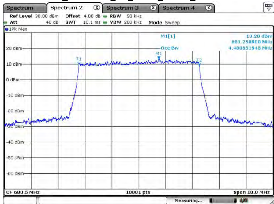
B71_CH133297_5M_QPSK_25RB0_99% BW
