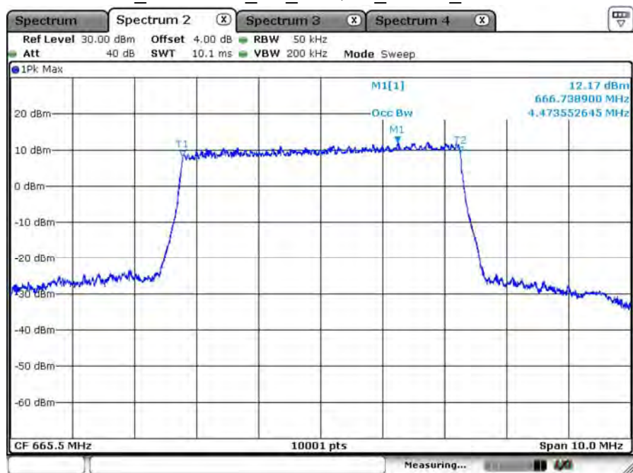
B71_CH133147_5M_16-QAM_25RB0_99% BW
