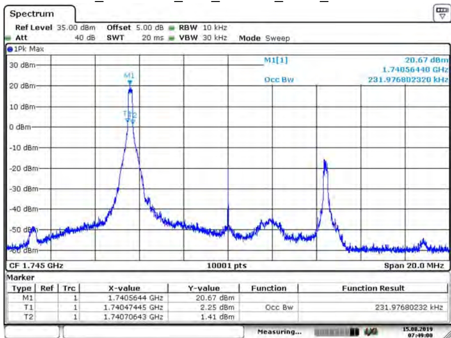
B66_CH132322_10M_16-QAM_1RB0_99% BW
