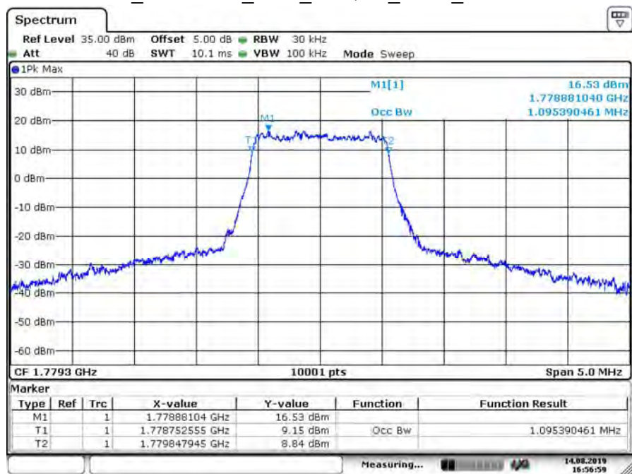
B66_CH132665_1.4M_16-QAM_6RB0_99% BW
