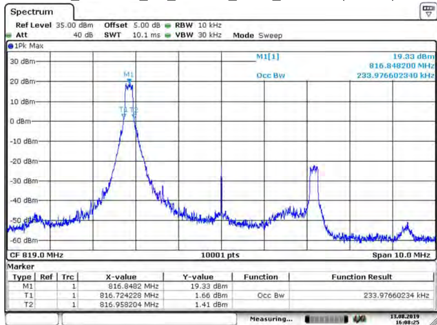
B26_CH26740_5M_16-QAM_1RB0_99% BW (Part 90)
