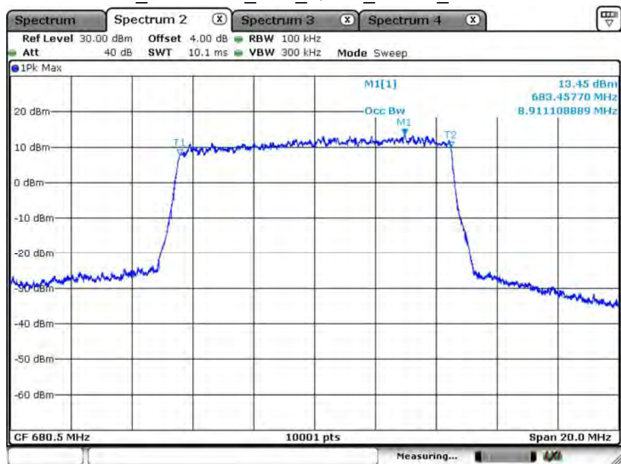
B71_CH133297_10M_QPSK_50RB0_99% BW
