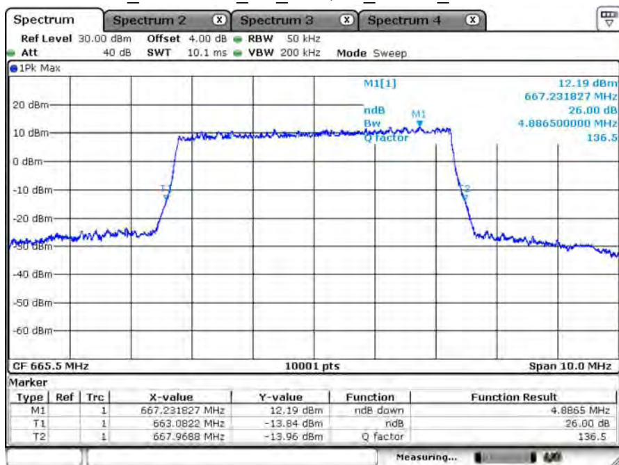
B71_CH133147_5M_16-QAM_25RB0_26dB BW
