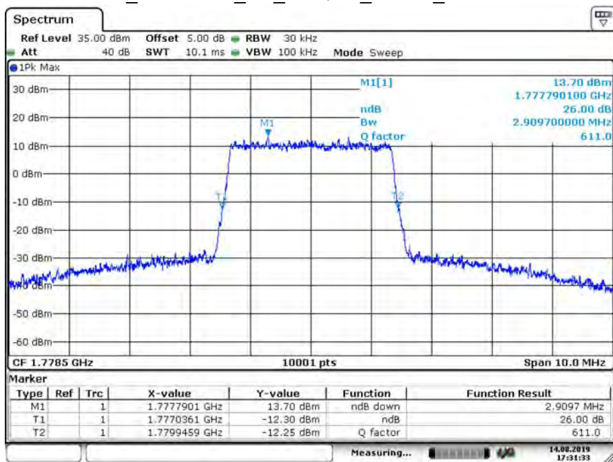
B66_CH132657_3M_16-QAM_15RB0_26dB BW
