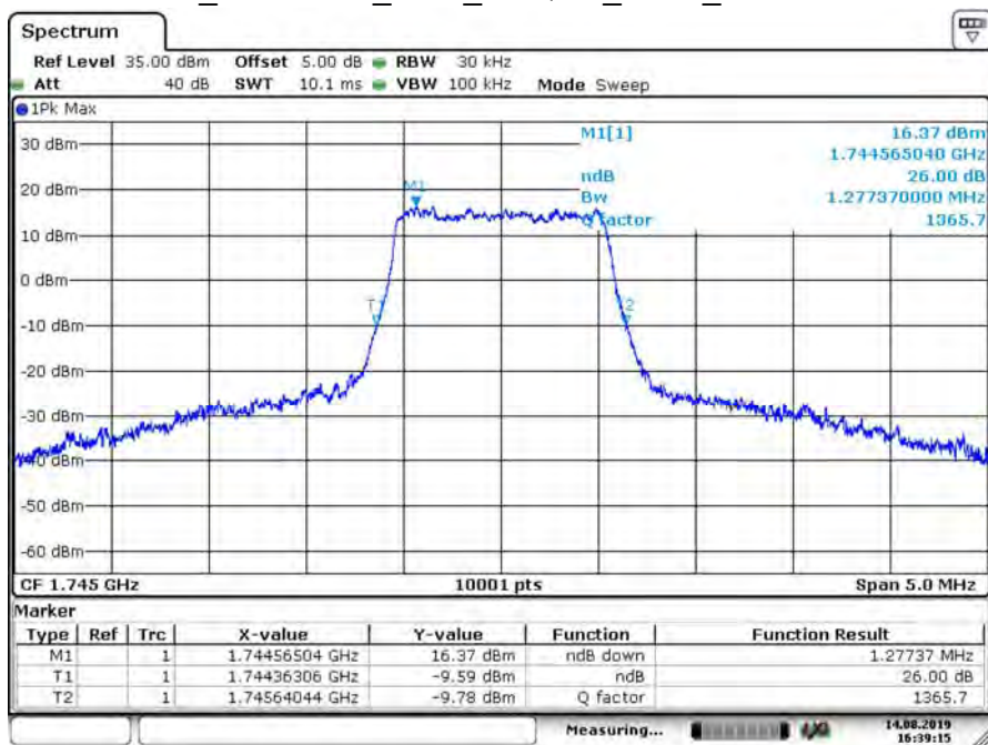
B66_CH132322_1.4M_16-QAM_6RB0_26dB BW
