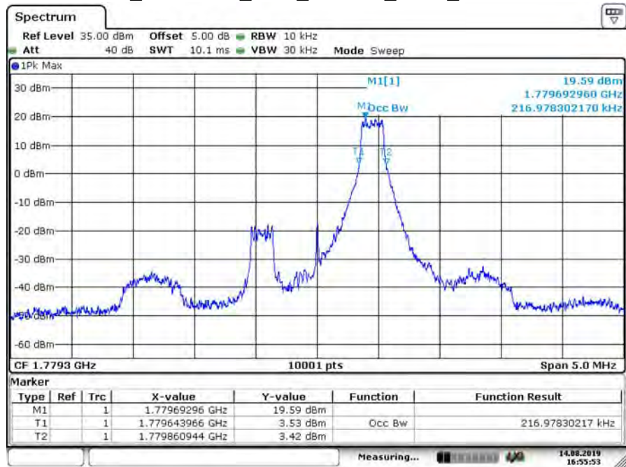
B66_CH132665_1.4M_16-QAM_1RB5_99% BW
