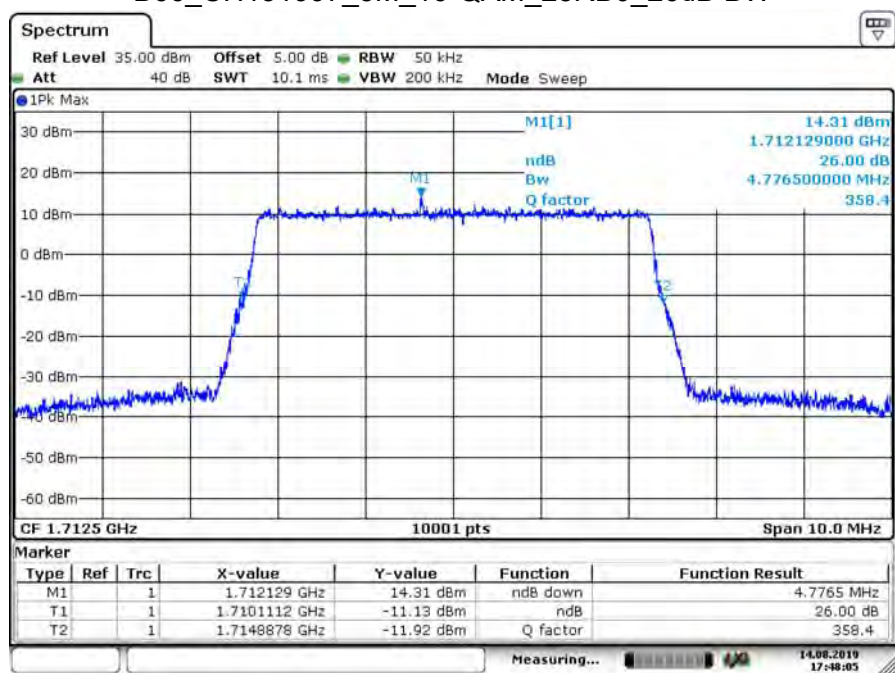
B66_CH131997_5M_16-QAM_25RB0_26dB BW
