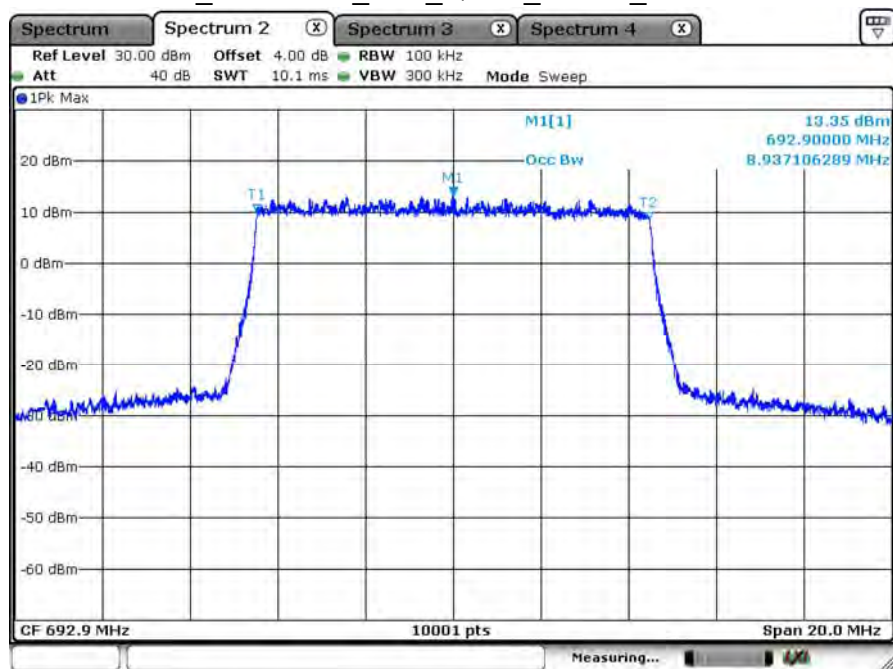
B71_CH133421_10M_QPSK_50RB0_99% BW
