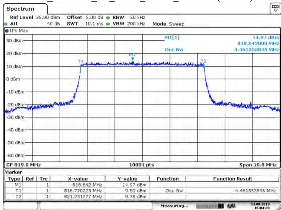
B26_CH26740_5M_QPSK_25RB0_99% BW (Part 90)
