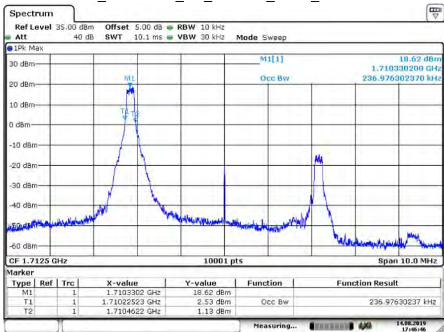
B66_CH131997_5M_16-QAM_1RB0_99% BW
