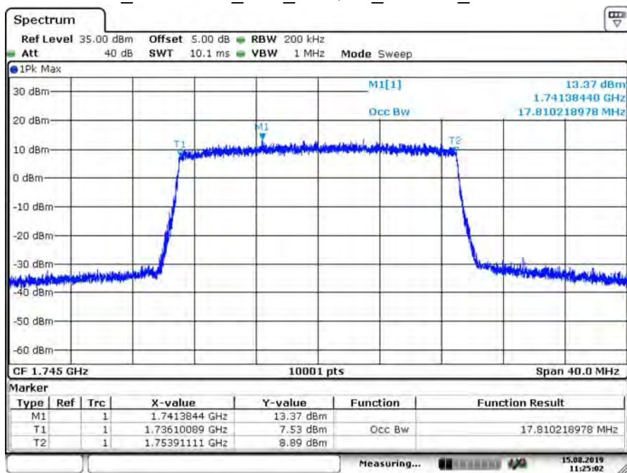
B66_CH132322_20M_16-QAM_100RB0_99% BW
