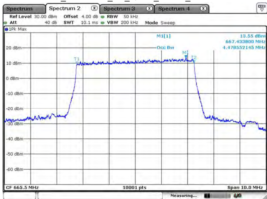
B71_CH133147_5M_QPSK_25RB0_99% BW
