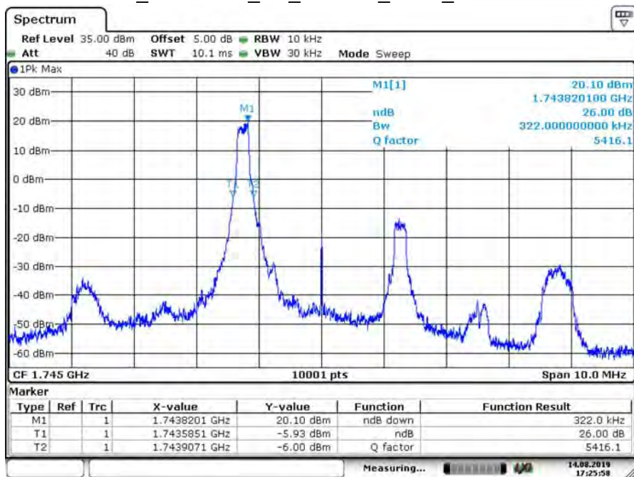
B66_CH132322_3M_16-QAM_1RB0_26dB BW
