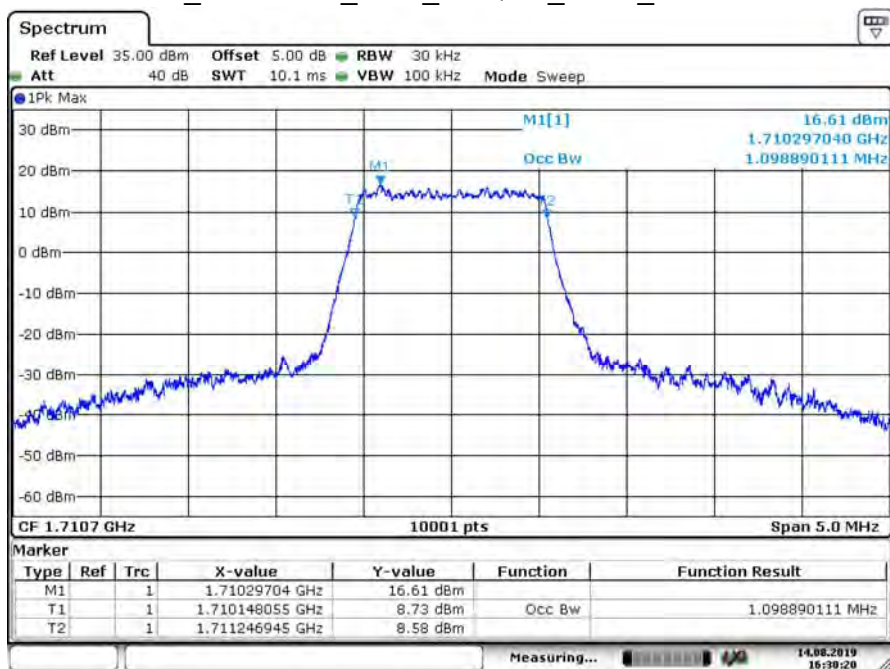
B66_CH131979_1.4M_16-QAM_6RB0_99% BW
