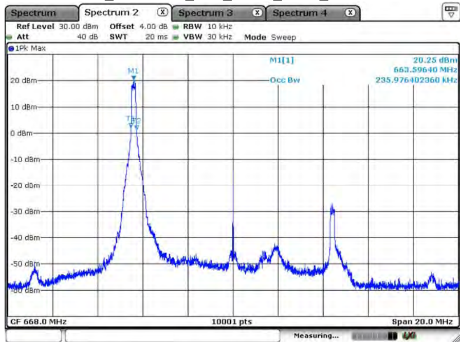
B71_CH133172_10M_QPSK_1RB0_99% BW
