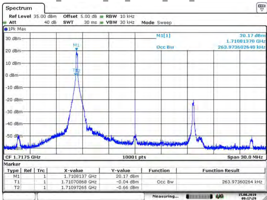
B66_CH132047_15M_16-QAM_1RB0_99% BW
