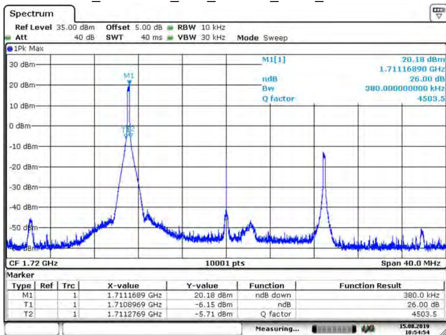
B66_CH132072_20M_16-QAM_1RB0_26dB BW
