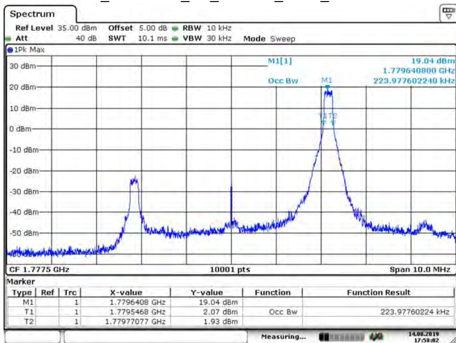
B66_CH132647_5M_16-QAM_1RB0_99% BW
