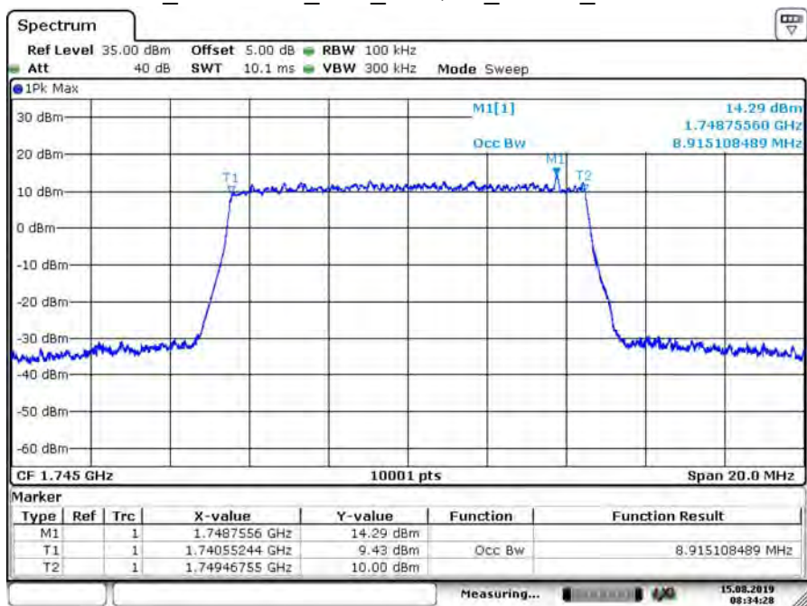
B66_CH132322_10M_16-QAM_50RB0_99% BW
