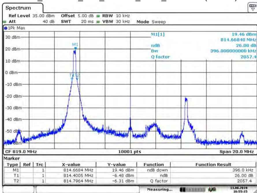
B26_CH26740_10M_16-QAM_1RB0_26dB BW (Part 90)
