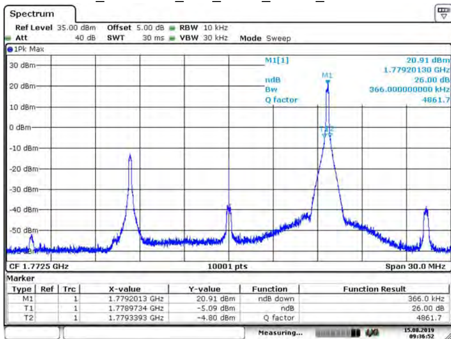
B66_CH132597_15M_QPSK_1RB74_26dB BW
