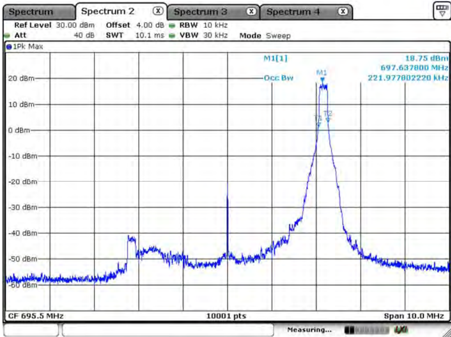
B71_CH133447_5M_16-QAM_1RB24_99% BW
