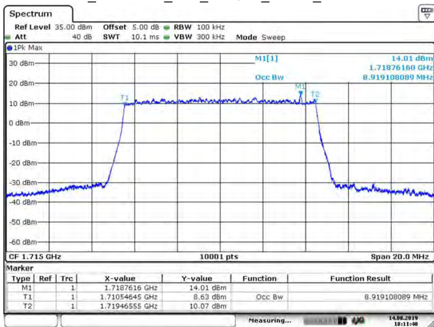
B66_CH132022_10M_16-QAM_50RB0_99% BW
