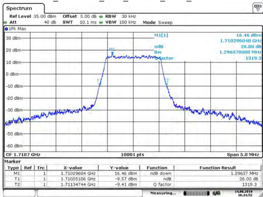
B66_CH131979_1.4M_16-QAM_6RB0_26dB BW
