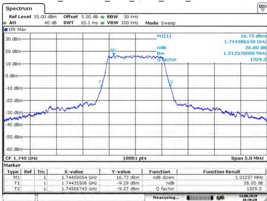
B66_CH132322_1.4M_QPSK_6RB0_26dB BW
