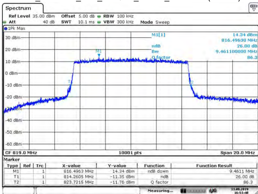
B26_CH26740_10M_16-QAM_50RB0_26dB BW (Part 90)
