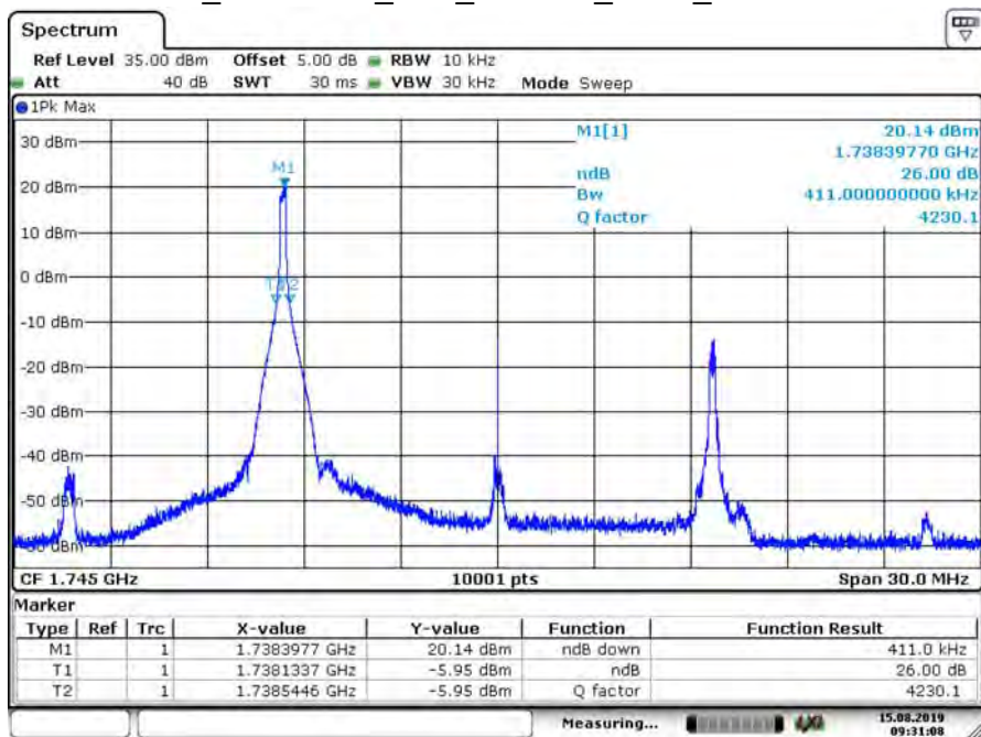
B66_CH132322_15M_16-QAM_1RB0_26dB BW
