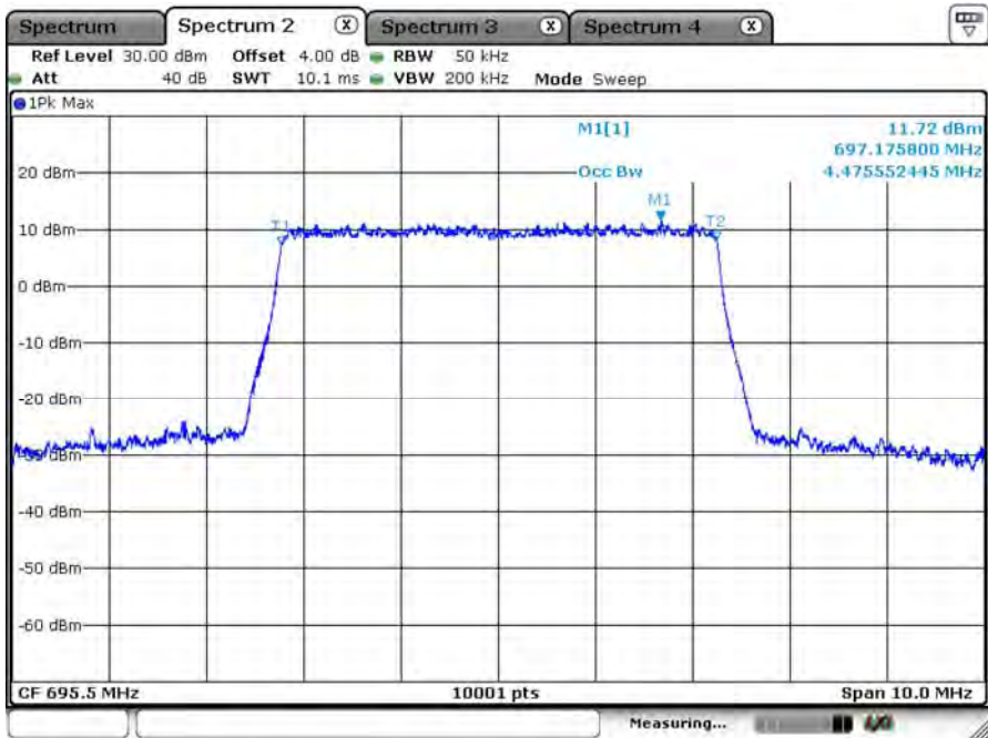
B71_CH133447_5M_16-QAM_25RB0_99% BW
