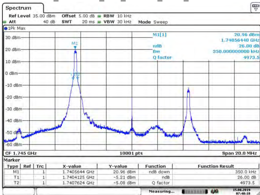
B66_CH132322_10M_16-QAM_1RB0_26dB BW
