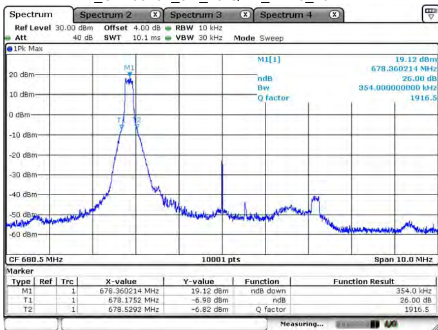
B71_CH133297_5M_16-QAM_1RB0_26dB BW
