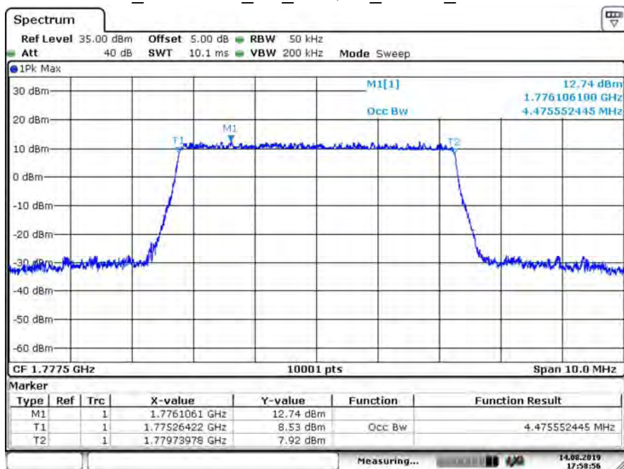
B66_CH132647_5M_16-QAM_25RB0_99% BW
