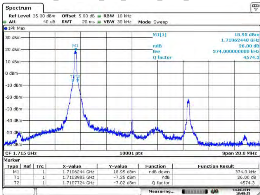
B66_CH132022_10M_16-QAM_1RB0_26dB BW
