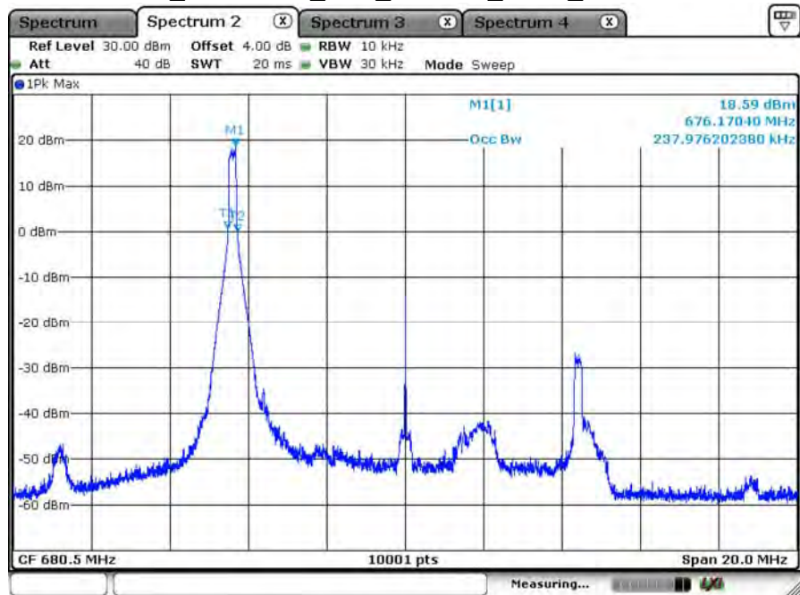
B71_CH133297_10M_16-QAM_1RB0_99% BW
