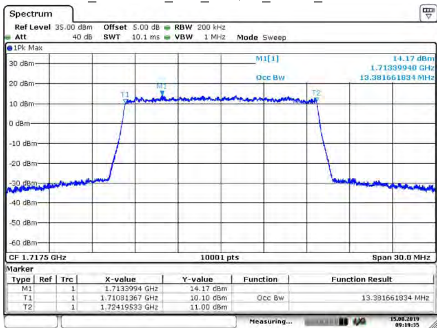
B66_CH132047_15M_16-QAM_75RB0_99% BW
