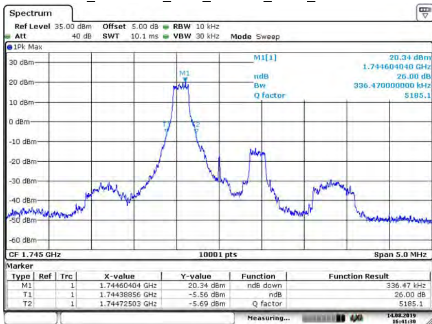
B66_CH132322_1.4M_16-QAM_1RB0_26dB BW
