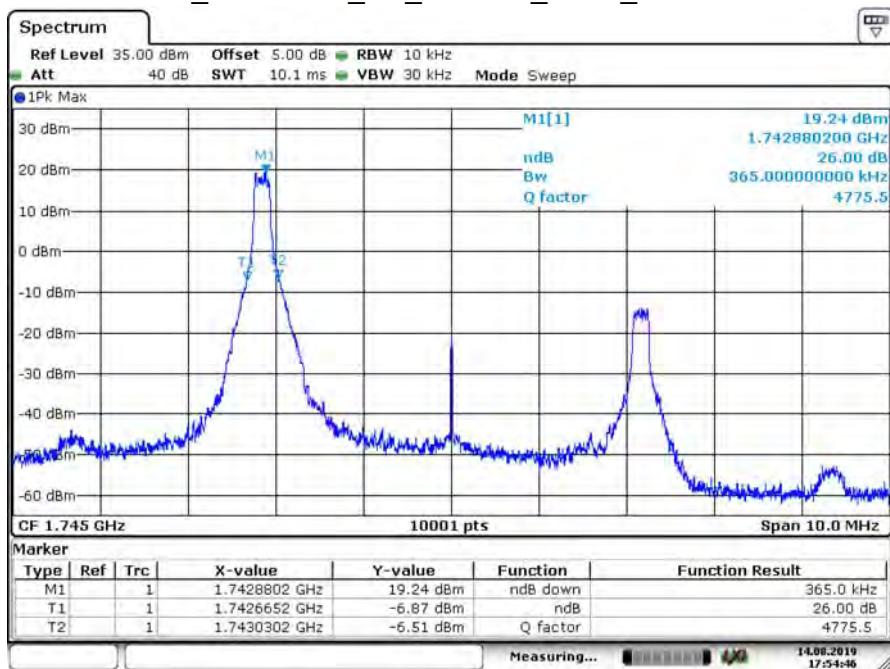
B66_CH132322_5M_16-QAM_1RB0_26dB BW
