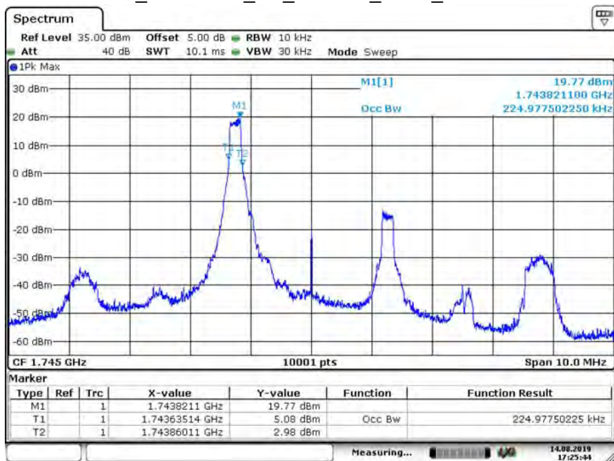
B66_CH132322_3M_16-QAM_1RB0_99% BW
