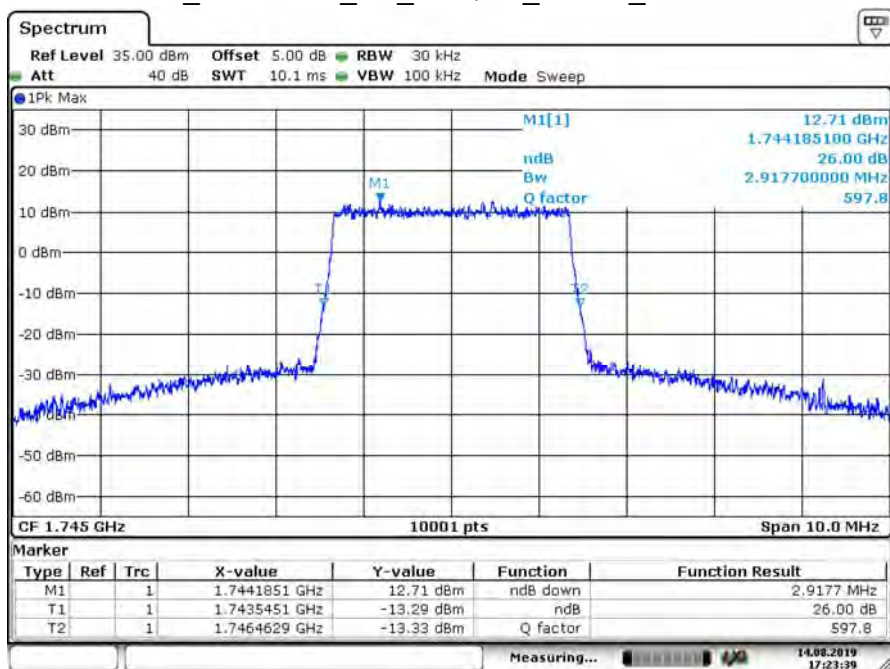
B66_CH132322_3M_16-QAM_15RB0_26dB BW
