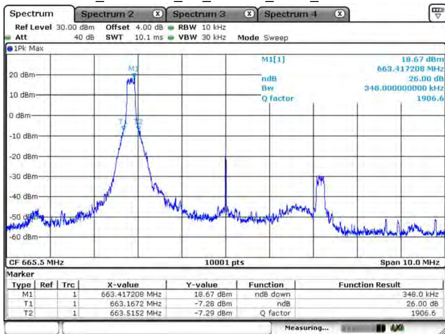
B71_CH133147_5M_16-QAM_1RB0_26dB BW
