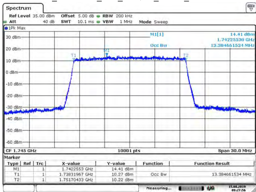
B66_CH132322_15M_16-QAM_75RB0_99% BW
