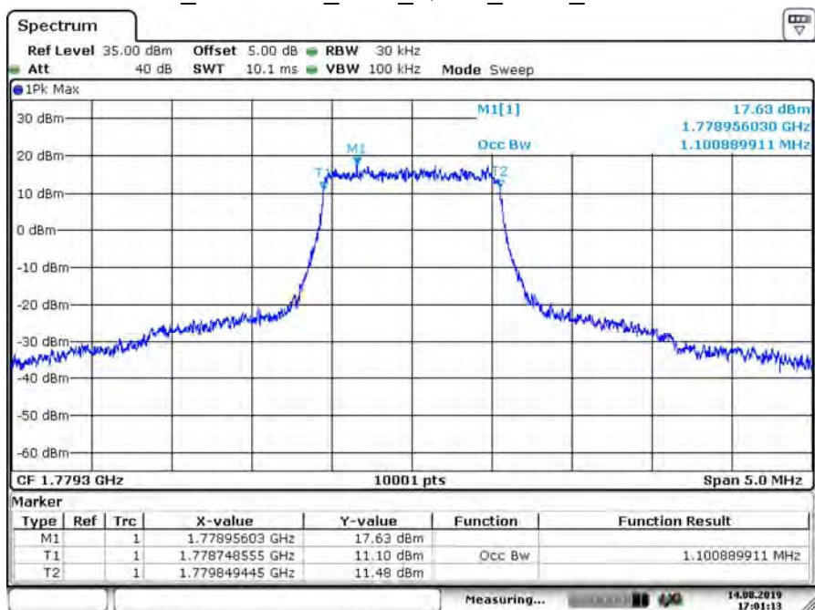
B66_CH132665_1.4M_QPSK_6RB0_99% BW
