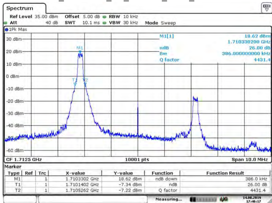
B66_CH131997_5M_16-QAM_1RB0_26dB BW
