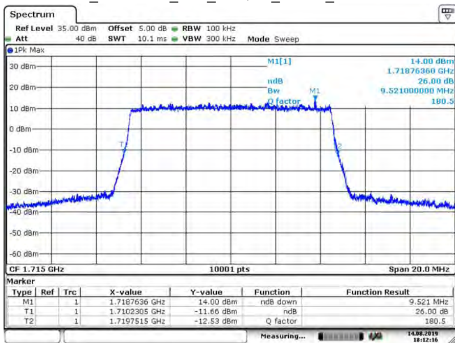
B66_CH132022_10M_16-QAM_50RB0_26dB BW
