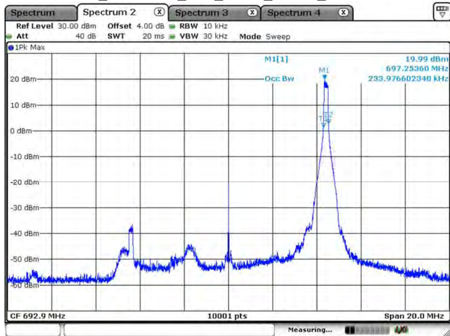
B71_CH133421_10M_QPSK_1RB49_99% BW
