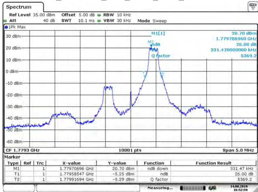
B66_CH132665_1.4M_QPSK_1RB5_26dB BW
