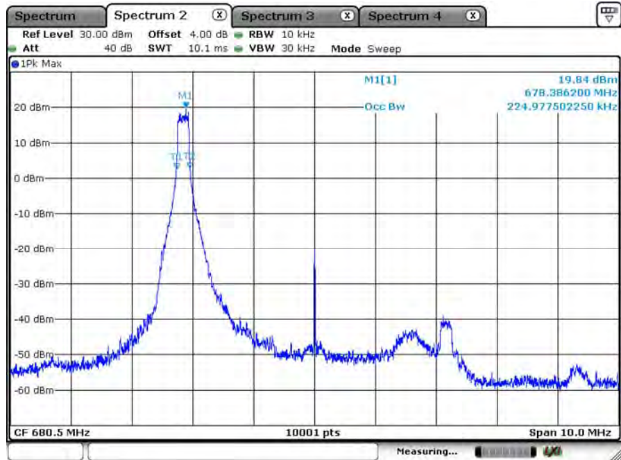
B71_CH133297_5M_QPSK_1RB0_99% BW
