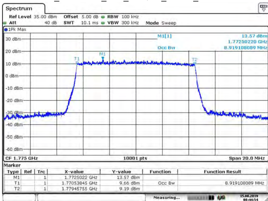
B66_CH132622_10M_16-QAM_50RB0_99% BW
