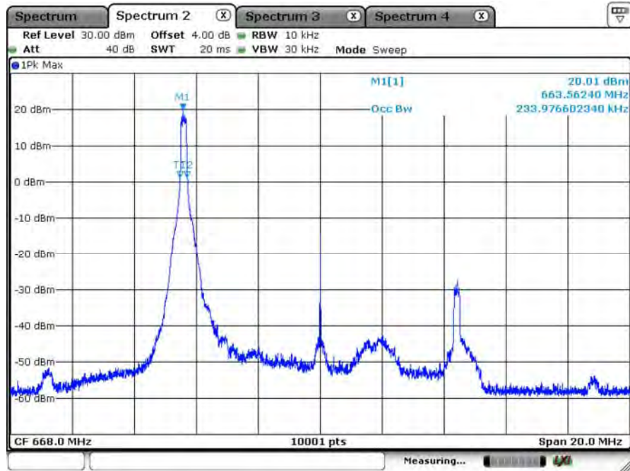
B71_CH133172_10M_16-QAM_1RB0_99% BW
