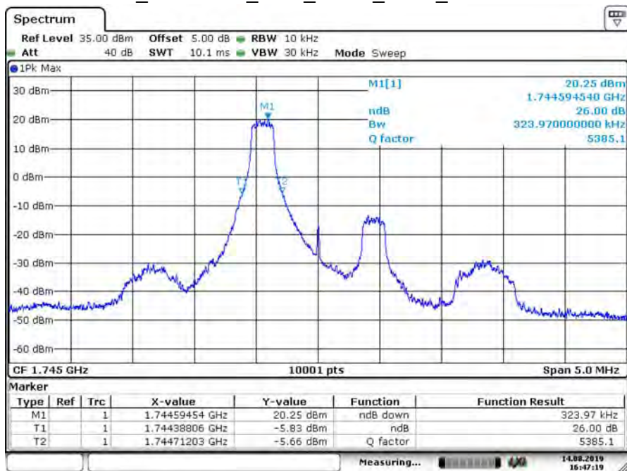
B66_CH132322_1.4M_QPSK_1RB0_26dB BW
