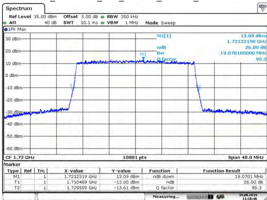
B66_CH132072_20M_16-QAM_100RB0_26dB BW
