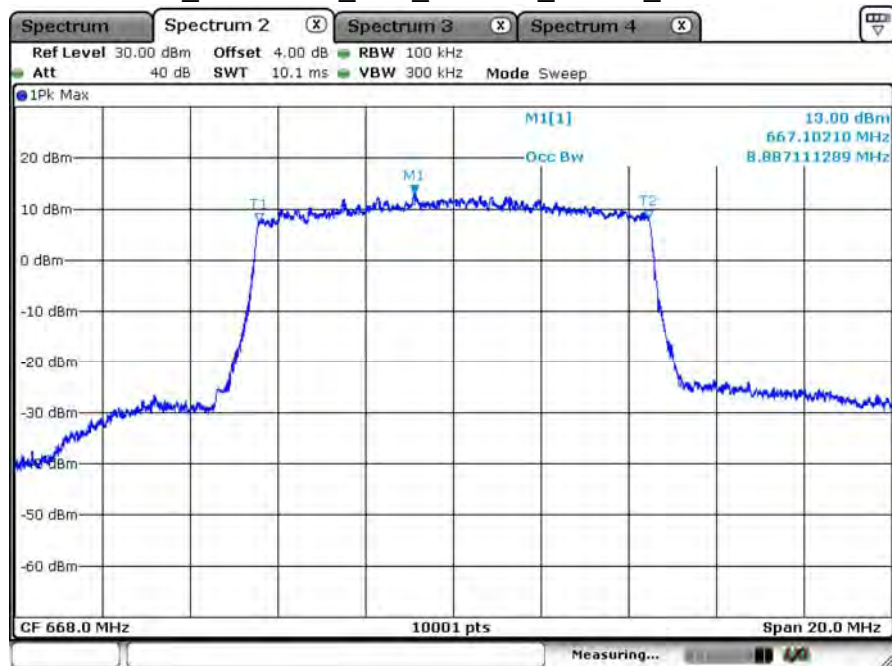
B71_CH133172_10M_16-QAM_50RB0_99% BW
