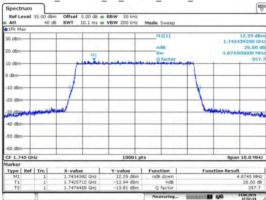
B66_CH132322_5M_16-QAM_25RB0_26dB BW
