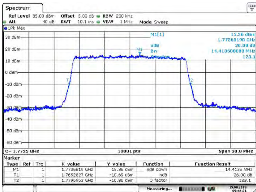
B66_CH132597_15M_QPSK_75RB0_26dB BW
