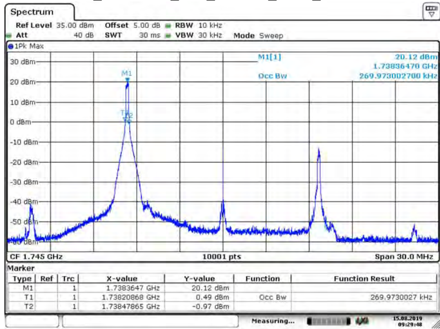
B66_CH132322_15M_16-QAM_1RB0_99% BW
