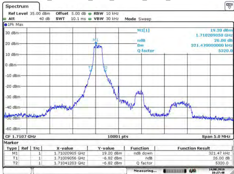
B66_CH131979_1.4M_16-QAM_1RB0_26dB BW
