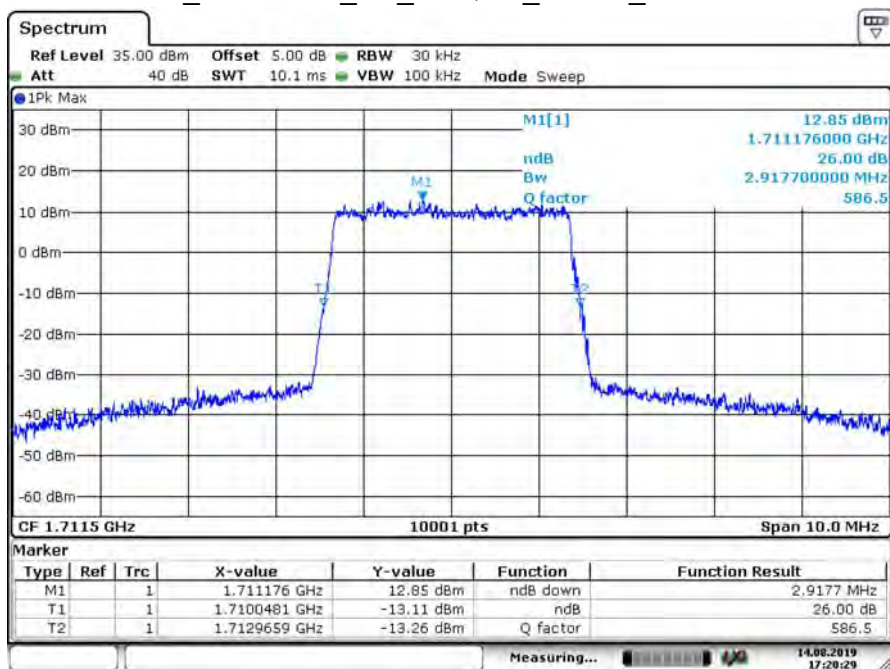
B66_CH131987_3M_16-QAM_15RB0_26dB BW
