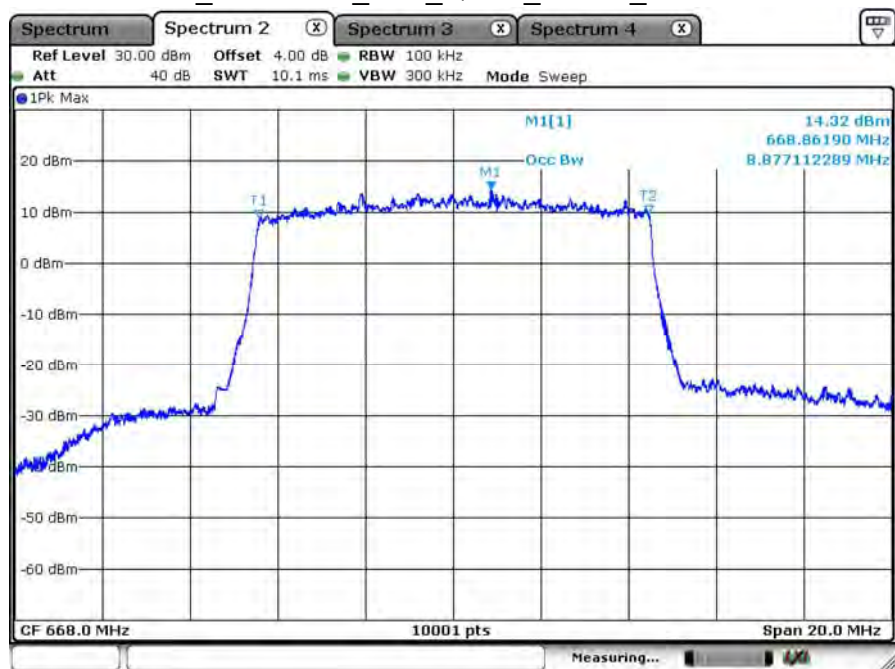
B71_CH133172_10M_QPSK_50RB0_99% BW
