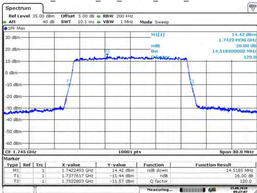
B66_CH132322_15M_16-QAM_75RB0_26dB BW
