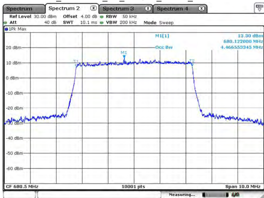
B71_CH133297_5M_16-QAM_25RB0_99% BW
