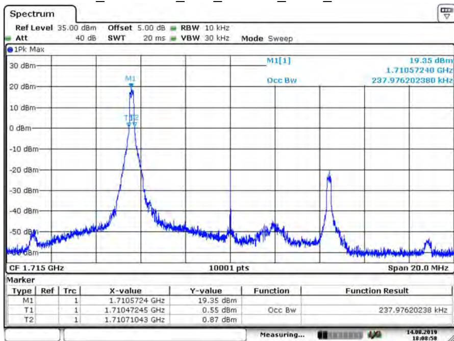
B66_CH132022_10M_16-QAM_1RB0_99% BW
