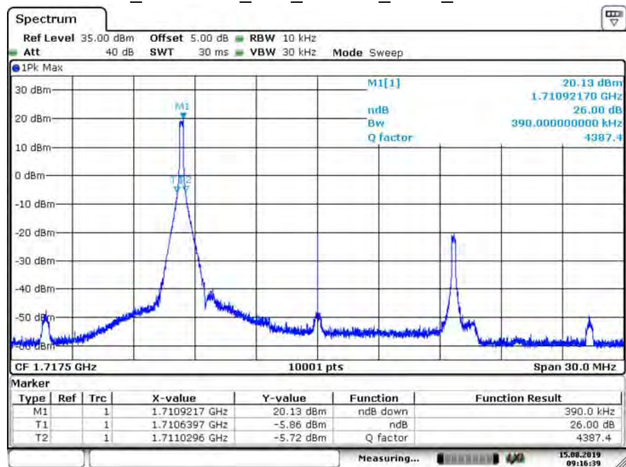
B66_CH132047_15M_16-QAM_1RB0_26dB BW
