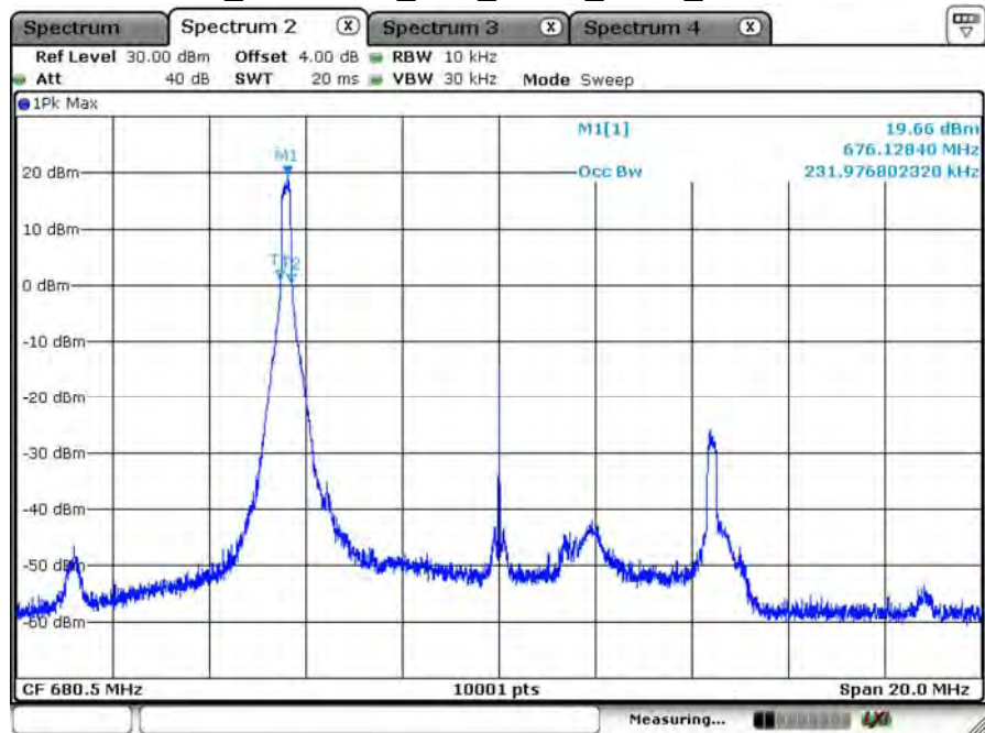
B71_CH133297_10M_QPSK_1RB0_99% BW
