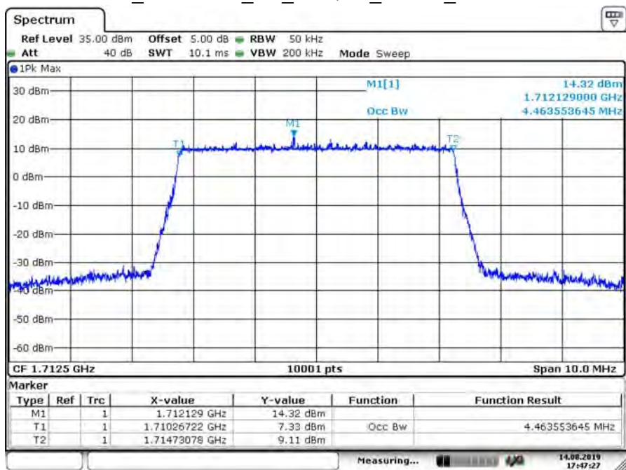
B66_CH131997_5M_16-QAM_25RB0_99% BW
