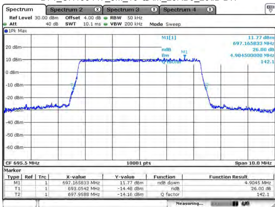
B71_CH133447_5M_16-QAM_25RB0_26dB BW
