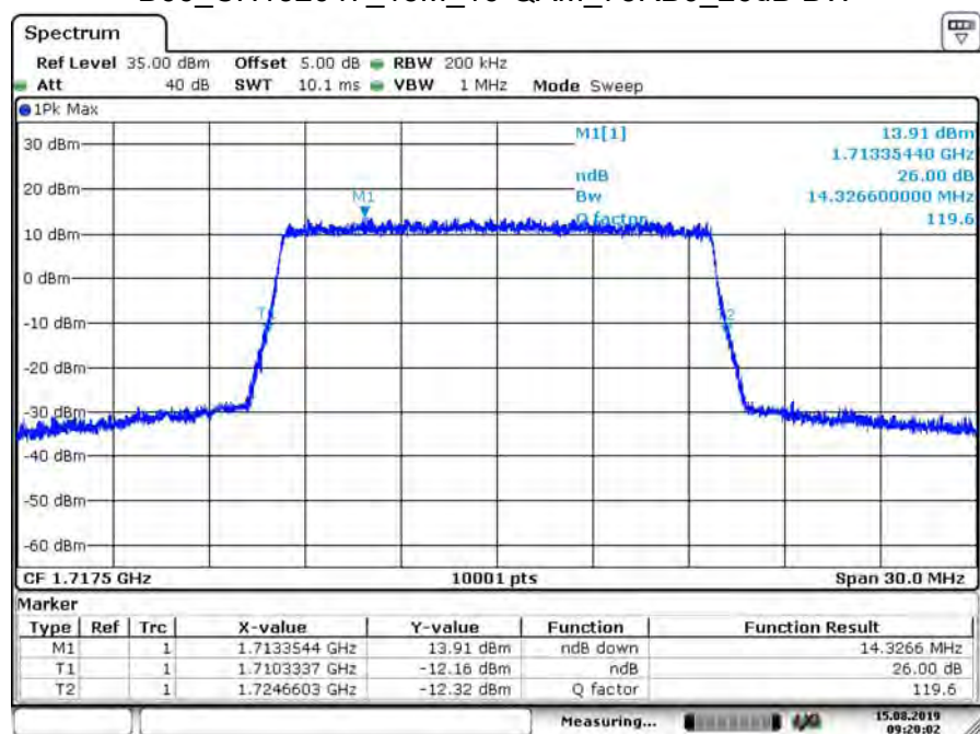
B66_CH132047_15M_16-QAM_75RB0_26dB BW
