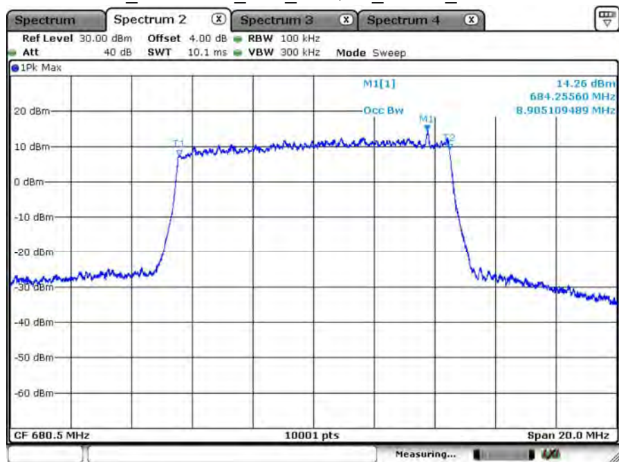
B71_CH133297_10M_16-QAM_50RB0_99% BW
