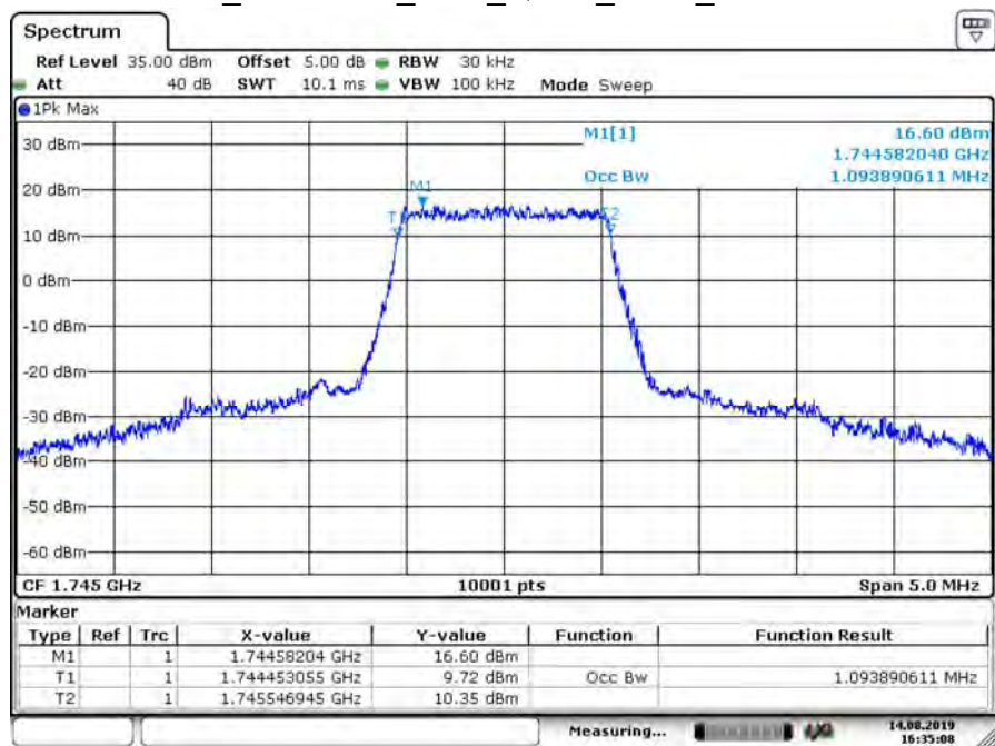
B66_CH132322_1.4M_QPSK_6RB0_99% BW
