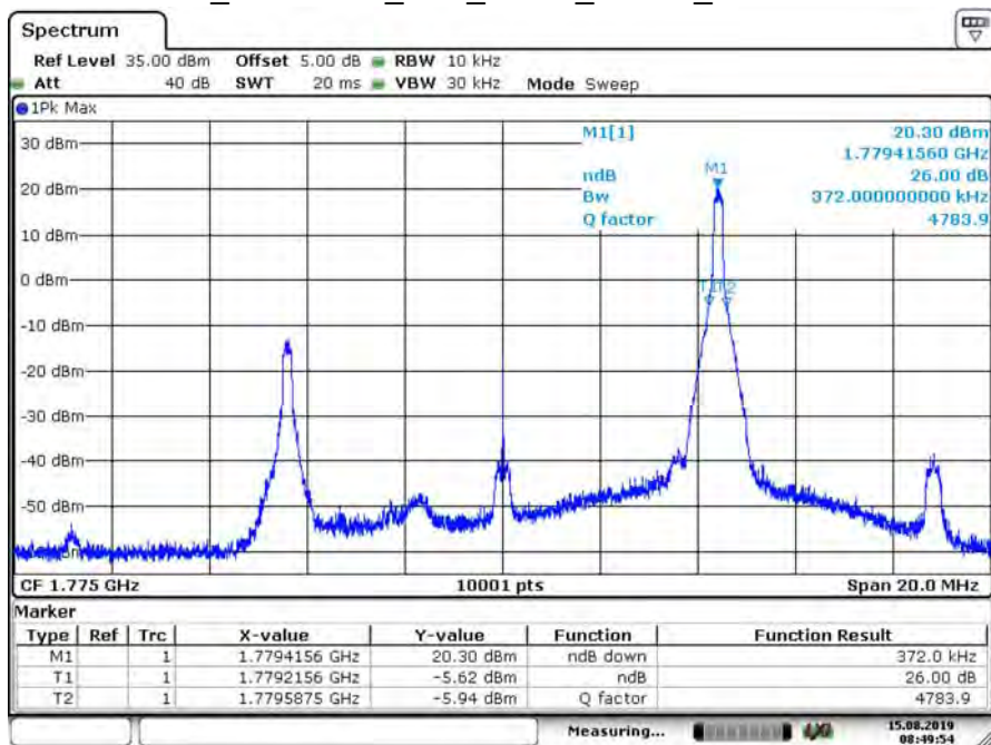
B66_CH132622_10M_QPSK_1RB49_26dB BW
