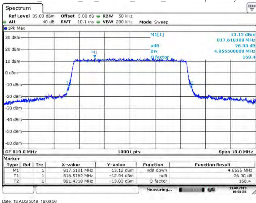
B26_CH26740_5M_16-QAM_25RB0_26dB BW (Part 90)
