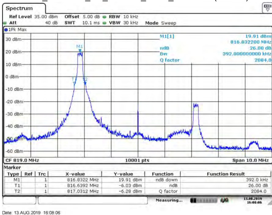
B26_CH26740_5M_16-QAM_1RB0_26dB BW (Part 90)
