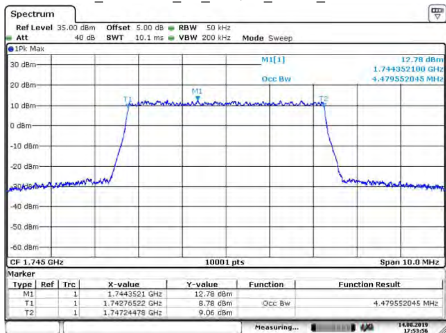
B66_CH132322_5M_16-QAM_25RB0_99% BW
