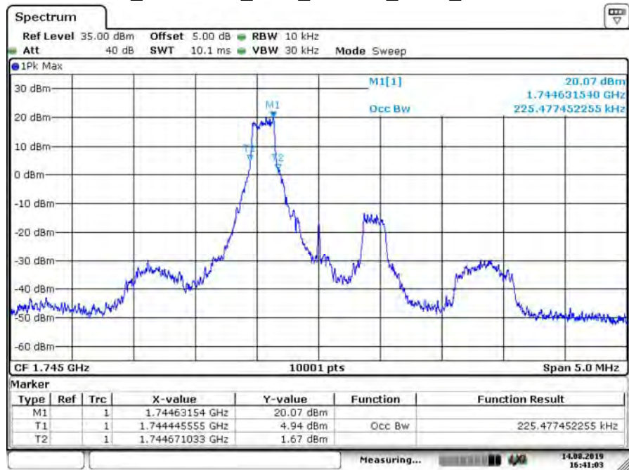
B66_CH132322_1.4M_16-QAM_1RB0_99% BW
