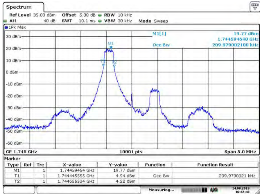
B66_CH132322_1.4M_QPSK_1RB0_99% BW
