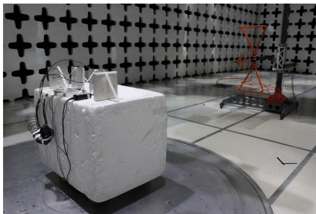
FCC RSE 30MHz to 1GHz – Rear View
