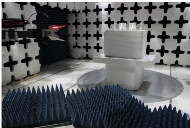
FCC RSE 1GHz to 18GHz – Front View
