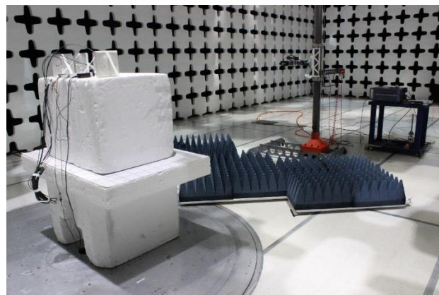
FCC RSE 18GHz to 40GHz – Rear View
