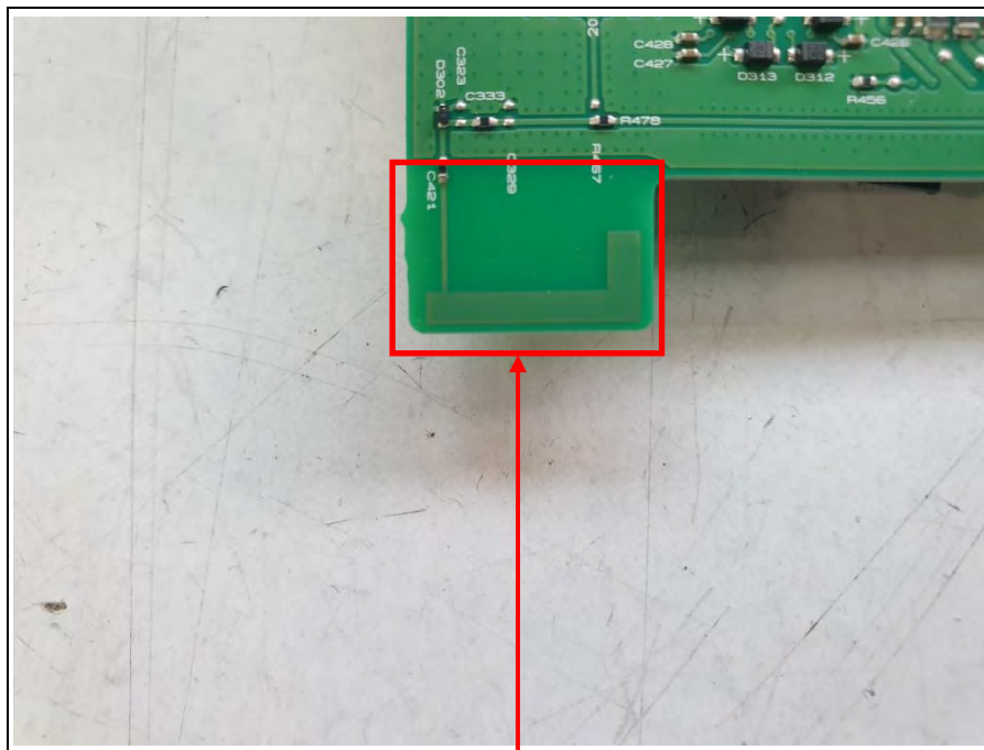
BT Antenna
