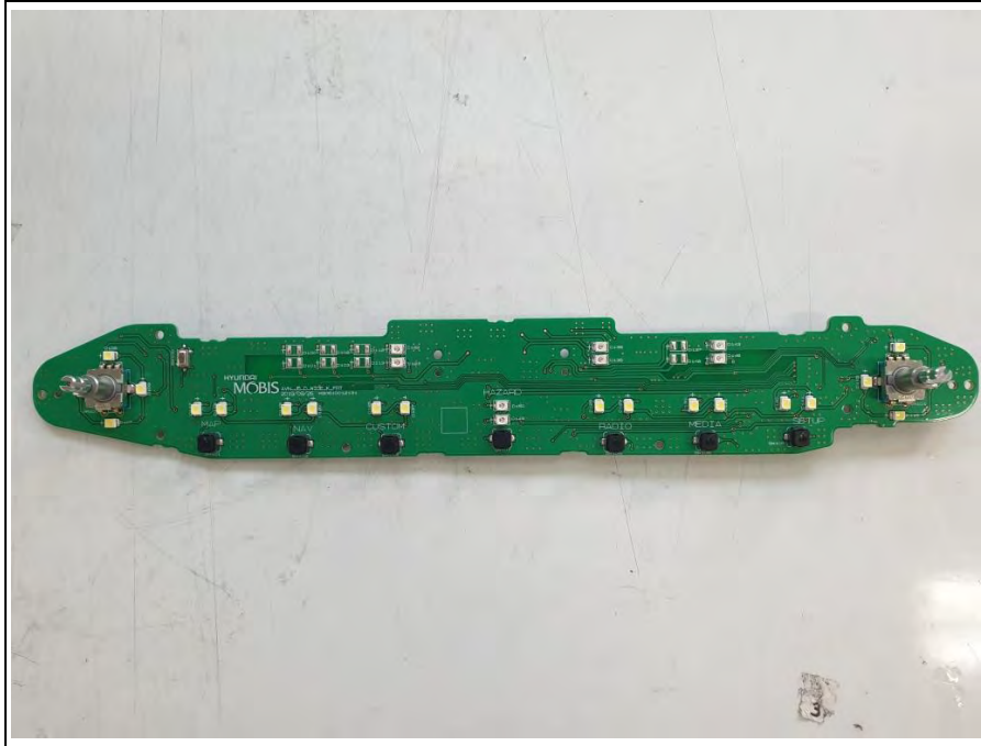
Bottom view of Sub PCB2
