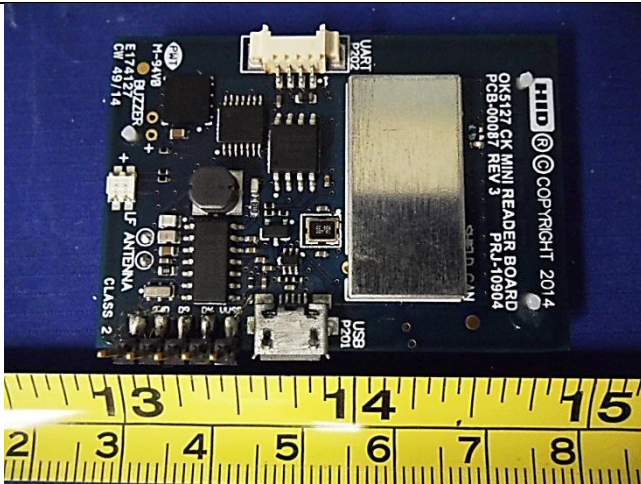
PCBA View 1
