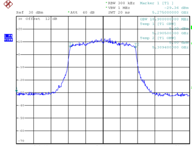
99 % Occupied Bandwidth
