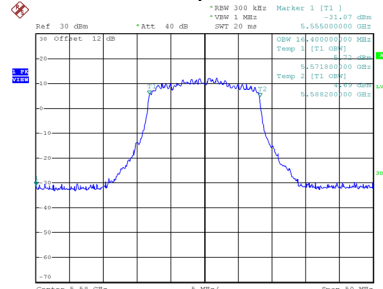
99 % Occupied Bandwidth
