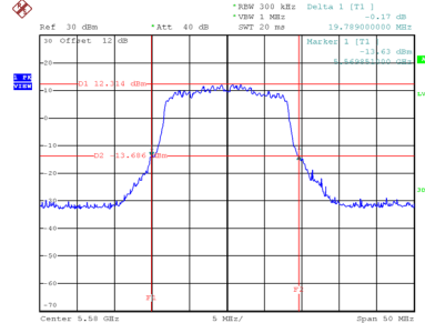
CH116 26 dB Bandwidth
