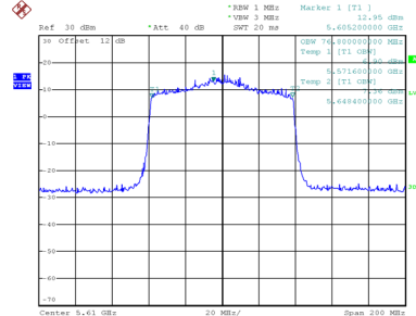
99 % Occupied Bandwidth
