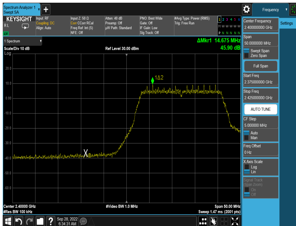
Plot 7-44. Band Edge Plot (802.11n MCS0 – Ch. 1)
