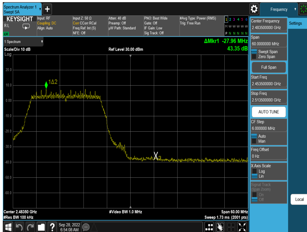
Plot 7-54. Band Edge Plot (802.11n MCS0 – Ch. 12)
