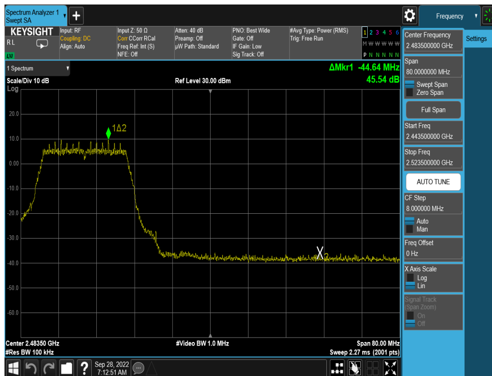
Plot 7-52. Band Edge Plot (802.11n MCS0 – Ch. 10)
