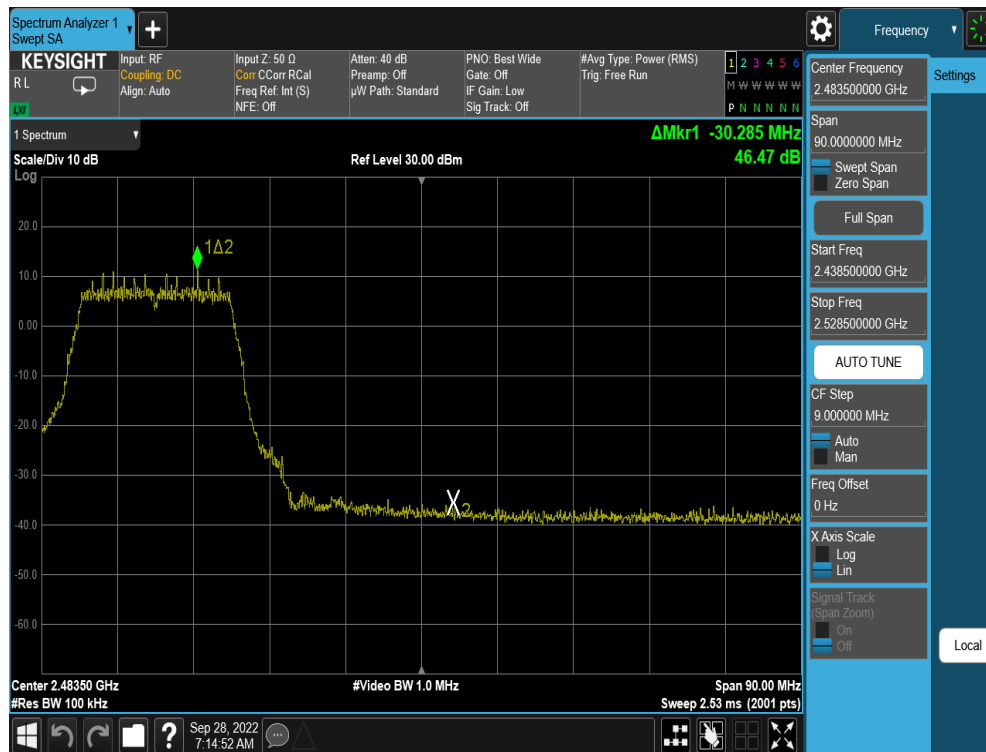
Plot 7-51. Band Edge Plot (802.11n MCS0 – Ch. 9)
