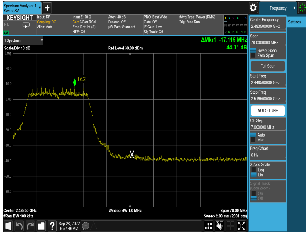
Plot 7-53. Band Edge Plot (802.11n MCS0– Ch. 11)
