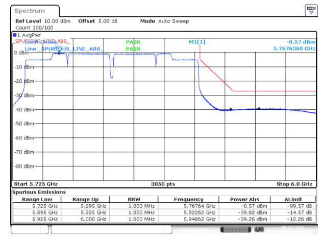
BE-NR-HIGH, MIMO-B, 802.11ac160-VHT0, Ch163
