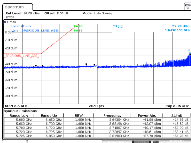
BE-NR-LOW, MIMO-B, 802.11n20-HT0, Ch177
