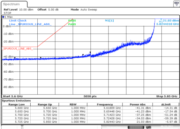
BE-NR-LOW, MIMO-B, 802.11ax40-MCS0, Ch167
