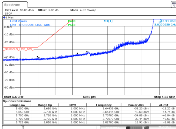
BE-NR-LOW, MIMO-A, 802.11n40-HT0, Ch167
