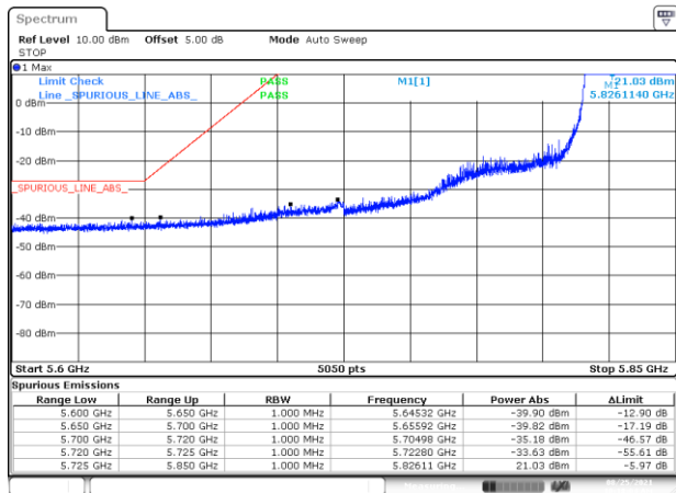
BE-NR-LOW, MIMO-A, 802.11ax40-MCS0, Ch167
