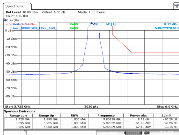
BE-NR-HIGH, MIMO-B, 802.11n20-HT0, Ch173
