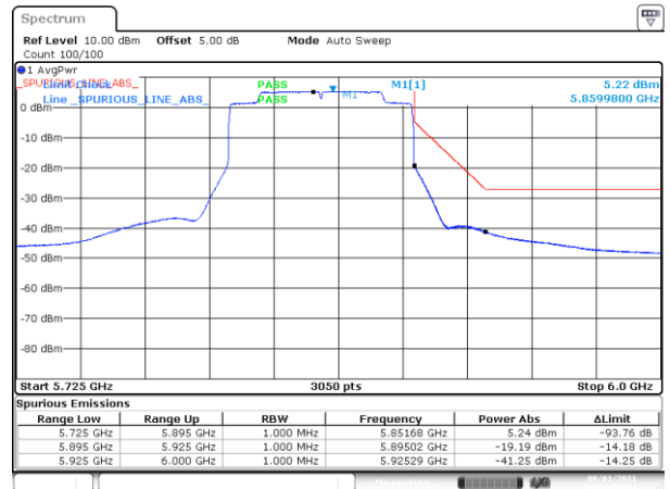
BE-NR-HIGH, MIMO-A, 802.11ax80-MCS0, Ch171
