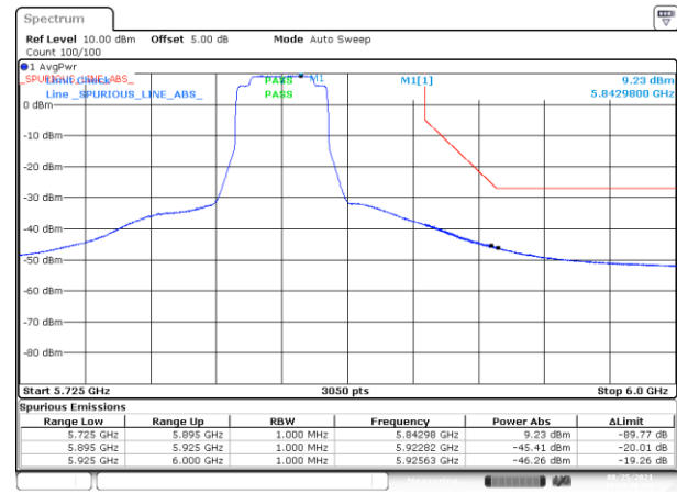
BE-NR-HIGH, MIMO-A, 802.11ax40-MCS0, Ch167
