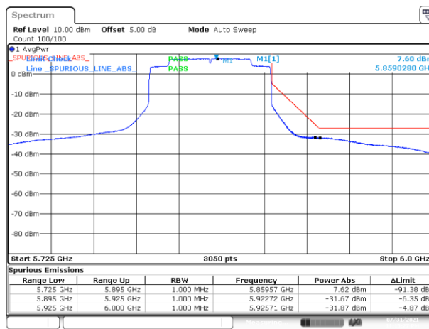
BE-NR-HIGH, SISO-A, 802.11ax80-MCS0, Ch171
