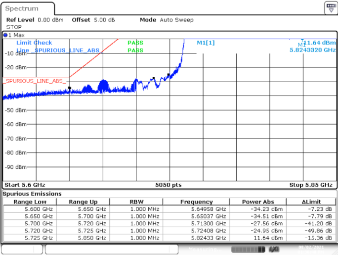
BE-NR-LOW, MIMO-B, 802.11ax160-MCS0, Ch163
