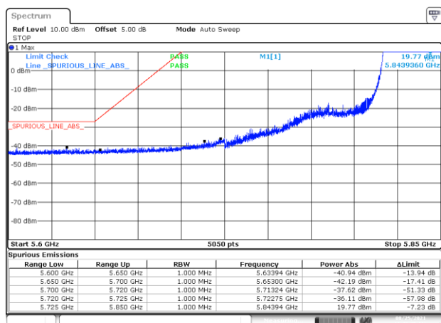
BE-NR-LOW, MIMO-B, 802.11n40-HT0, Ch167
