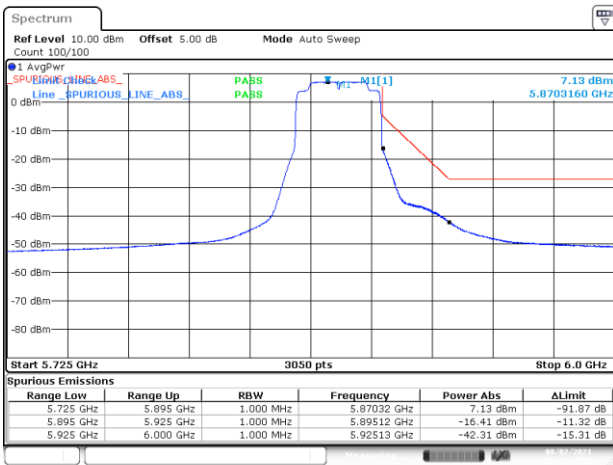
BE-NR-HIGH, MIMO-B, 802.11ax40-MCS0, Ch175
