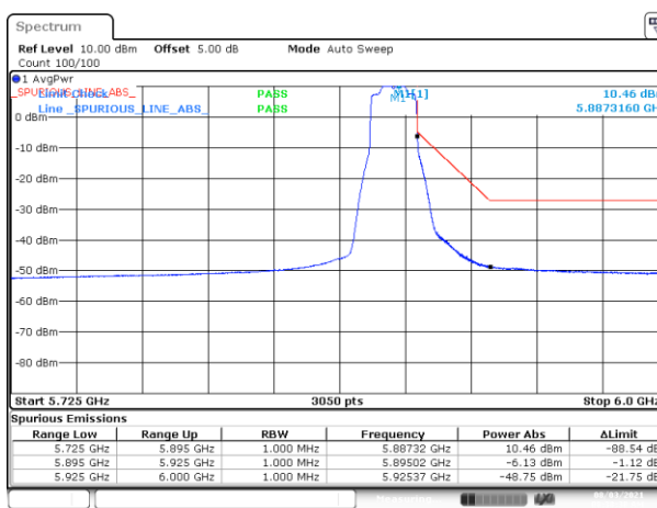
BE-NR-HIGH, SISO-B, 802.11ax20-MCS0, Ch177
