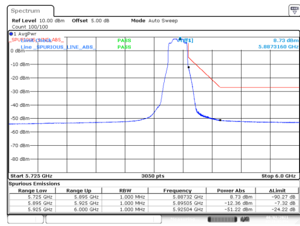
BE-NR-HIGH, MIMO-B, 802.11n20-HT0, Ch177
