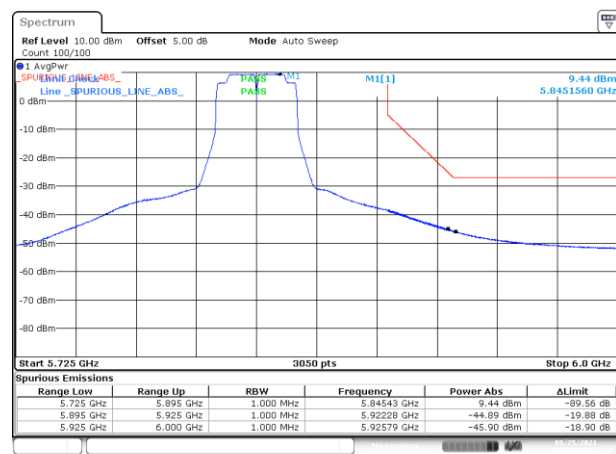
BE-NR-HIGH, MIMO-B, 802.11n40-HT0, Ch167
