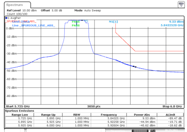
BE-NR-HIGH, MIMO-A, 802.11n40-HT0, Ch167
