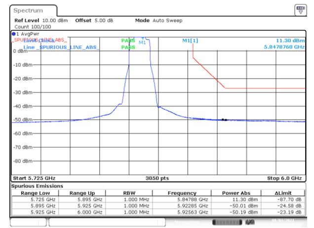
BE-NR-HIGH, SISO-B, 802.11ax20-MCS0, Ch169
