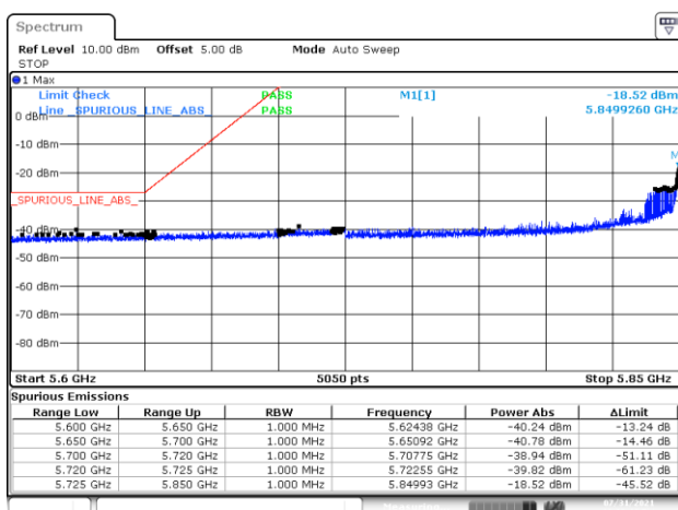
BE-NR-LOW, SISO-A, 802.11ax20-MCS0, Ch173
