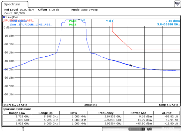
BE-NR-HIGH, MIMO-B, 802.11ax40-MCS0, Ch167
