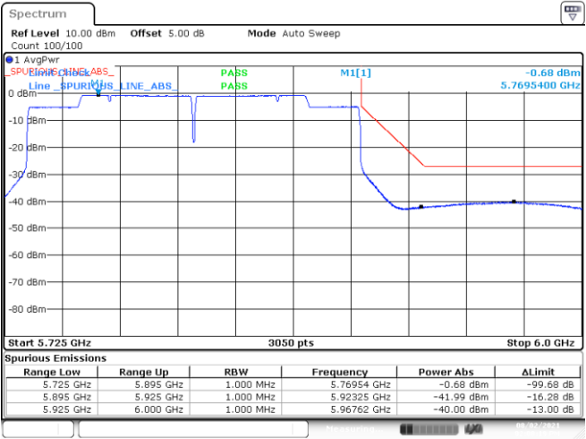
BE-NR-HIGH, MIMO-B, 802.11ax160-MCS0, Ch163
